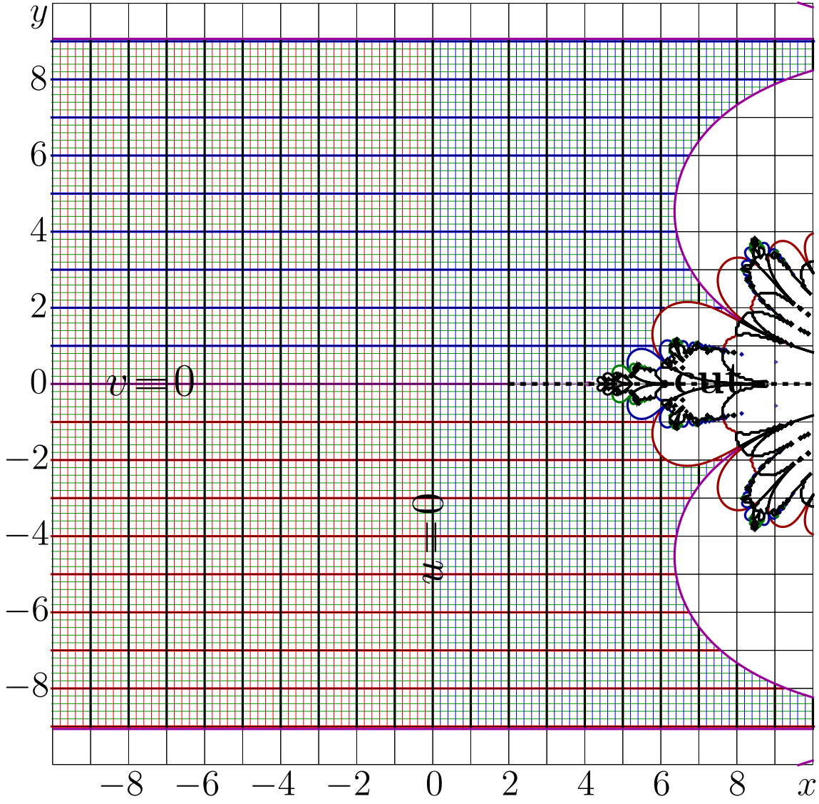
Figure 16.4: u+iv = \text{tet}_{\sqrt{2}}(\text{ate}_{\sqrt{2}}(x+iy))
