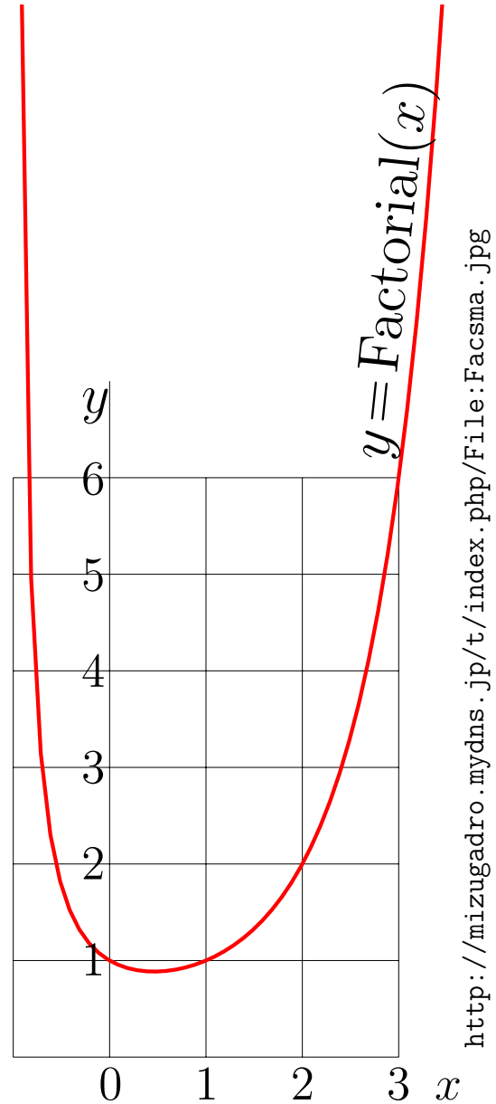
Figure 8.1: y = \text{Factorial}(x)
