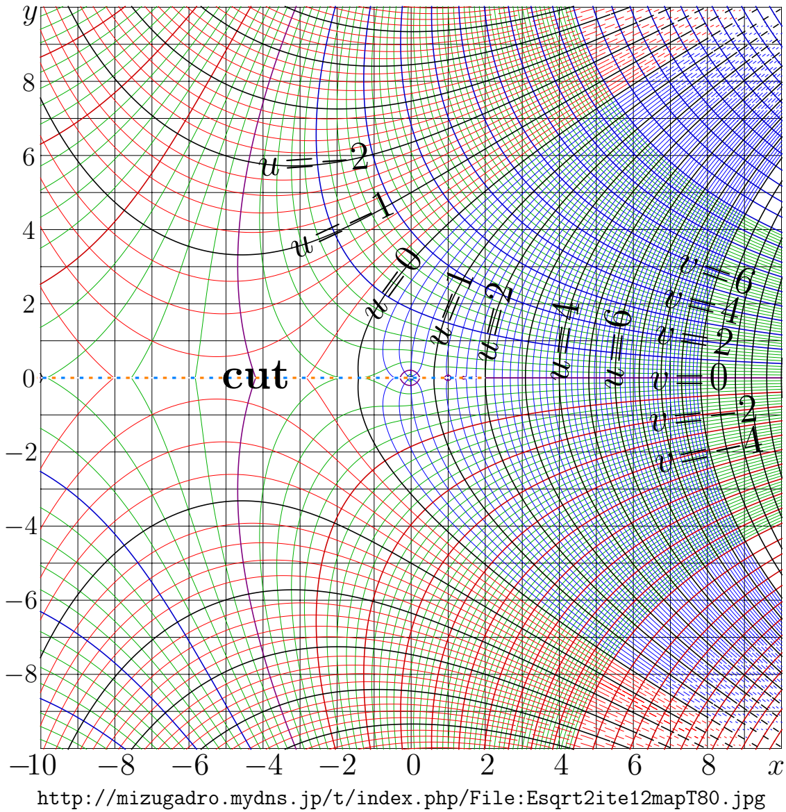
Figure 9.9: u+iv = T^{1/2}(x+iy) by formula (9.24).
