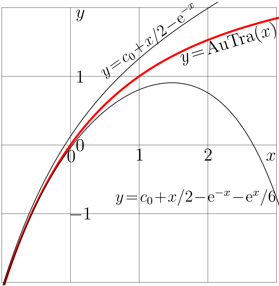
Figure 20.9: y = \text{AuTra}(x) by (20.47) and two its asymptotics by (20.44)
