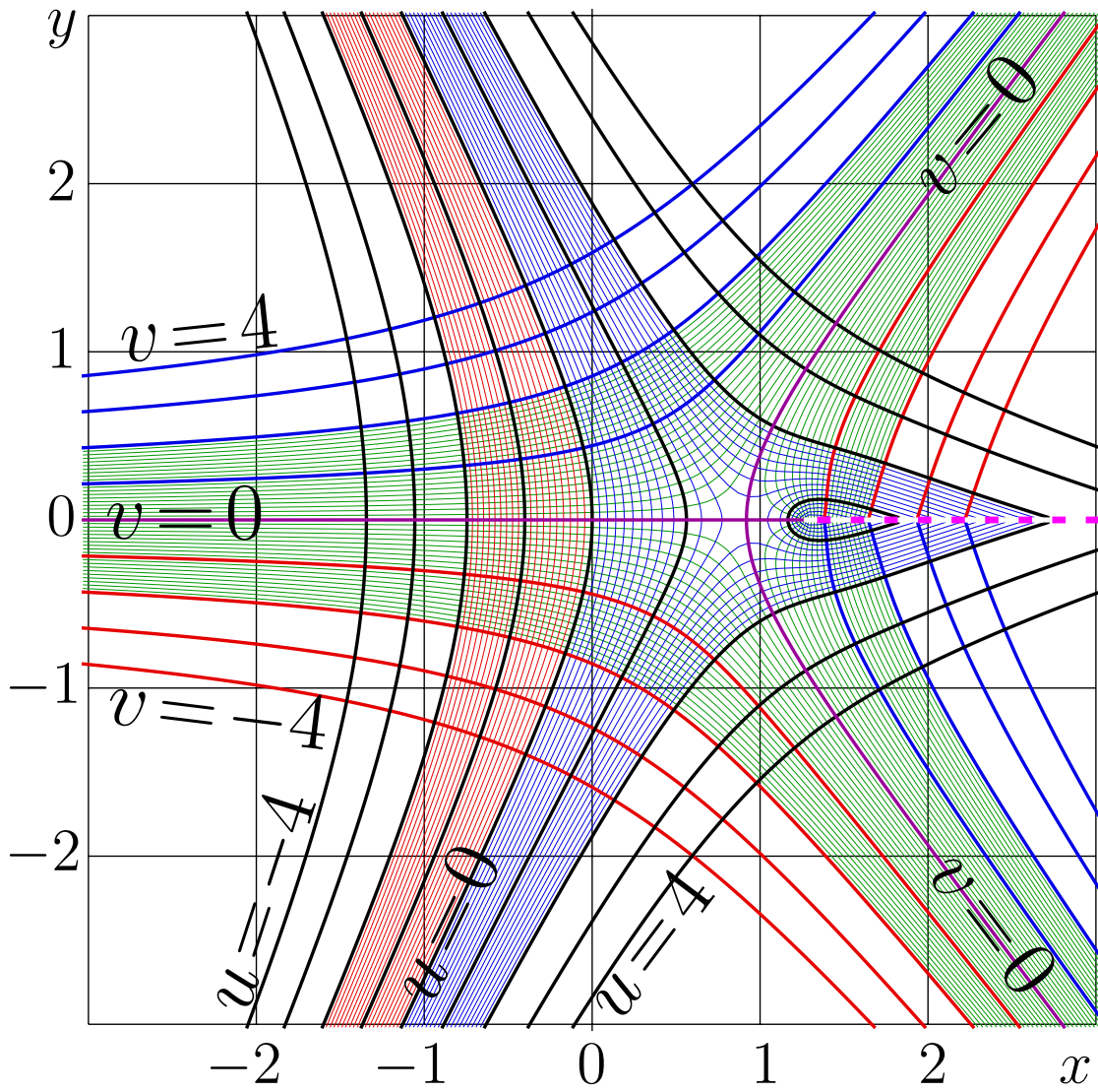
Figure 7.12: u+iv = \text{Elu}_5^{0.5}(x+iy)
