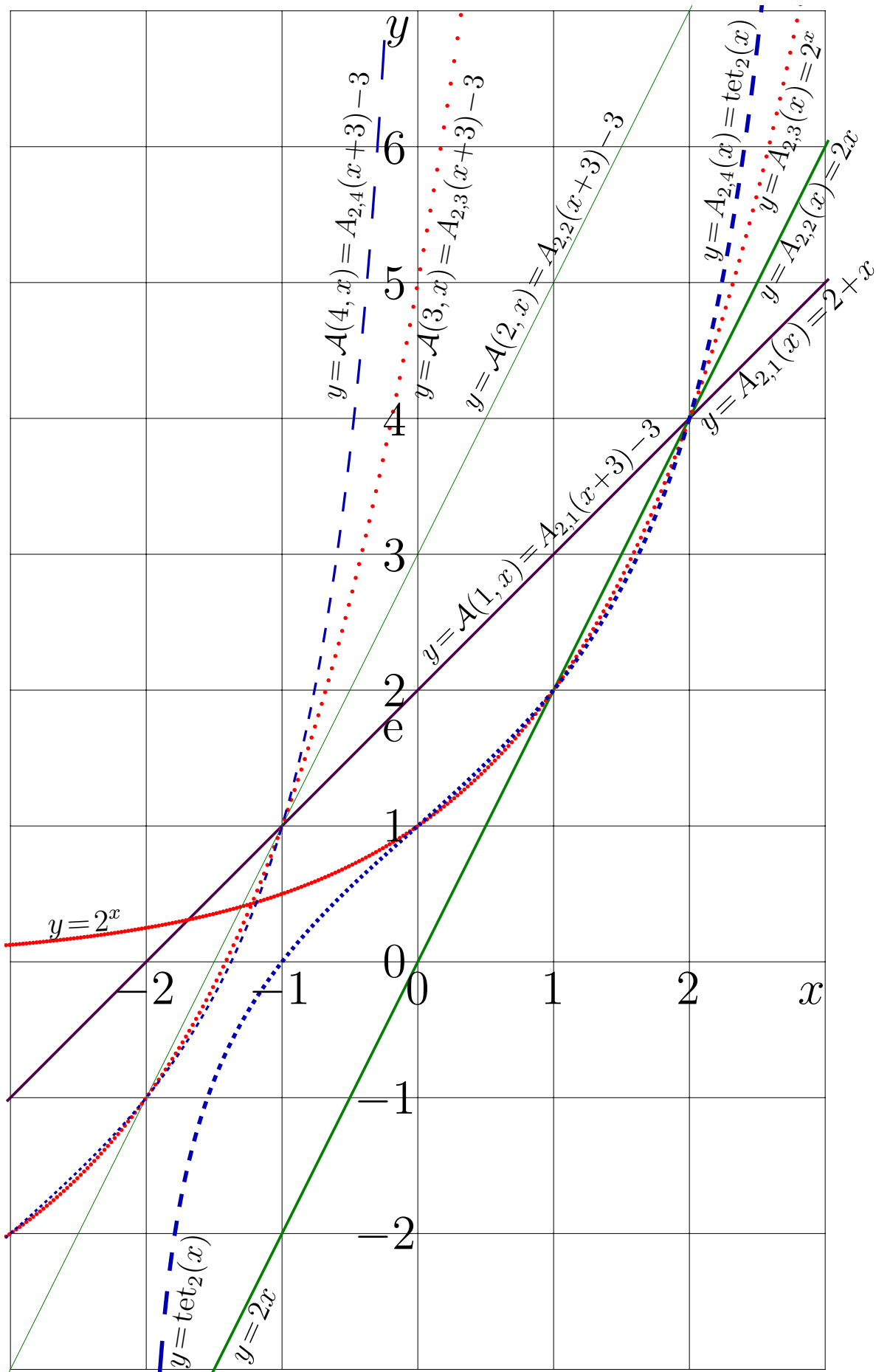
Figure 19.2: Comparison of definitions for binary ackermanns
