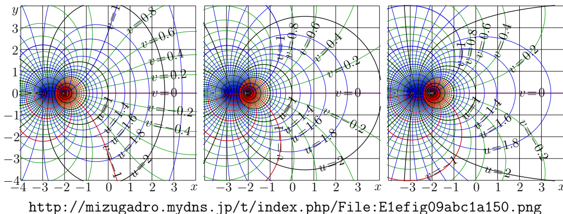
Figure 17.4: u+iv = \text{tet}_b(x+iy) for b=1.5 , b=\exp(1/e) and b=\sqrt{2}
