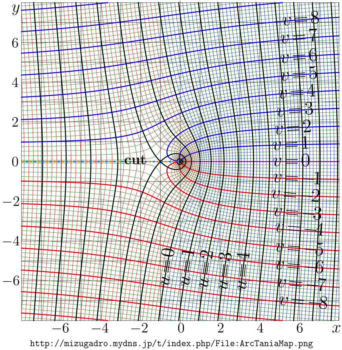
Figure 5.3: u+iv = \text{ArcTania}(x+iy)
