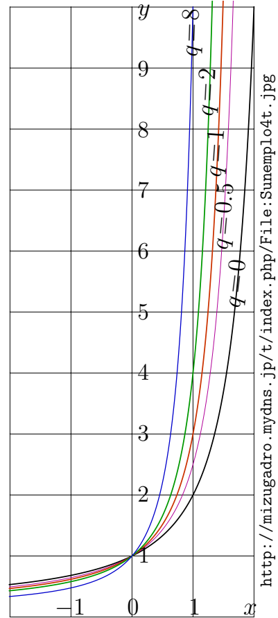
Figure 13.5: y = \text{SuNem}_q(x)
