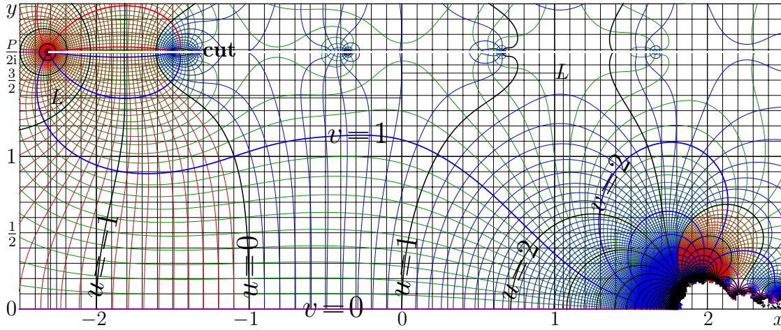
Figure 19.6: u+iv = \text{pen}(x+iy) by (19.24), zoom-in from figure 19.5
