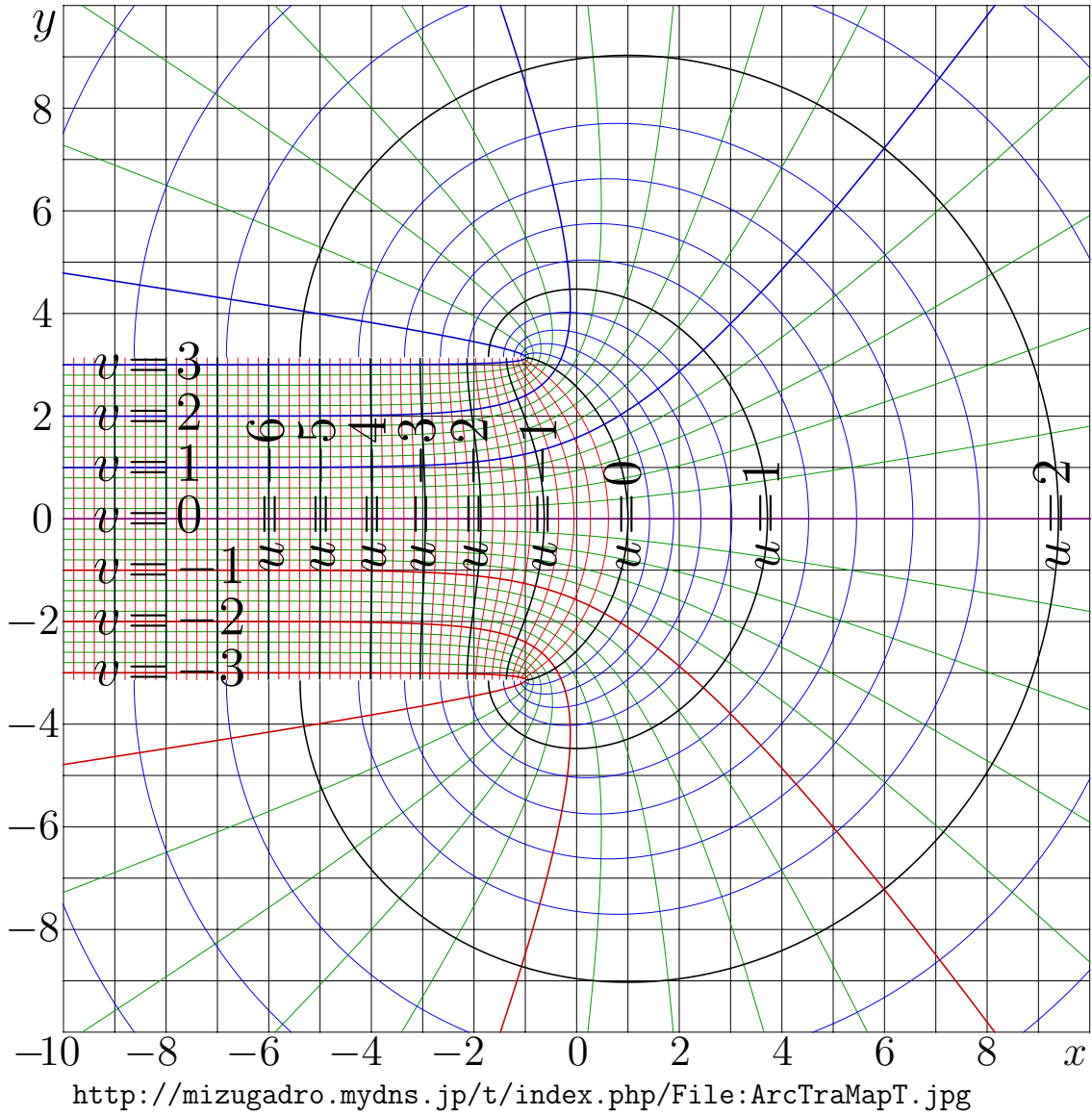
Figure 20.3: u+iv = \text{ArcTra}(x+iy)
