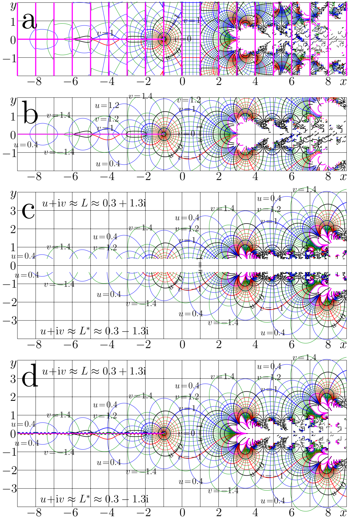
Figure 14.4: \exp(u+iv) = f(x+iy) for the following functions: f = \exp , (a); f = \text{Fit}_3 , (b); f = \text{Fit}_6 , (c); f = \text{tet} , (d)
