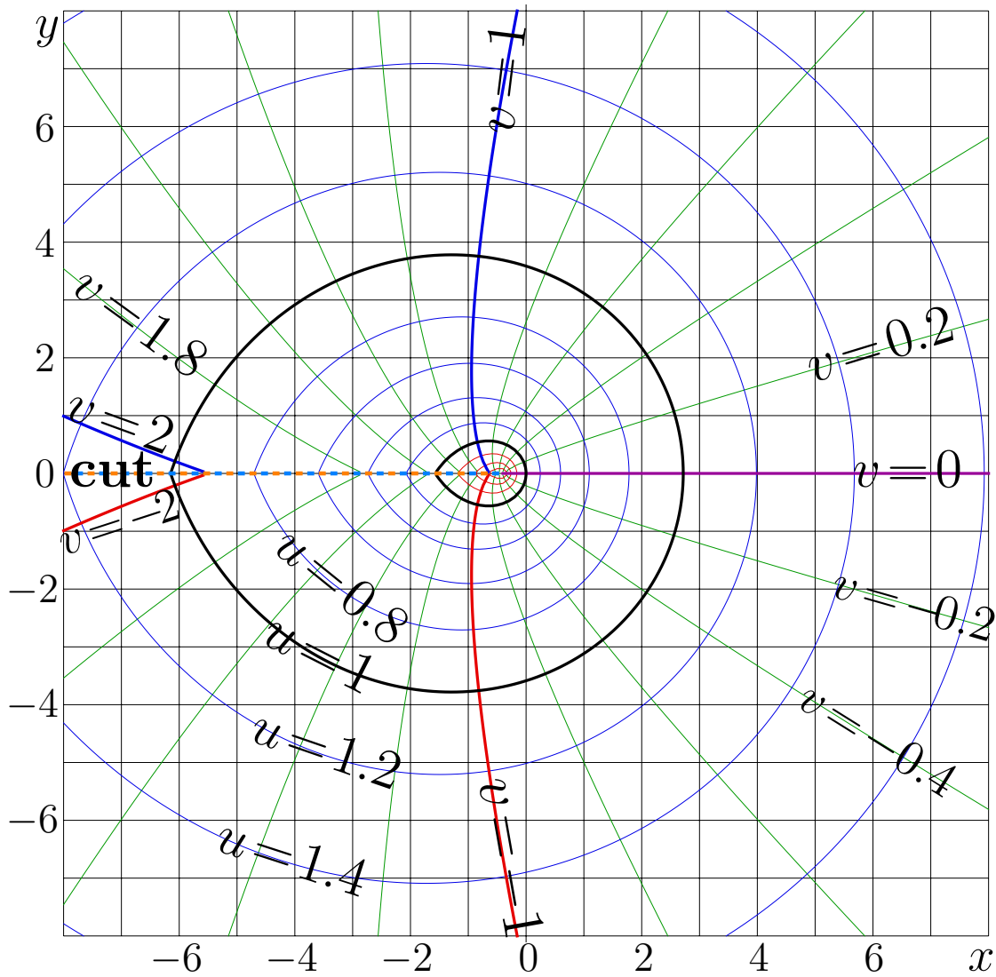
Figure 11.4: u+iv=\text{ArcZex}(x+iy)=\text{LambertW}(x+iy)
