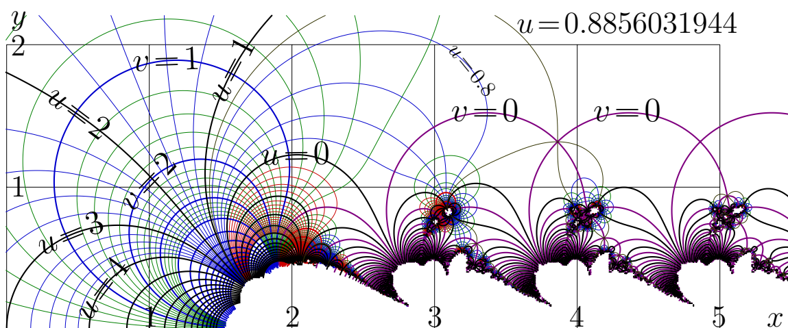
Figure 8.6: u+iv=\text{SuFac}(x+iy) and the zoom-in of the central part
