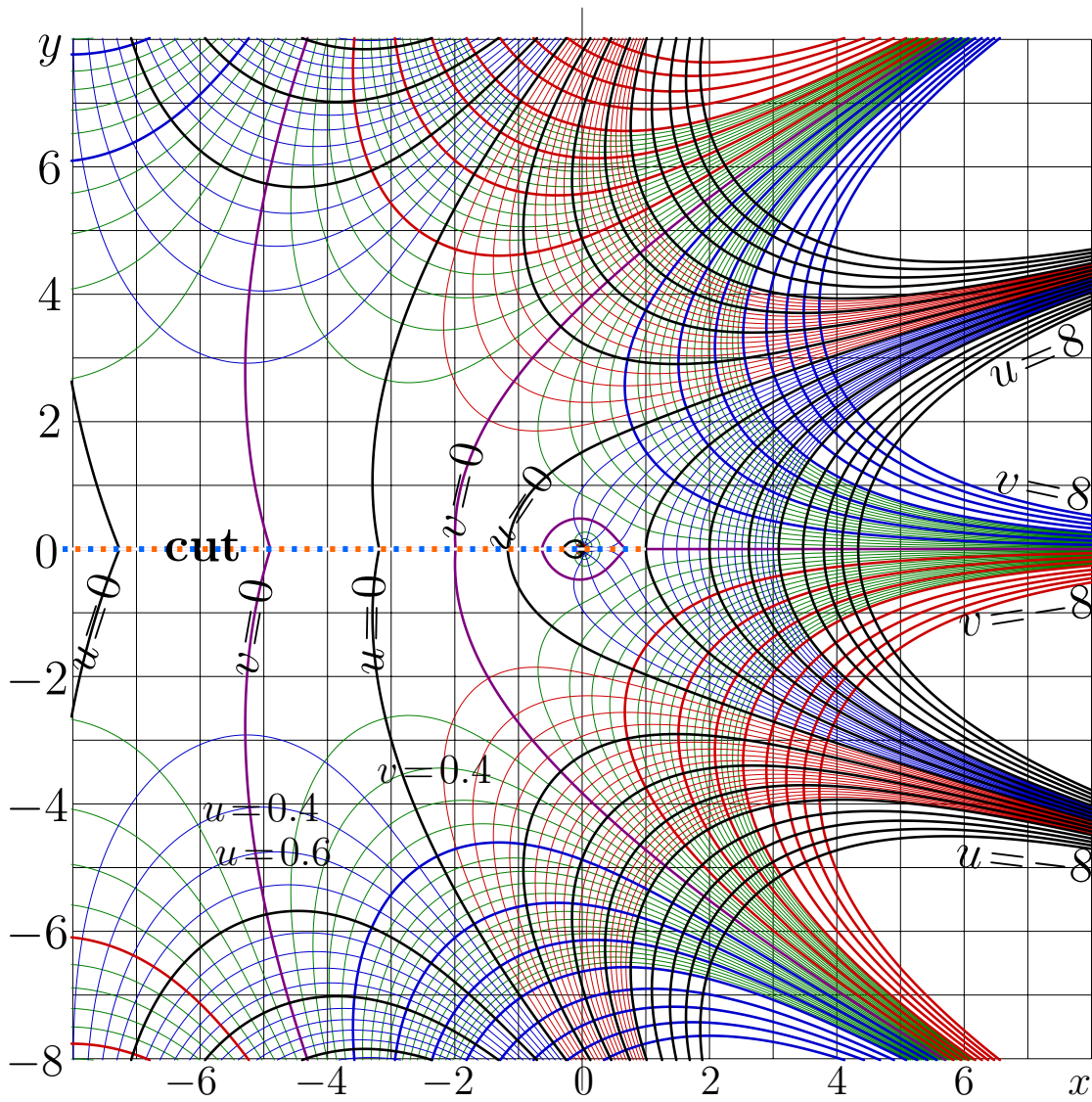
Figure 8.10: u+iv = \text{Factorial}^{0.5}(x+iy)
