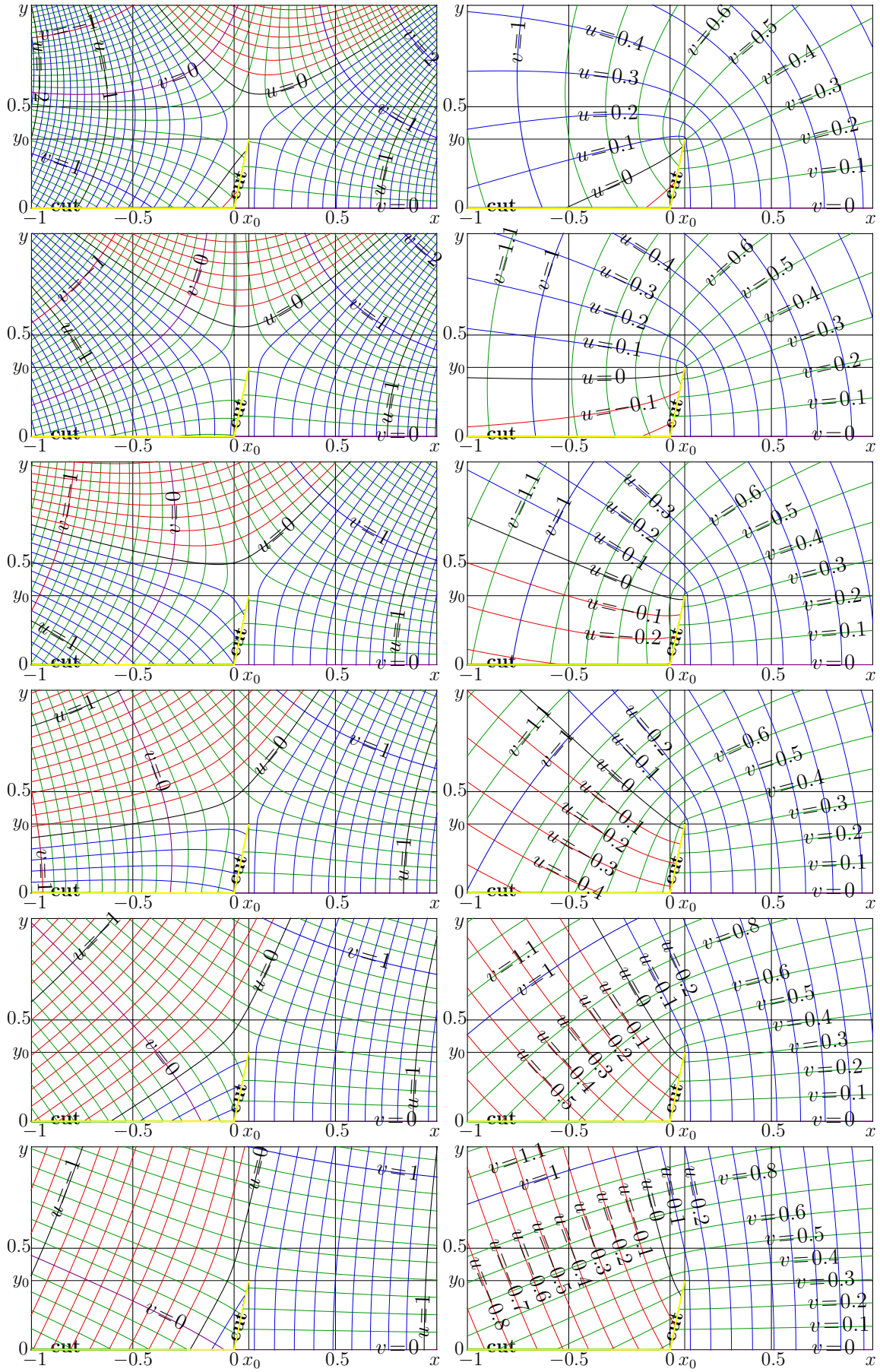
Figure 13.9: u+iv = \text{Nem}_1^n(x+iy) by (13.24) for n = 0.6 \dots 0.1 , left, and for n = -0.6 \dots -0.1 , right
