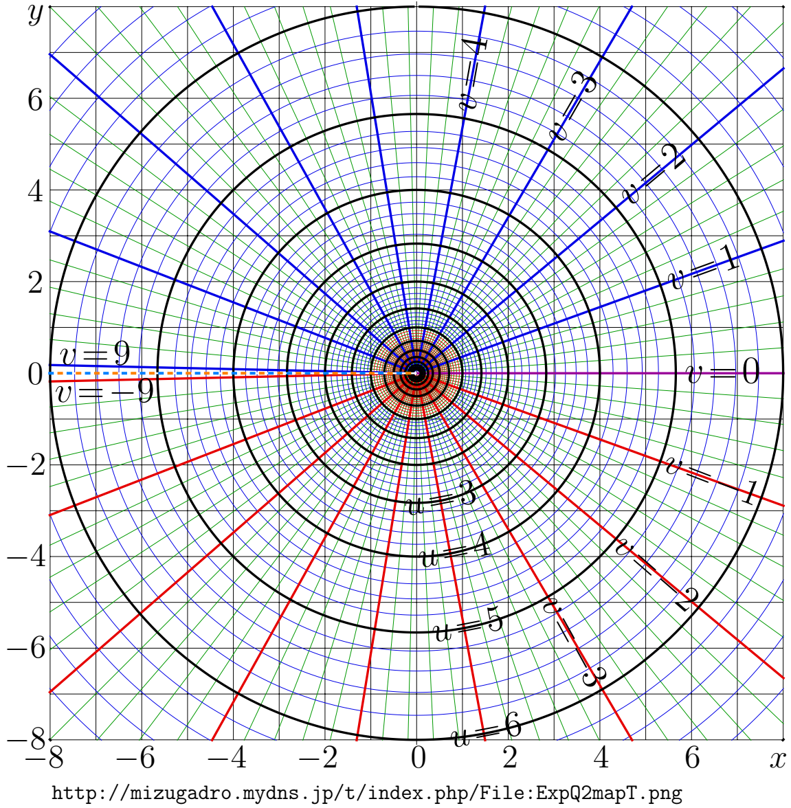
Figure 9.3: u+iv = \log_{\sqrt{2}}(x+iy)
