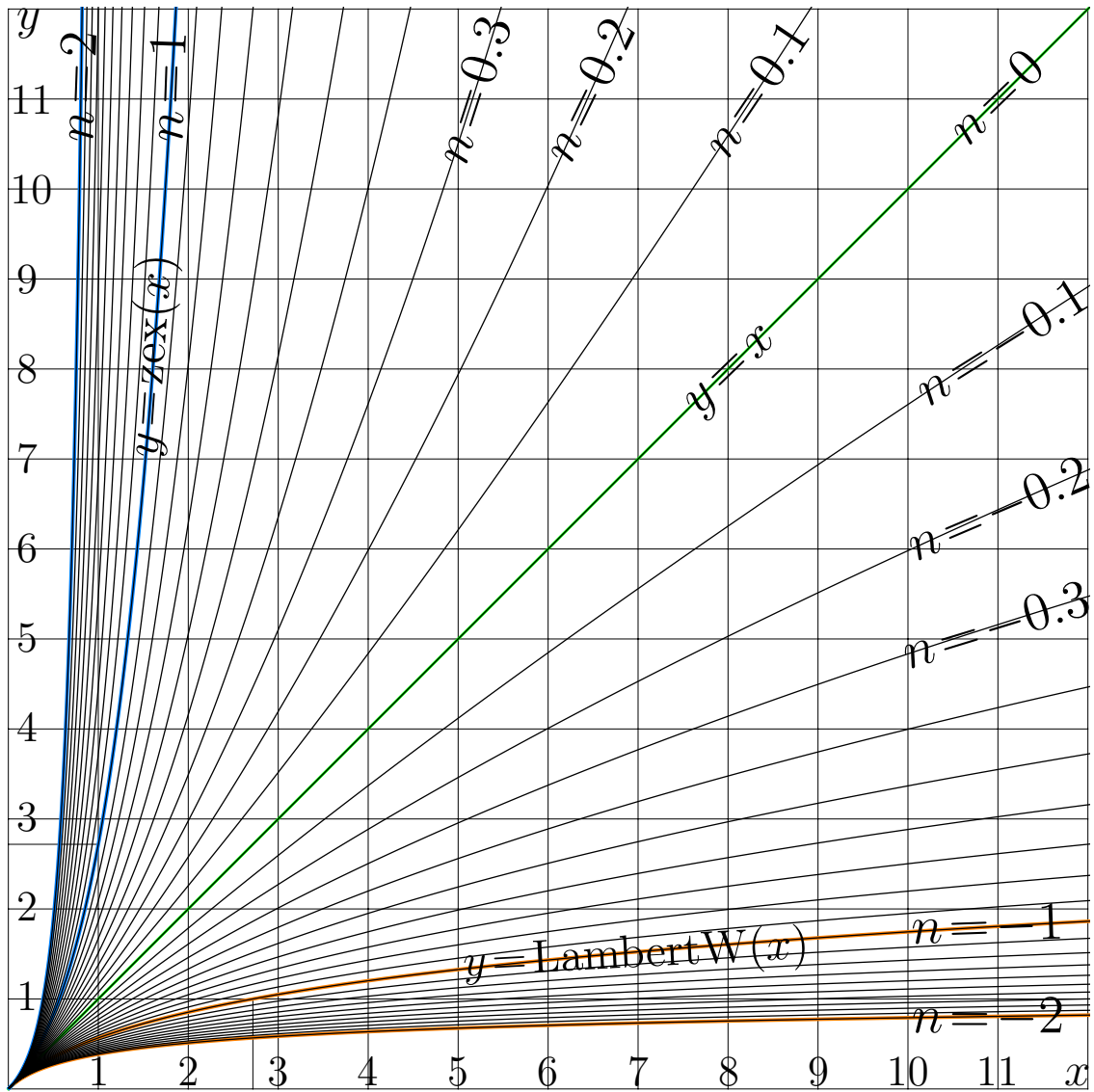
Fig. 11.8: y = \text{zex}^n(x) by (11.23) versus x for various n [zexiteplo]
