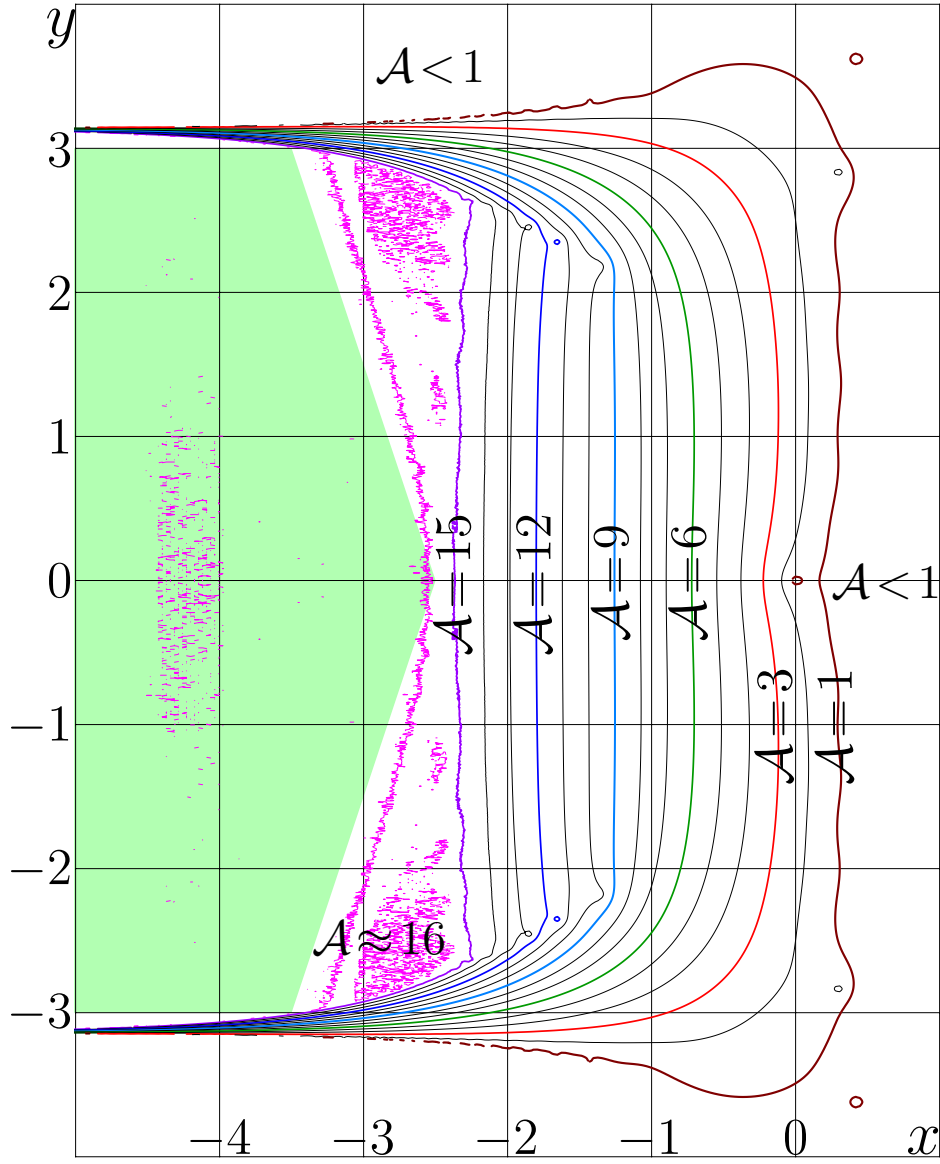
Fig. 20.10: Map of agreement \mathcal{A} = A(x+iy) by (20.50); range (20.49) is shaded \mathcal{A} = A(x+iy) по формуле (20.50) [autraAgreMap]
