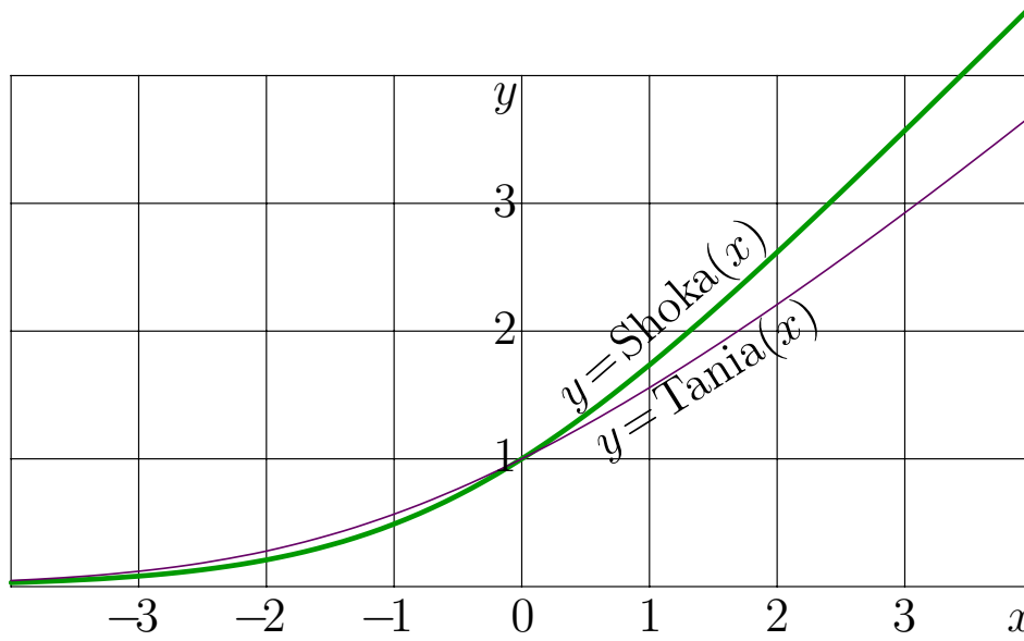
Fig. 5.1: Functions Tania and Shoka by (5.1) and (5.2) [shokataniaplot]
