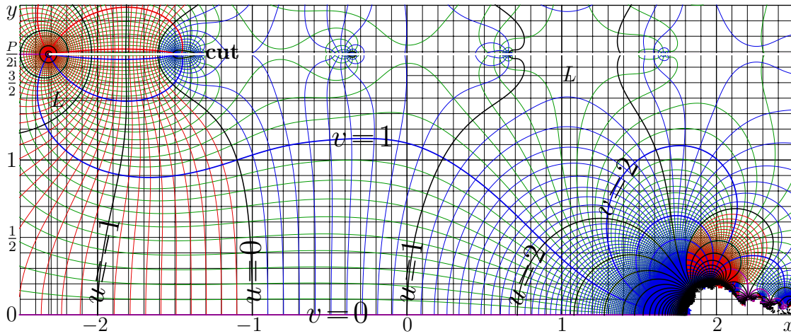
Fig. 19.6: u+iv = \text{pen}(x+iy) by (19.24), zoom-in from figure 19.5 [penzoo]
