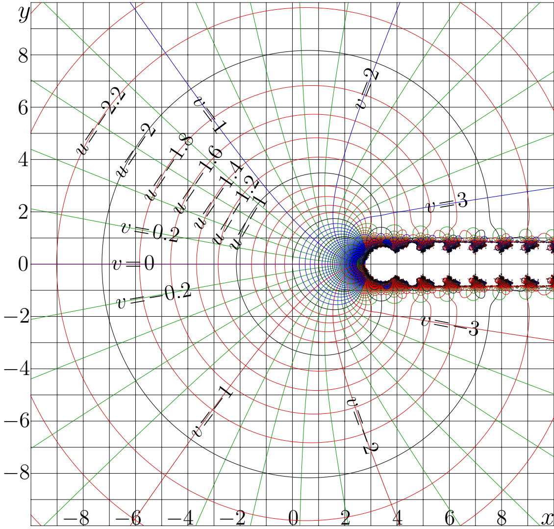
Fig. 20.6: u+iv = \text{SuTra}(x+iy) по формуле (20.33) [sutramap]
