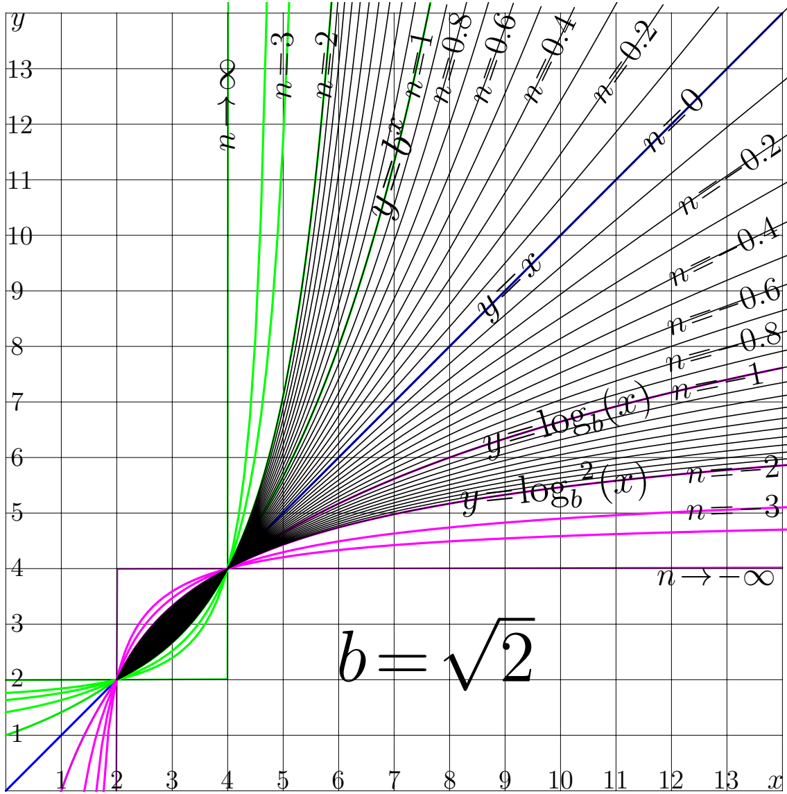
Fig. 9.8: y = \exp_{\sqrt{2},u}^n(x) by (9.23) for various n . [iterEq2plot]
