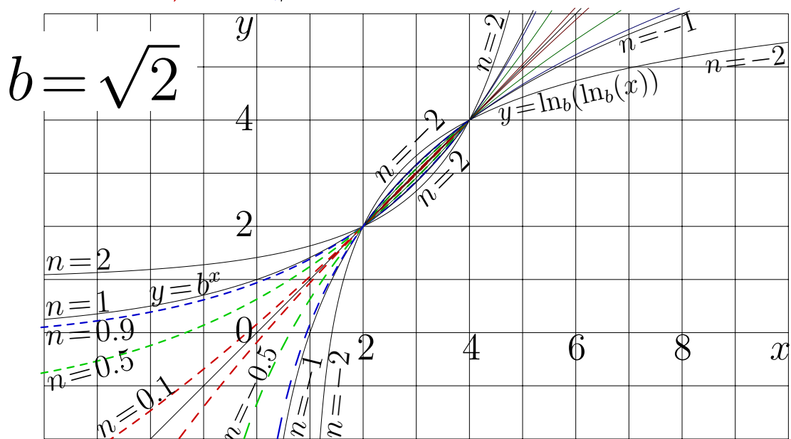
http://mizugadro.mydns.jp/t/index.php/File:E1e14z600.jpg Fig. 17.3: y = \exp^n_b(x) for various n at b=e , b=\exp(1/e) , b=\sqrt{2} [e1e14]
