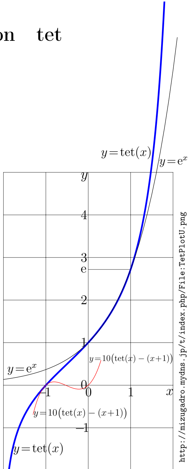
Fig. 14.1: y = \text{tet}(x) , y = \exp(x) , and y = 10(\text{tet}(x) - (x+1)) [TetPlot]
