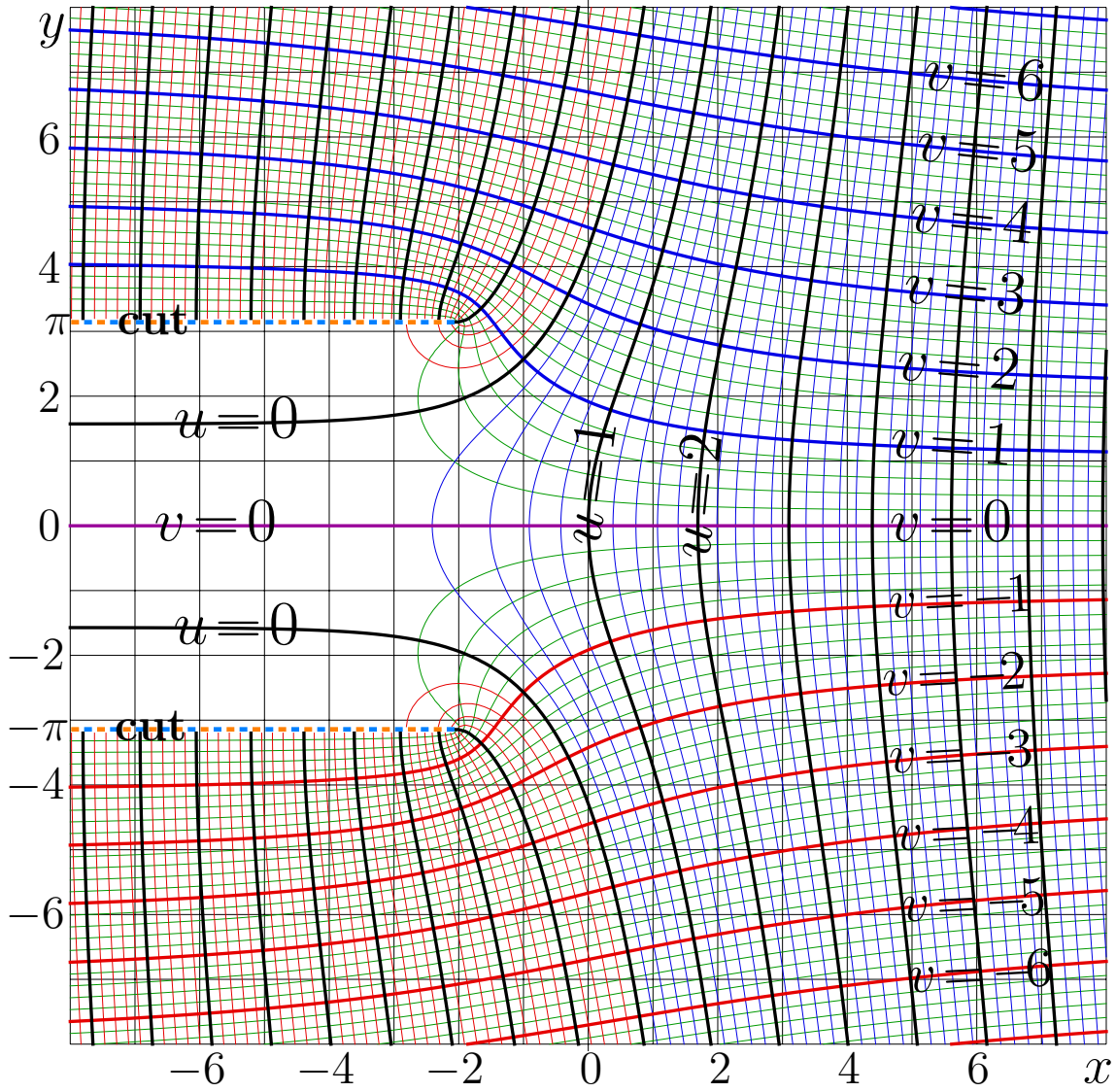
Fig. 5.2: Complex map of function Tania, u+iv=\text{Tania}(x+iy) [TaniaMap]
