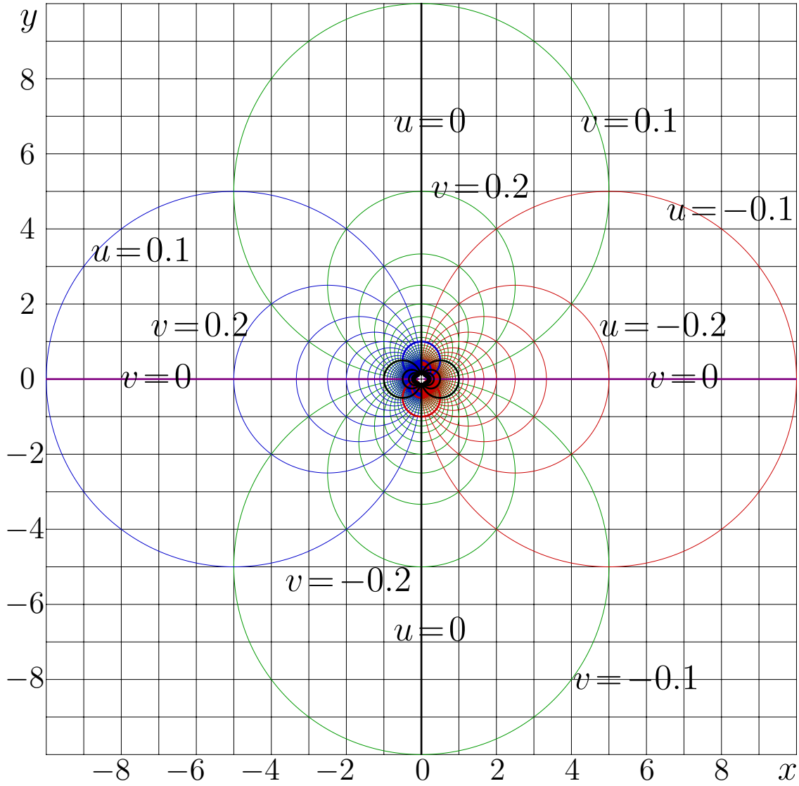
Fig. 4.4: u+iv=T(x+iy) = 1/(x+iy) [f1xmap]
