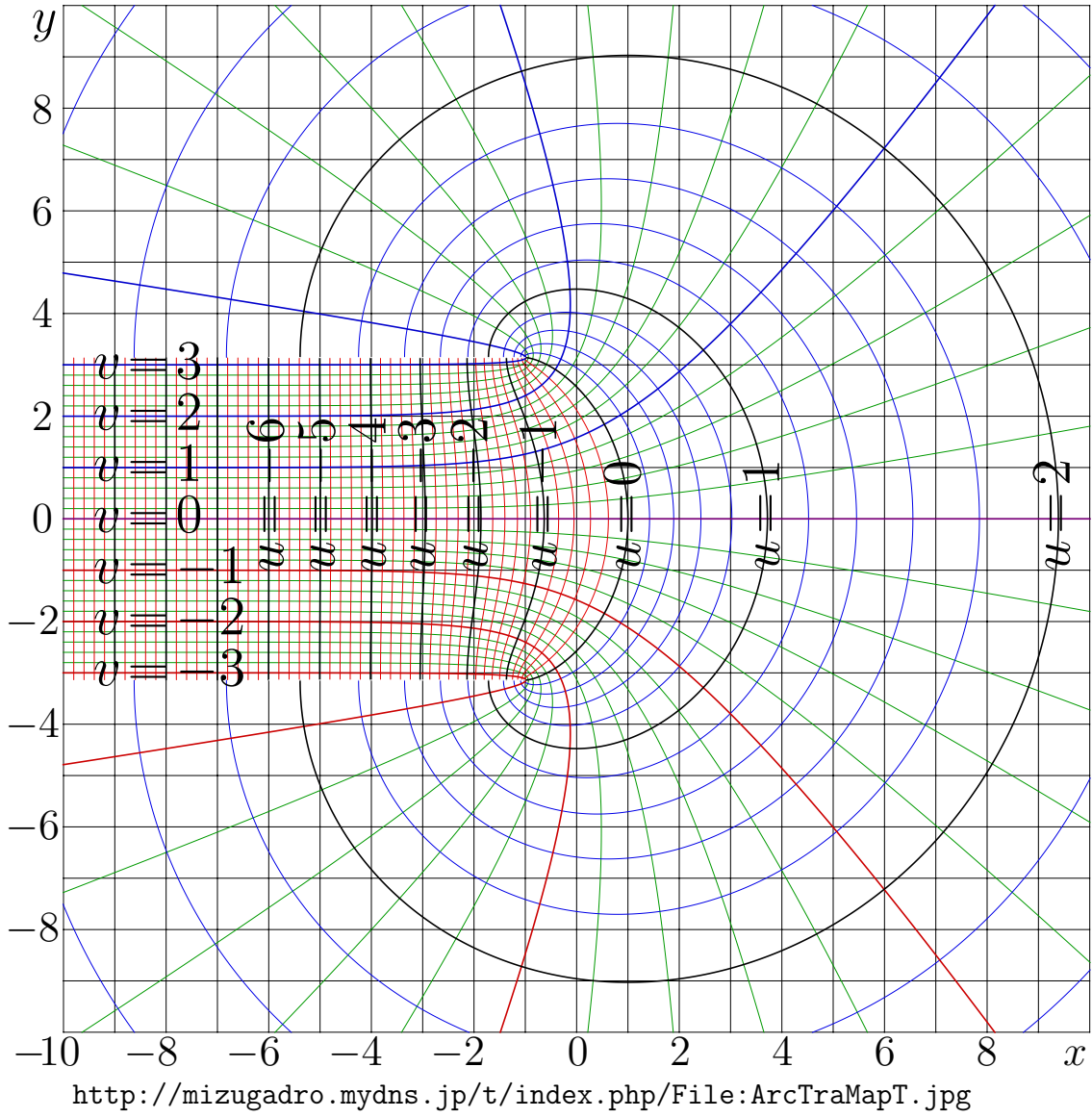
Fig. 20.3: u+iv = \text{ArcTra}(x+iy) [arctranmap]
