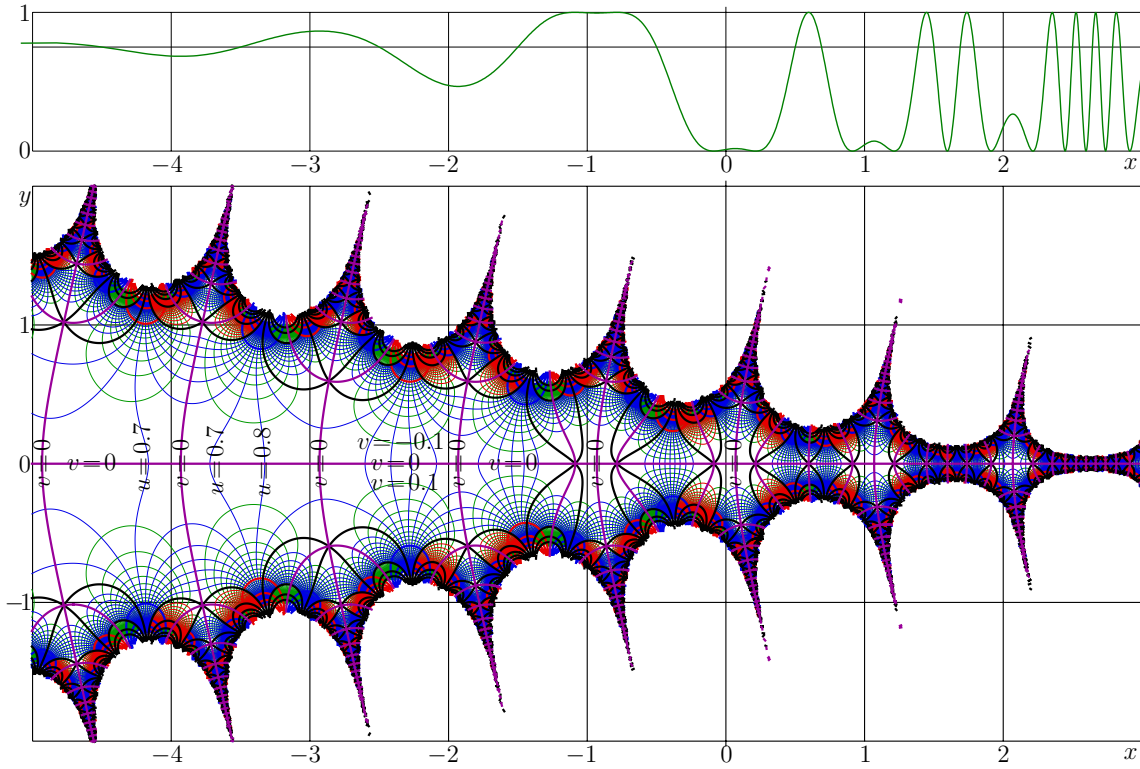
Fig. 7.15: Superfunction \text{Paw}_4(x) by (7.25),(6.12): explicit plot y = \text{Paw}_4(x) , top picture, and complex map u+iv = \text{Paw}_4(x+iy) , bottom picture, by (7.28) [logi5ab4]
