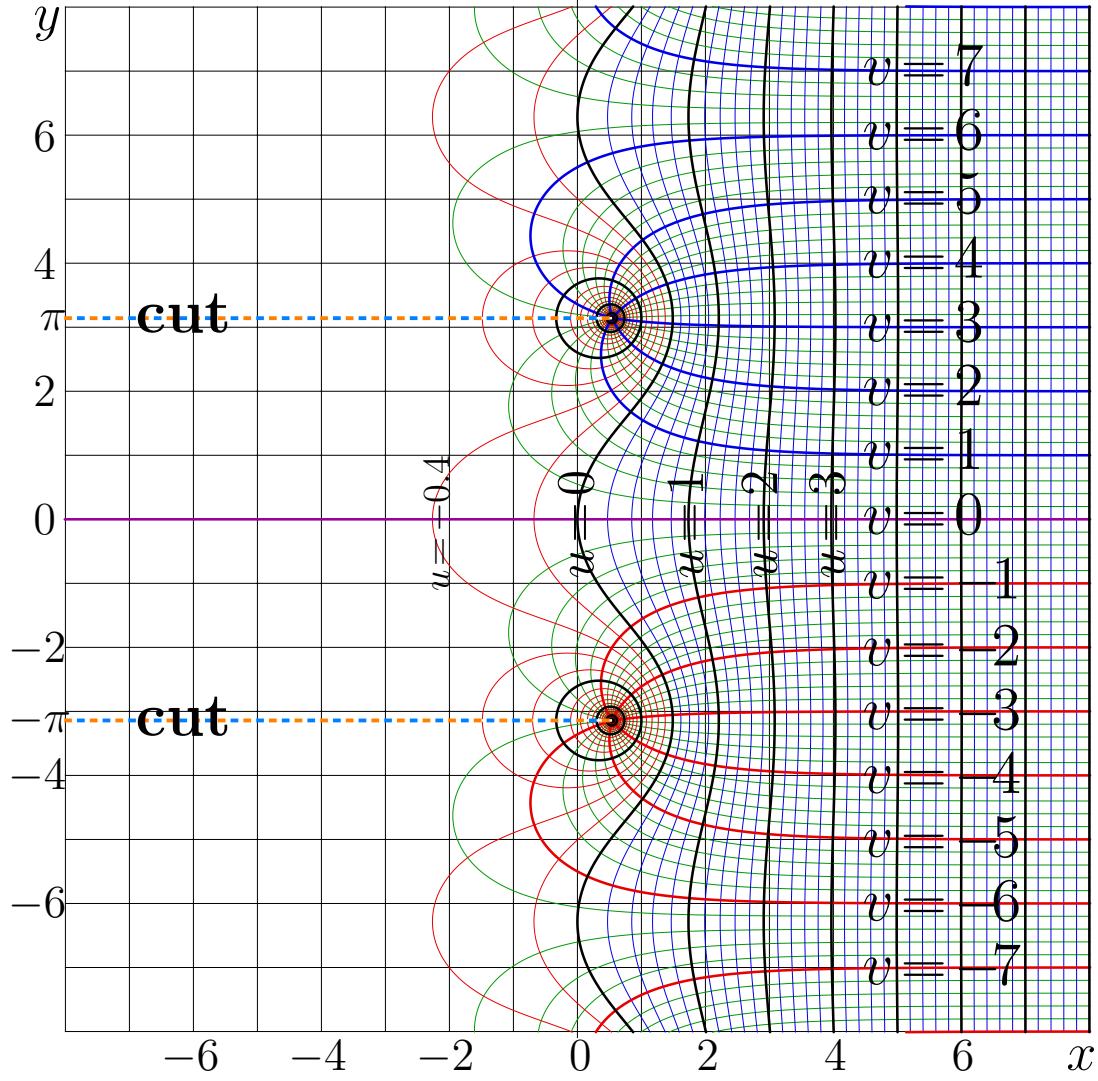
Fig. 5.8: u + v = \text{ArcKeller}(x + iy) by (5.16). [ArcKellerMap]
