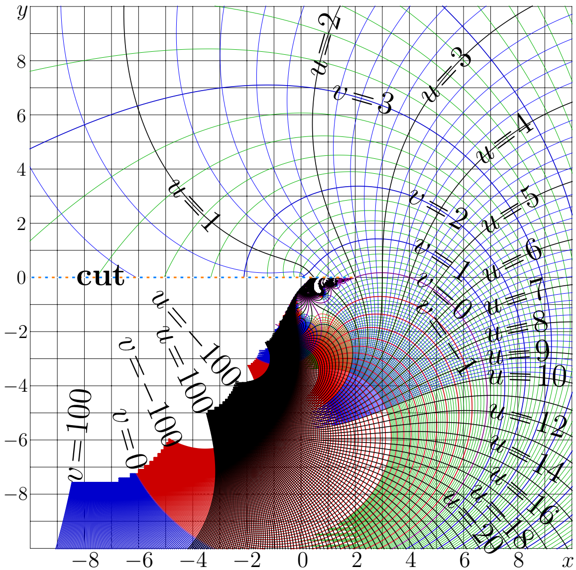
Fig. 16.11: u + iv = \exp_{\sqrt{2},u}^i(x + iy) по формуле (16.37) [sqrt2iimap2]
