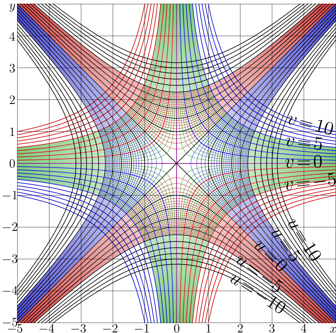
Fig. 4.11: u+iv = T(x+iy) = (x+iy)^2 , by (4.19) for a=2 [z2itmap]
