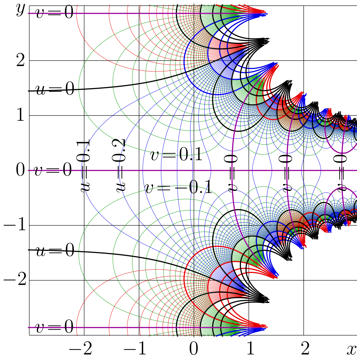
Fig. 7.4: u+iv = \text{Pav}_3(x+iy) by (7.8) [logi2c3]
