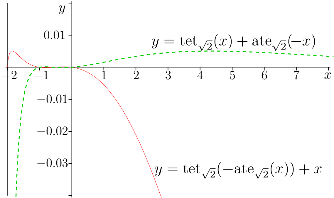
Fig. 16.5: Precision of “symmetry” of figure 16.1: y = \text{devia}(x) by (16.27), dashed, and y = \text{devib}(x) by (16.28), solid [sqrt27b]
