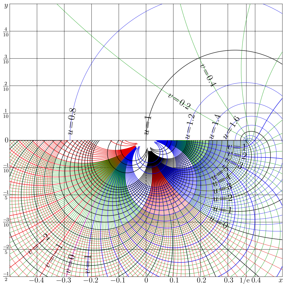
Fig. 18.2: u+iv = \text{flog}(x+iy) , zoom-in from the central part of figure 18.1 [flogzo2]
