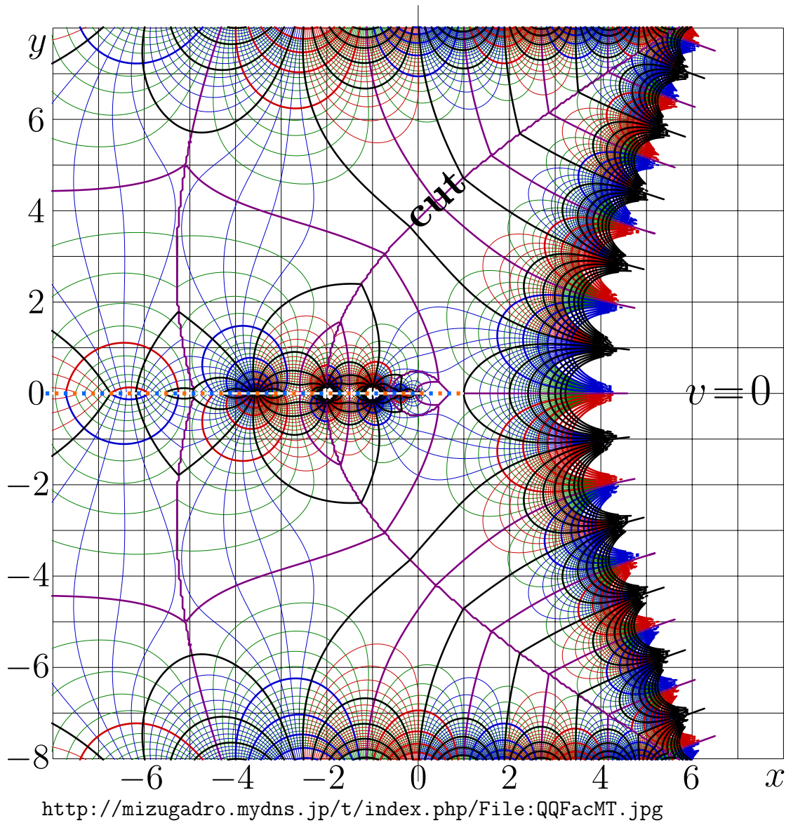
Fig. 8.11: u+iv = h^2(x+iy) . [QQFacMap]
