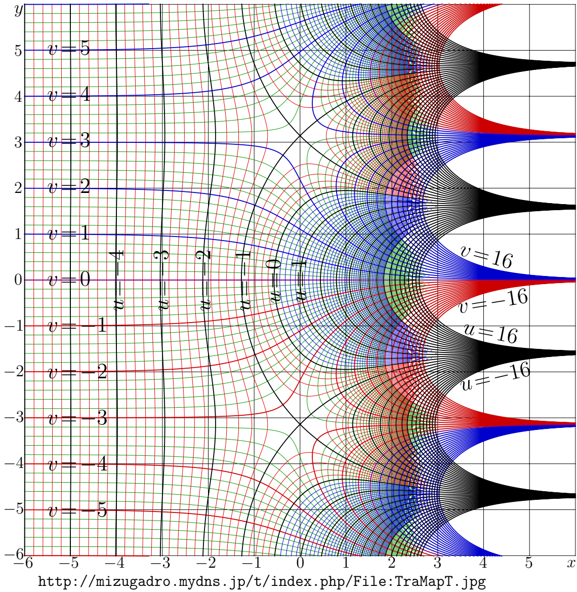
Fig. 20.2: u+iv = \text{tra}(x+iy) по формуле (20.1) [tramap]
