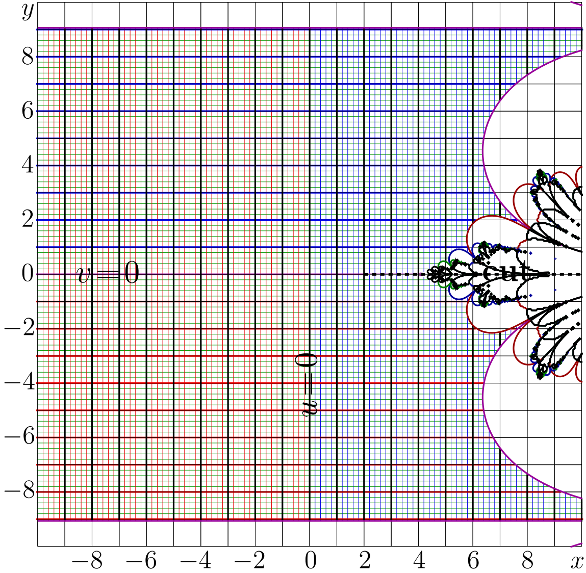
Fig. 16.4: u+iv = \text{tet}_{\sqrt{2}}(\text{ate}_{\sqrt{2}}(x+iy)) [sqrt2tetate]
