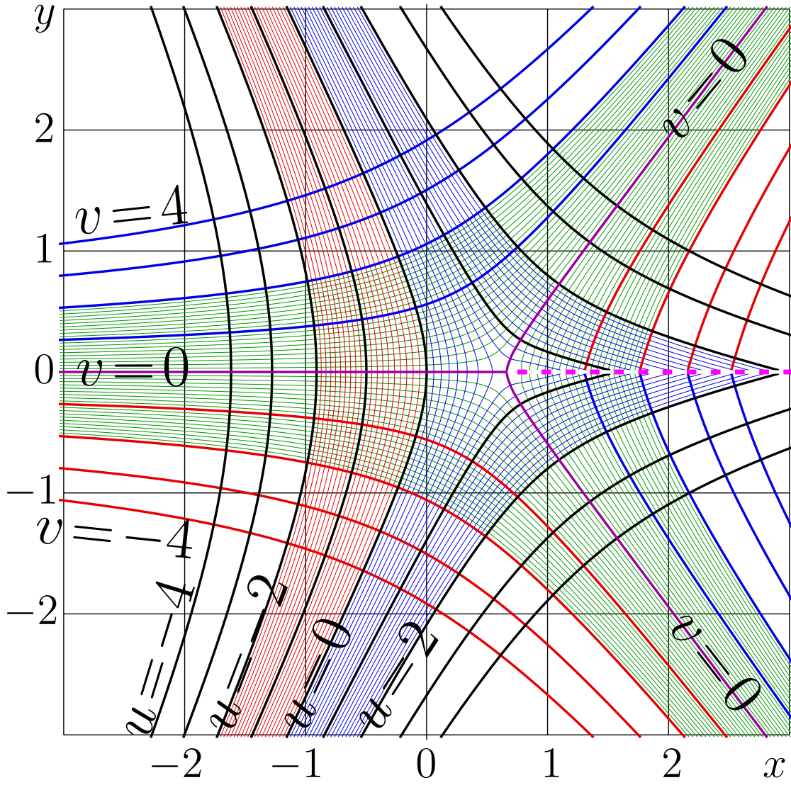
Fig. 7.10: u+iv = \text{Elu}_3^{1/2}(x+iy) . [logi2b3]
