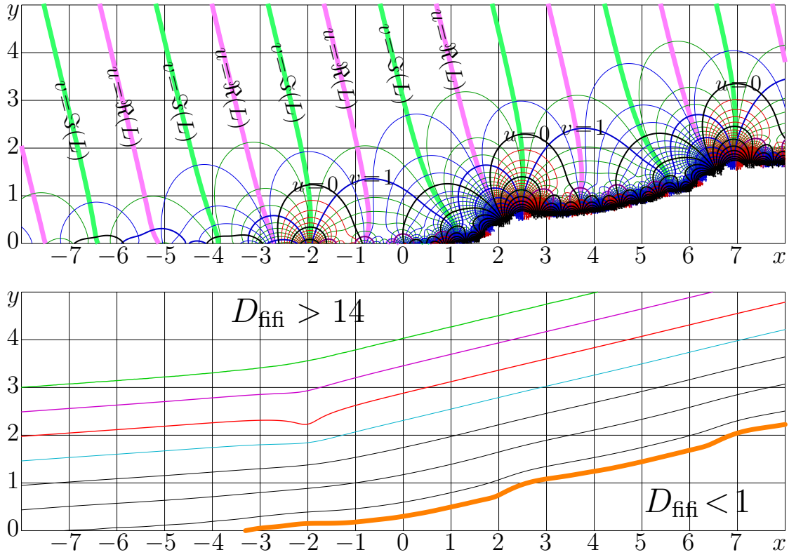
Fig. 14.9: Top: u+iv = \text{fima}(x+iy) by (14.45); bottom: map of D_{\text{fifi}} = D_{\text{fifi}}(x+iy) by (14.55) [figfima]
