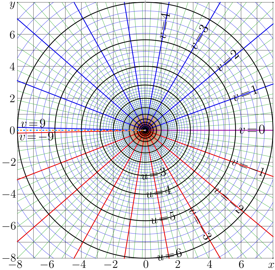
Fig. 9.3: u+iv = \log_{\sqrt{2}}(x+iy) [LogQ2map]
