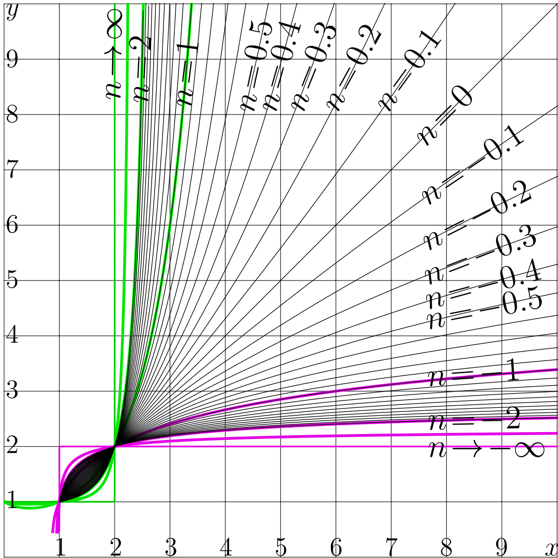
Fig. 8.9: y = \text{Factorial}^n(x) versus x for various n [facit]
