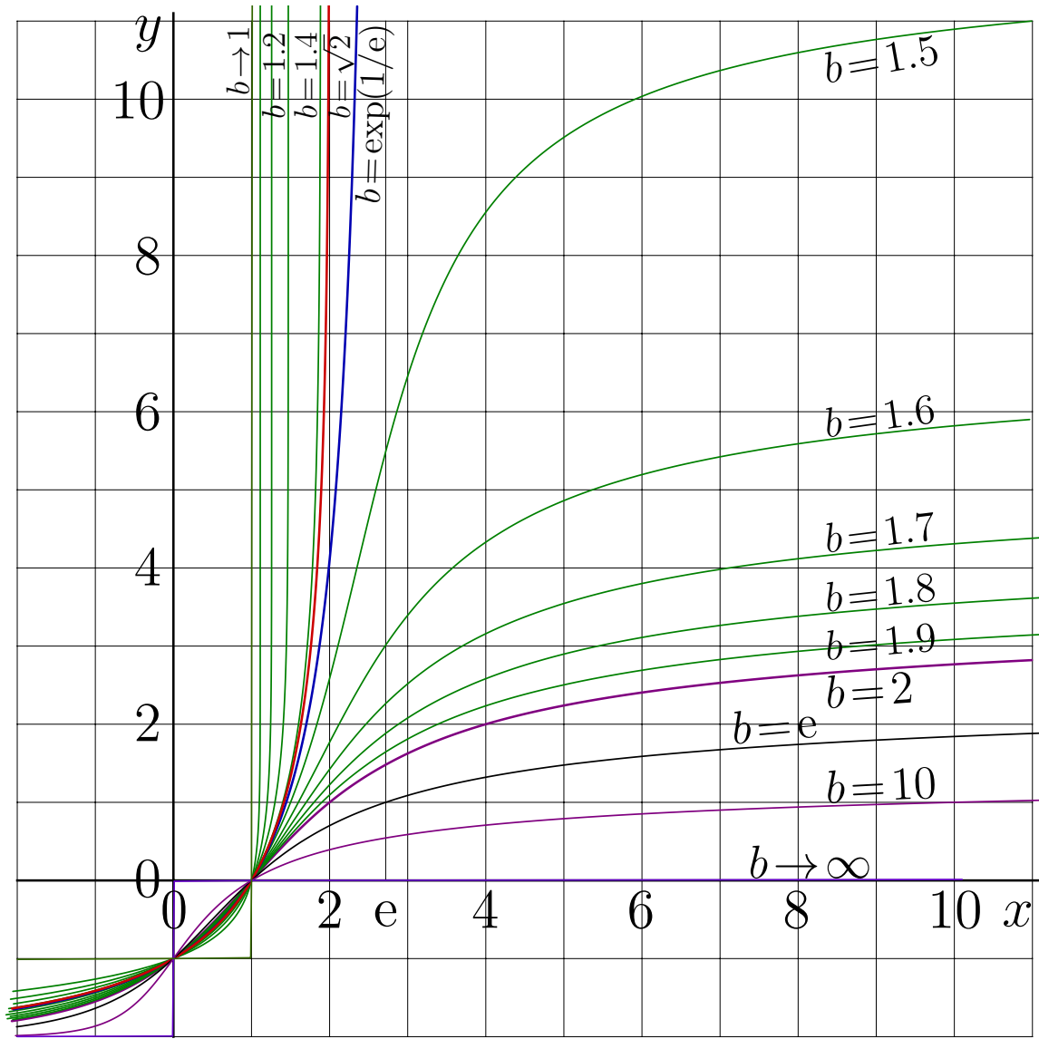
Fig. 17.2: y = \text{ate}_b(x) for various b [ate10bx]
