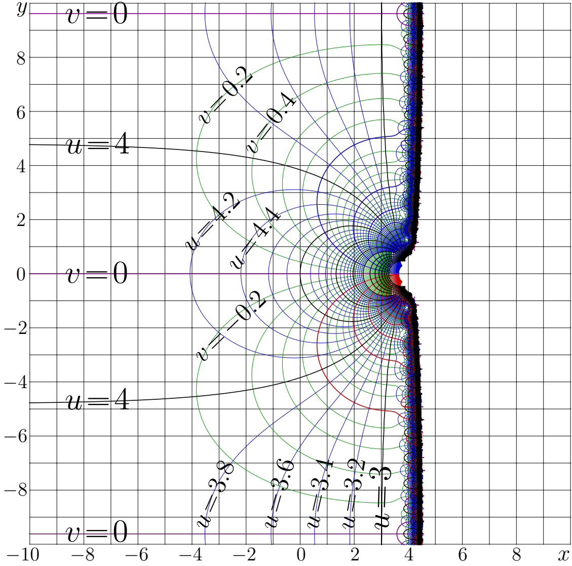
http://mizugadro.mydns.jp/t/index.php/File:Sqrt2figf45bT.png Fig. 9.5: u+iv = \tilde{f}(x-1.11520724513161 + iy) ; [sqrt2figf45b] [mapeq2F4]
