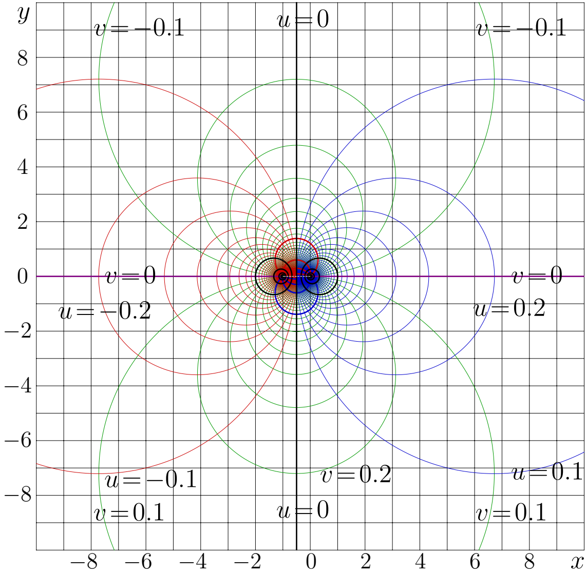
Fig. 4.10: u+iv = g(x+iy) by (4.16) at c=2 [gzfracmap]
