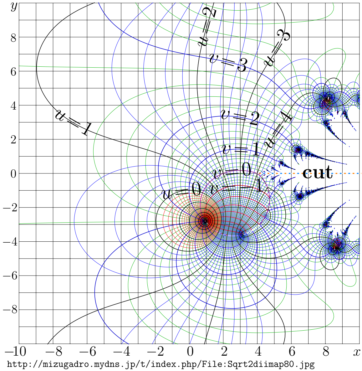
Fig. 16.10: u+iv = \exp_{\sqrt{2},d}^i(x+iy) by (16.36) [sqrt2iemap1]
