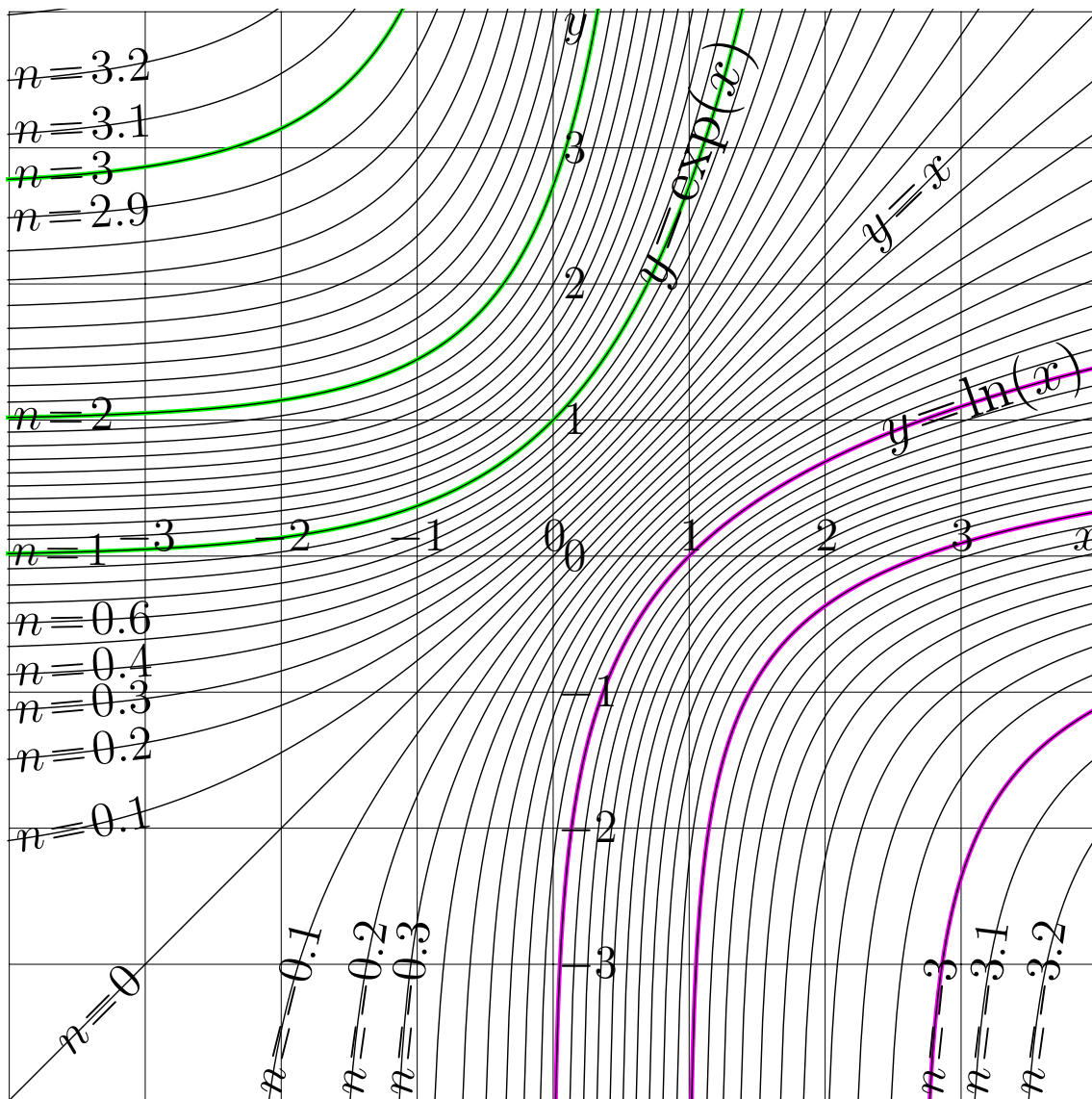
Fig. 15.4: y = \exp^n(x) by (15.15) for various n [expiteplot]
