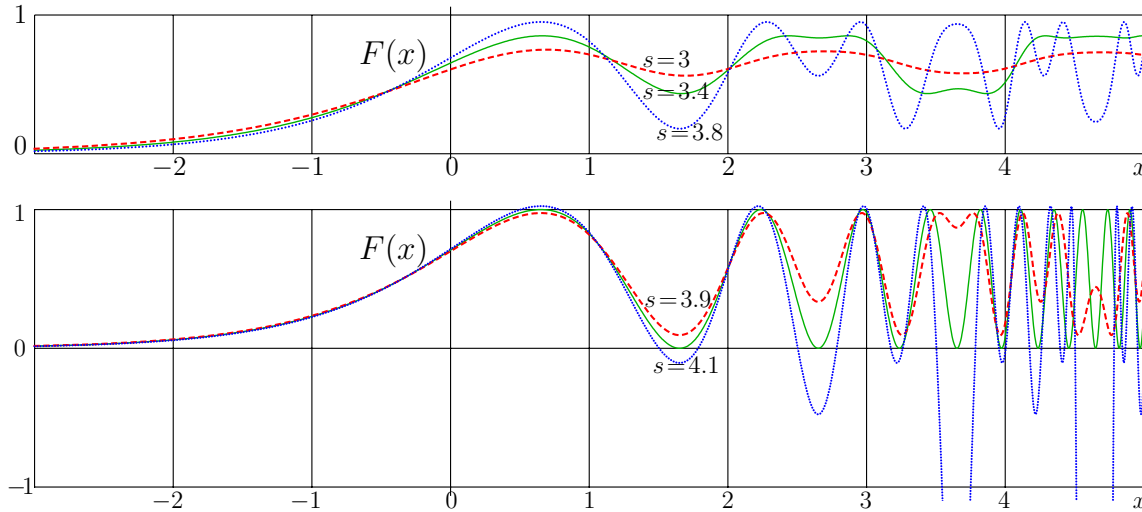
Fig. 7.3: \text{Pav}_s(x) by formulas (7.4), (6.12), (7.8) for s=3 , s=3.4 , s=3.8 , at the top picture, and for s=3.9 , s=4 , s=4.1 , bottom. [logi56]
