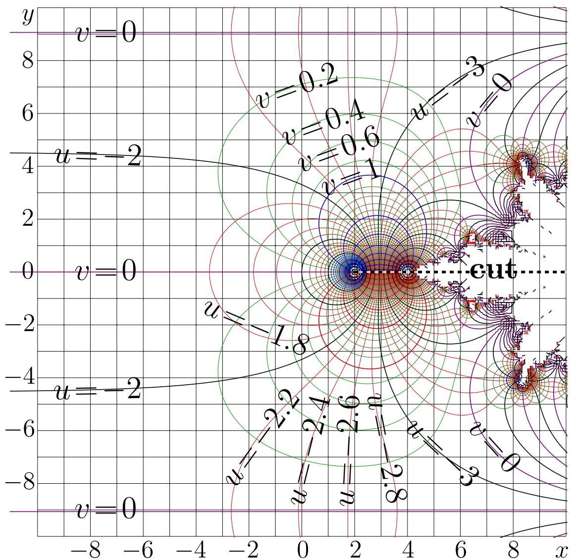
Fig. 16.3: u+iv = \text{ate}_{\sqrt{2}}(x+iy) [sqrt2atemap]
