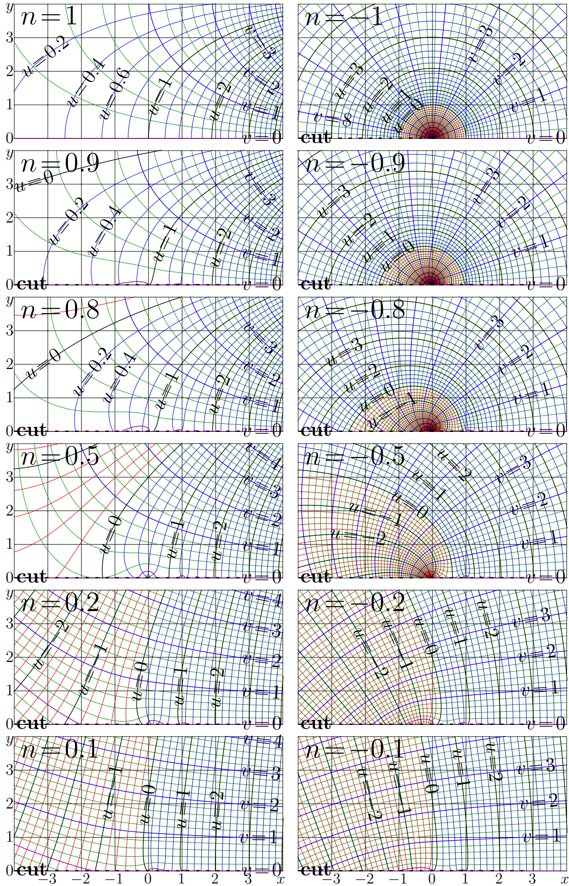
Fig. 10.10: u+iv = \exp_{\eta,u}^n(x+iy) , complex maps of iterates of exponent to base \eta by equation (10.53) for various n [e1e000map]
