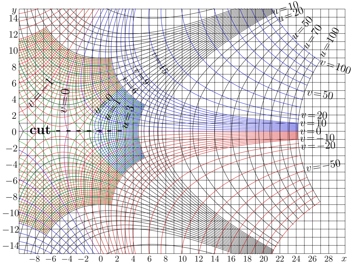
Fig. 10.9: u+iv = \exp_{\eta,u}^{1/2}(x+iy) by (10.53) for n=1/2 [e1eghalf]
