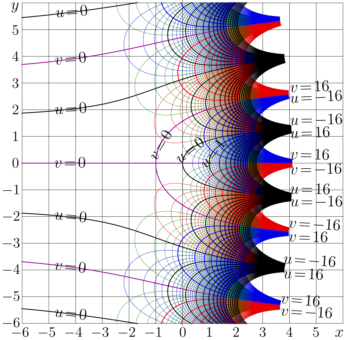
Fig. 6.5: u+iv = \text{Anka}(x+iy) by (6.27)
