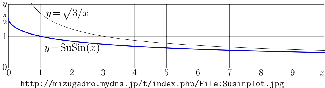
Fig. 12.1: y = \text{SuSin}(x) by (12.8) and its asymptotics (12.3) [susinplot]
