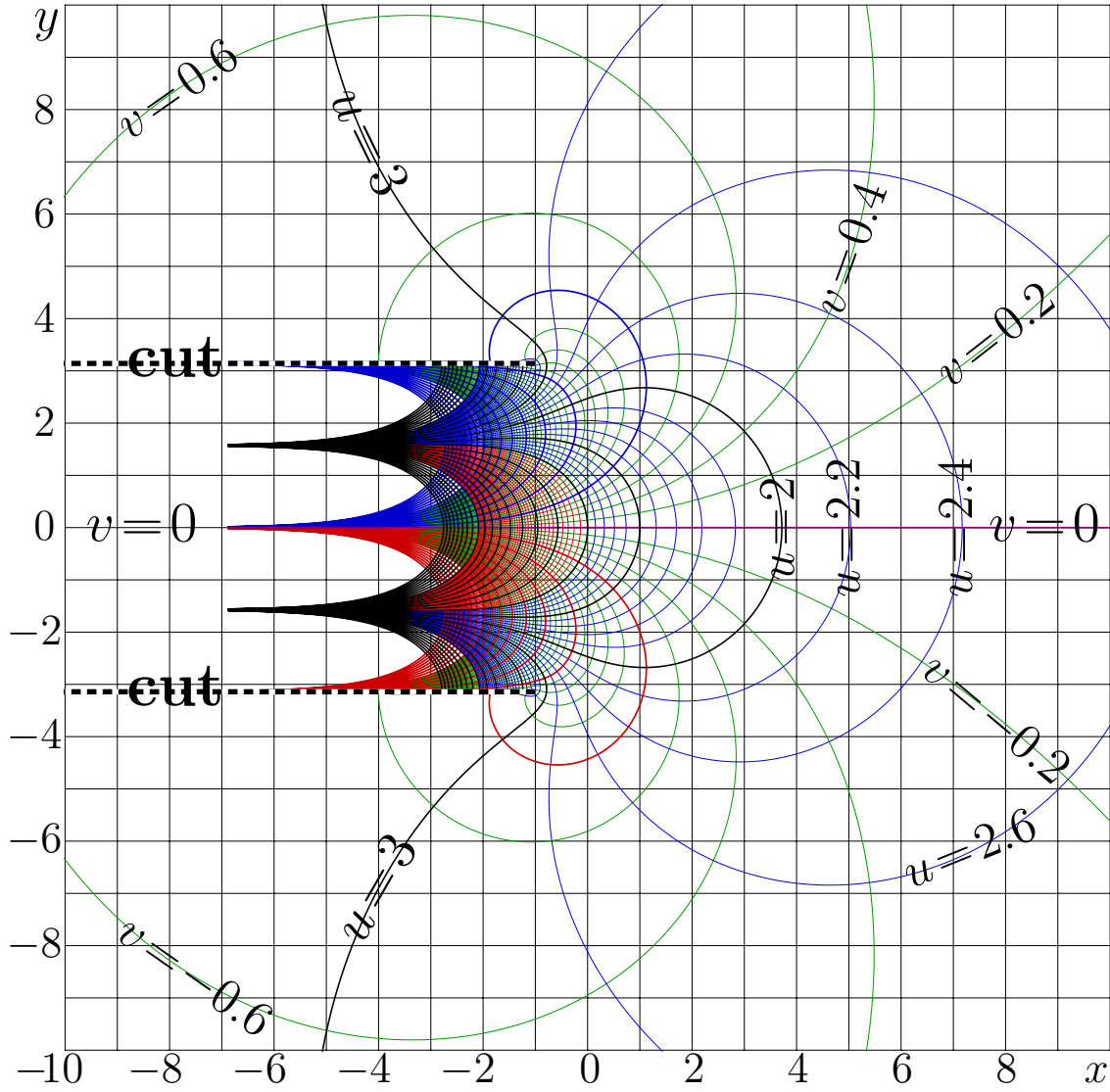
Fig. 20.11: u+iv = \text{AuTra}(x+iy) [autraMap]
