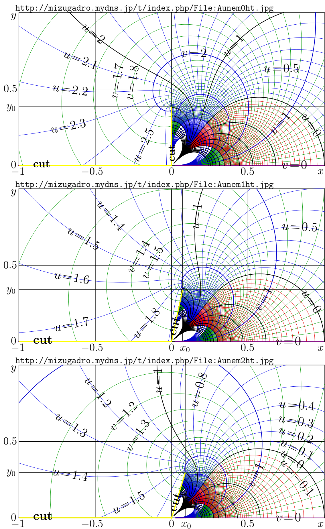
Fig. 13.7: u+iv = \text{AuNem}_q(x+iy) for q=0, q=1, q=2 [aunema]
