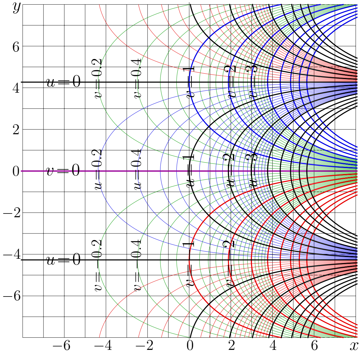
Fig. 10.3: u+iv = \exp_{\eta}(x+iy) [expe1emap]
