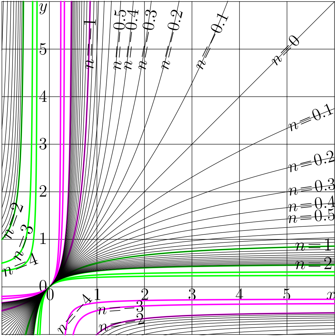
Fig. 4.7: y=t^n(x) by (4.13) at c=1 [c10]
