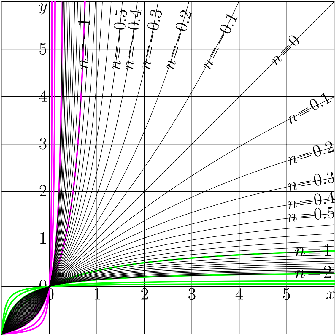
Fig. 4.8: y = t^n(x) by (4.13) at c=2 [c20]
