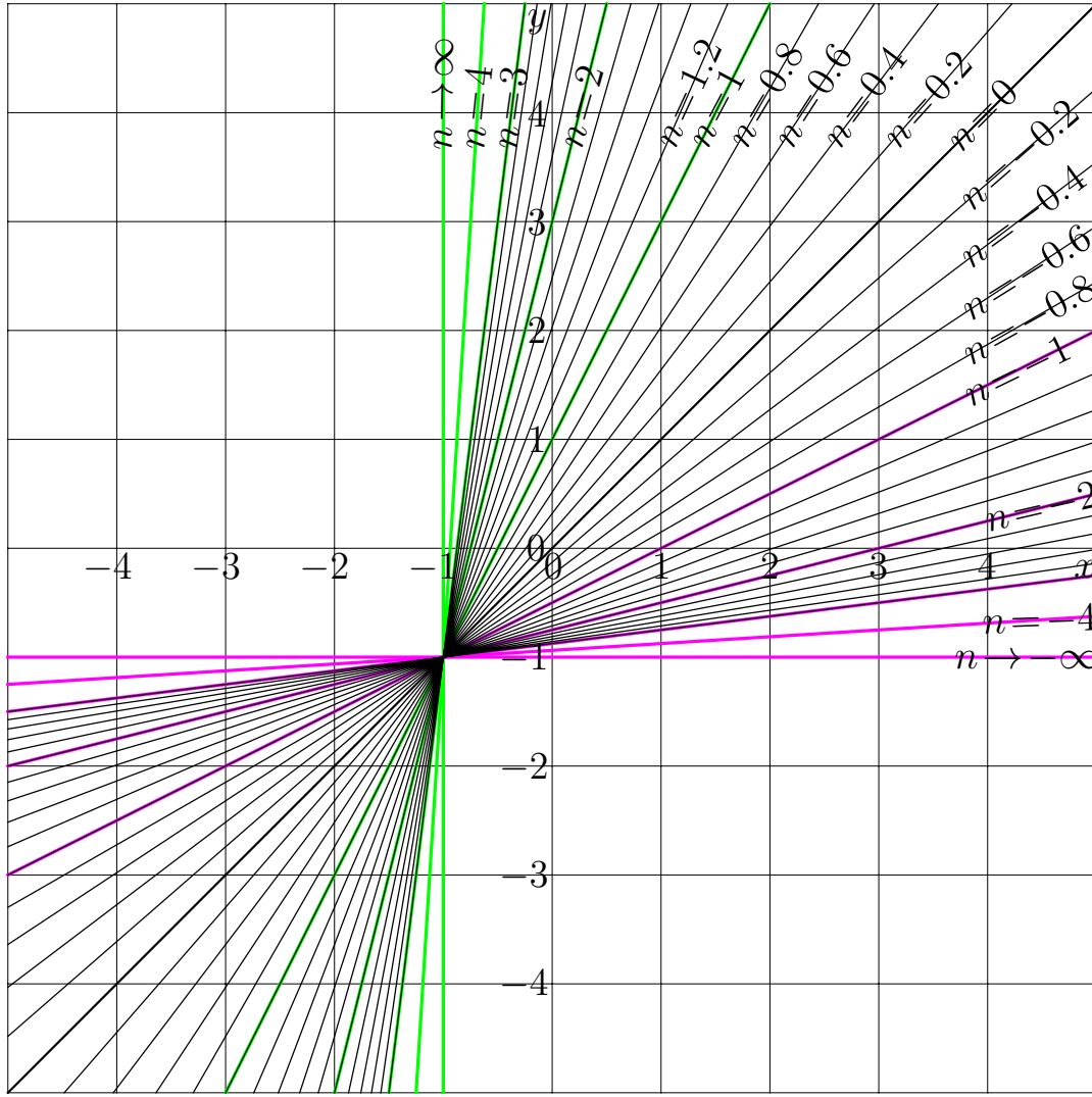
http://mizugadro.mydns.jp/t/index.php/File:Itelin125T.jpg Fig. 4.2: Iterates of linear function (4.1) at A = 1 , B = 2 ; y = T^n(x) versus x for various n [itelin125]
