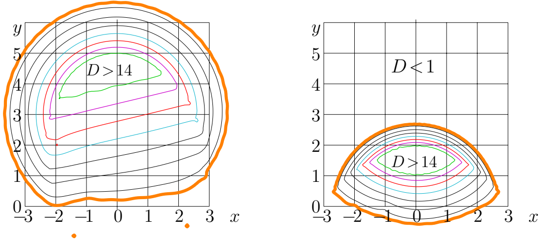
Fig. 14.10: Comparison of approximations tai by (14.40) to fima by (14.45) and to maclo by (14.36): agreements D = D_6(x+iy) and D = D_7(x+iy) by (14.56),(14.57) in the complex z -plane. [figco] [vladi07]
