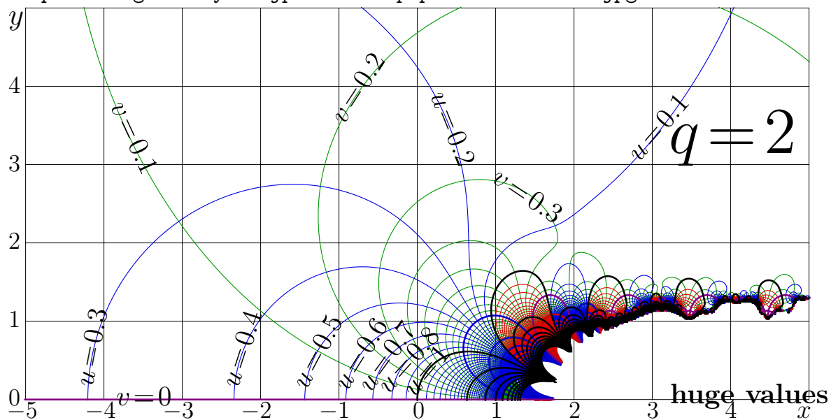
Fig. 13.6: u+iv = \text{SuNem}_q(x+iy) , for q=0, 1, 2 [suma]
