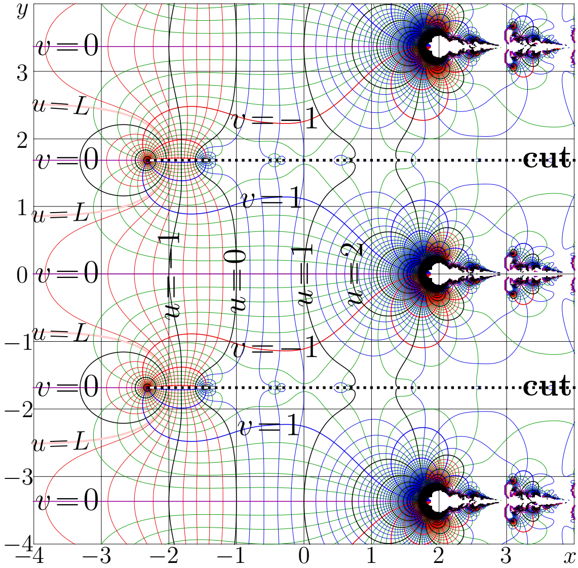
Fig. 19.5: u+iv = \text{pen}(x+iy) по формуле (19.24) [penmap]
