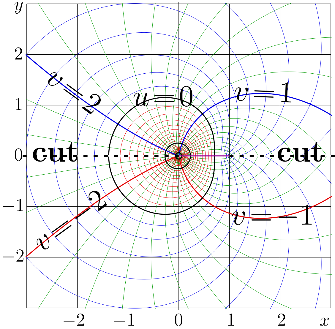
Fig. 7.8: u+iv = \text{ArcPav}_4(x+iy) . [logi2d4]
