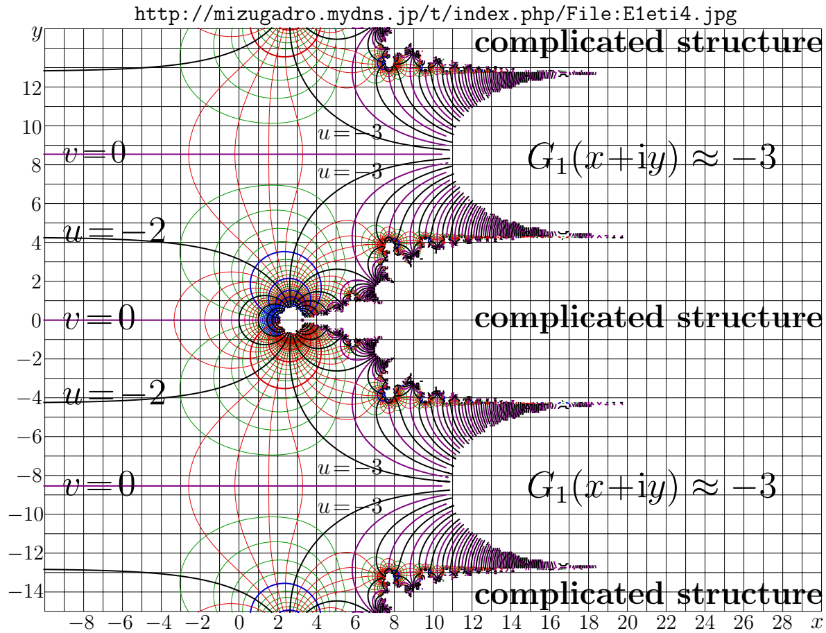
Fig. 10.7: u+iv = G_3(x+iy) = \text{AuExp}_{\eta,3}(x+iy) by (10.50), top map, and u+iv = G_1(x+iy) = \text{ate}_{\eta}(x+iy) by (10.49), map at the bottom [e1efig3]
