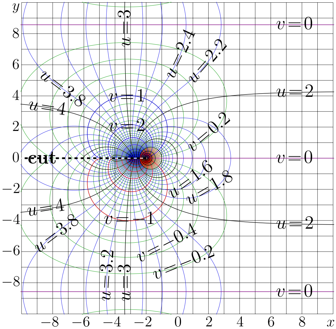
Fig. 16.2: u+iv = \text{tet}_{\sqrt{2}}(x+iy) [sqrt2tetmap]
