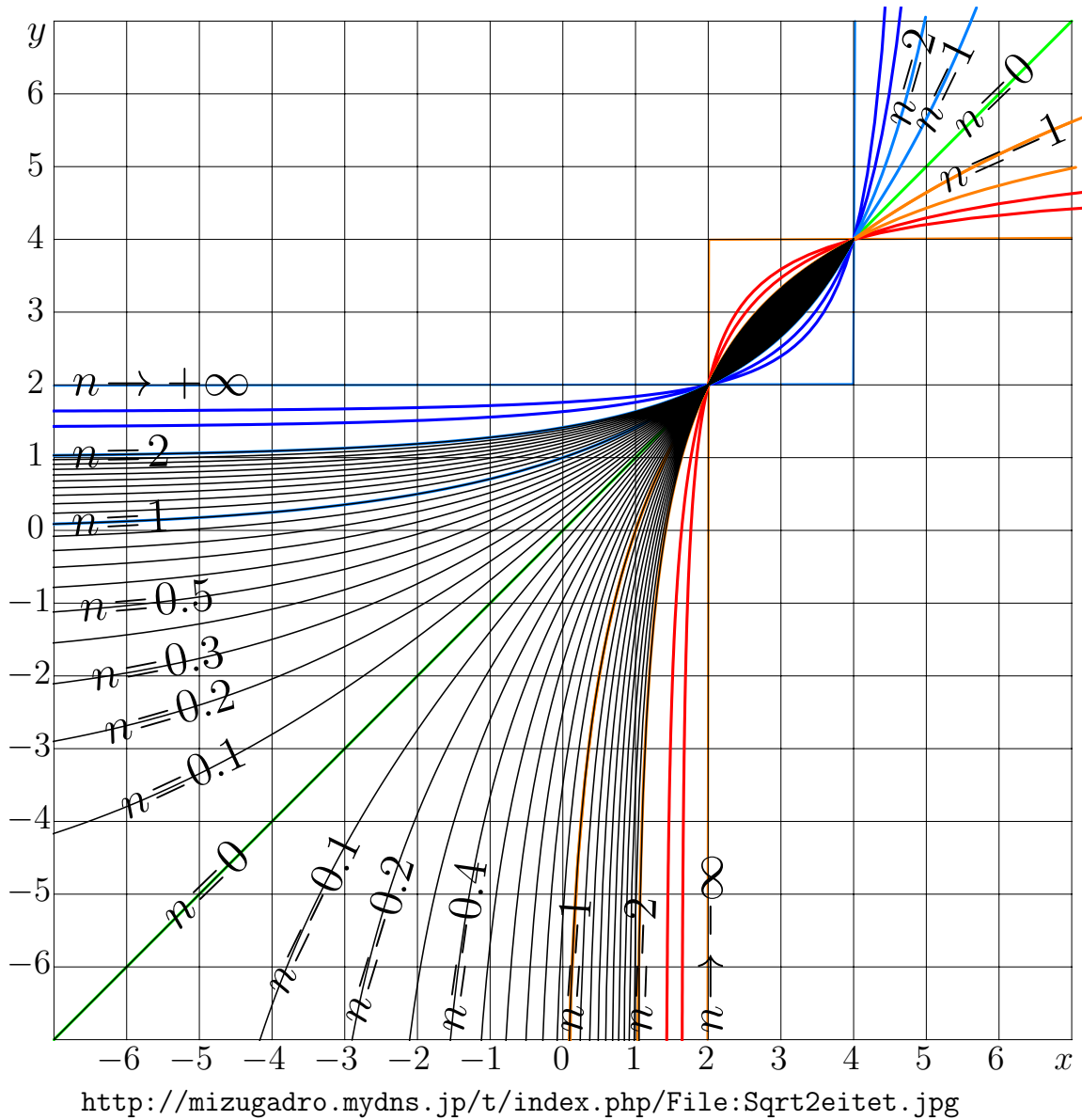
Fig. 16.6: y = \exp_{\sqrt{2},u}^n(x) for various n [sqrt2eitet]
