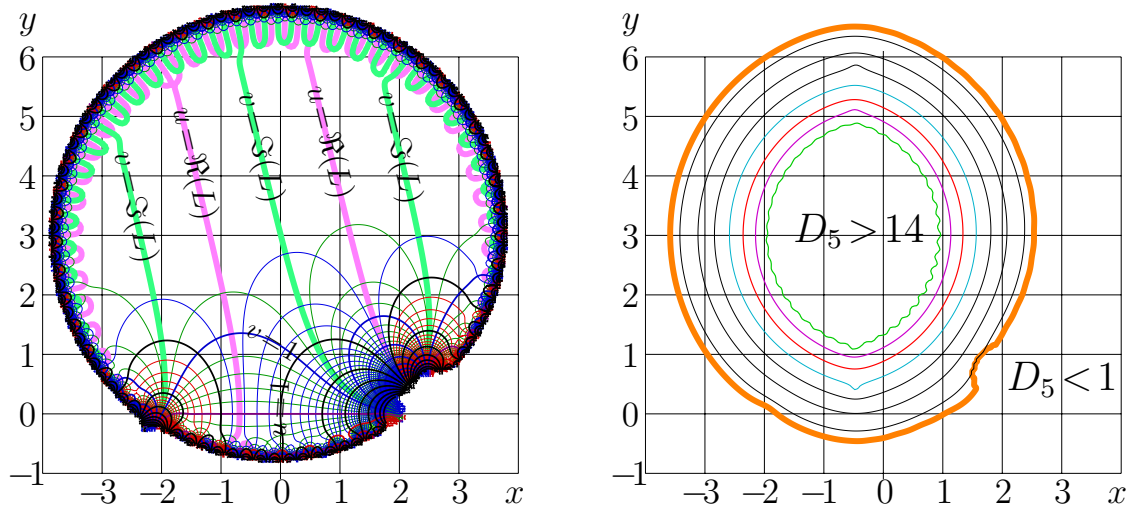
Fig. 14.8: u+iv = \text{tai}(x+iy) by (14.40) at N=51 and agreement D_5(x+iy)
