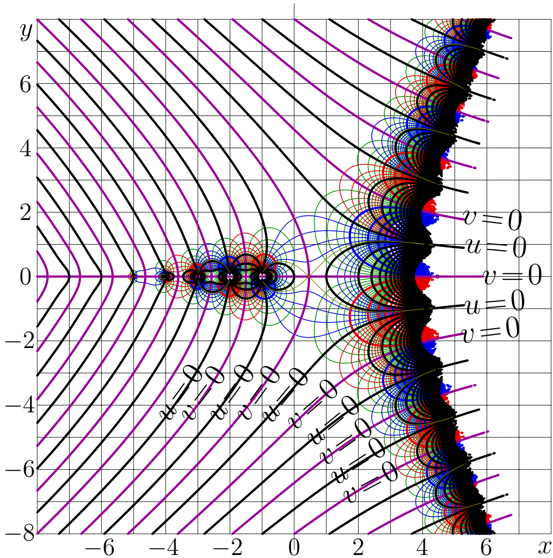
Fig. 8.3: Complex map: u+iv = \text{Factorial}(x+iy) [facmap]
