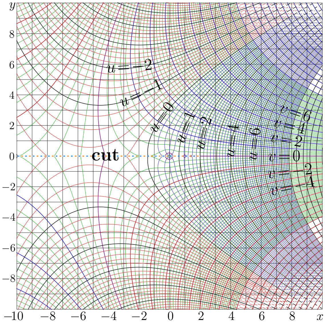
Fig. 9.9: u+iv = T^{1/2}(x+iy) by formula (9.24). [iterEq2map]
