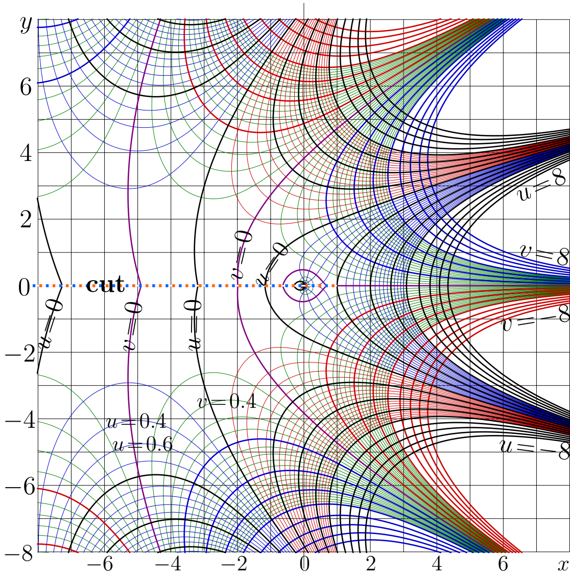
Fig. 8.10: u+iv = \text{Factorial}^{0.5}(x+iy) [QFacMap]
