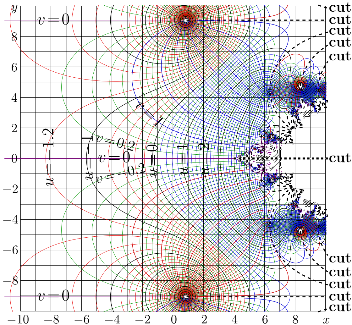
Fig. 16.7: u+iv = \exp_{\sqrt{2},d}^{1/2}(x+iy) [sqrt2q2map]
