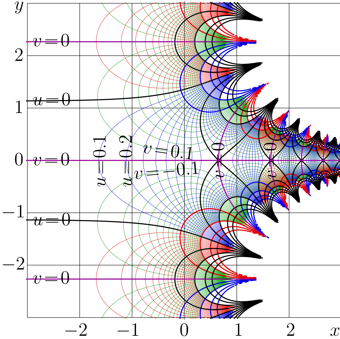
Fig. 7.5: u+iv = \text{Pav}_4(x+iy) by (7.8) [logi2c4]
