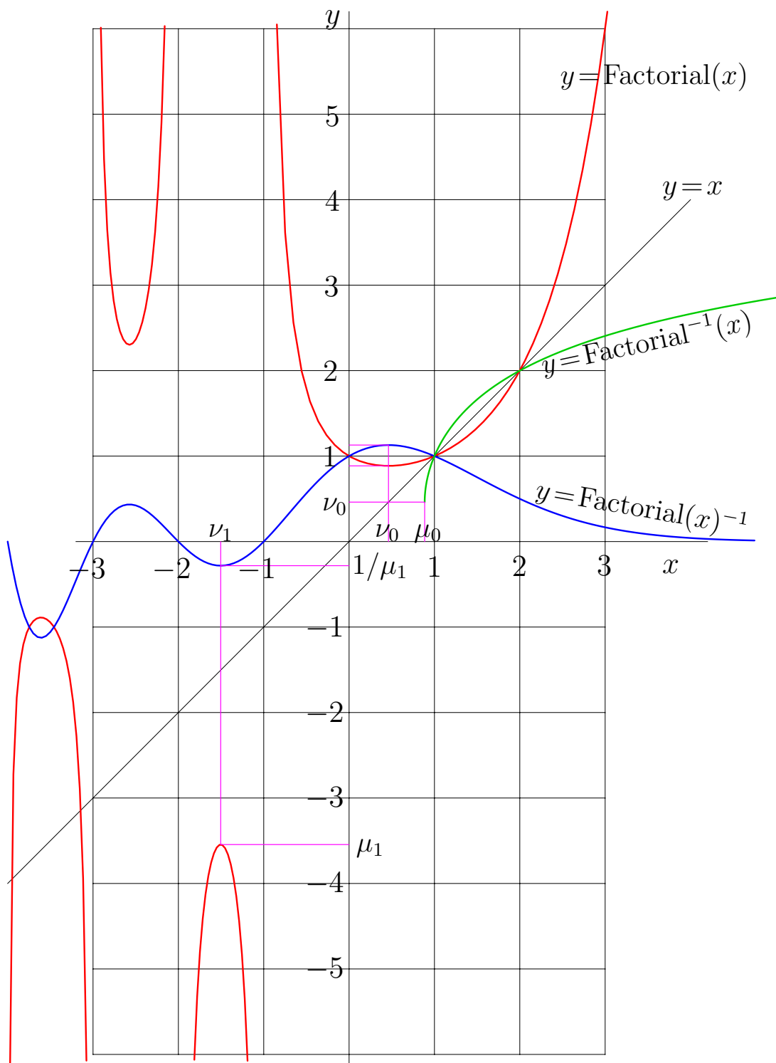
Fig. 8.2: Factorial and related functions for real argument [figfac]
