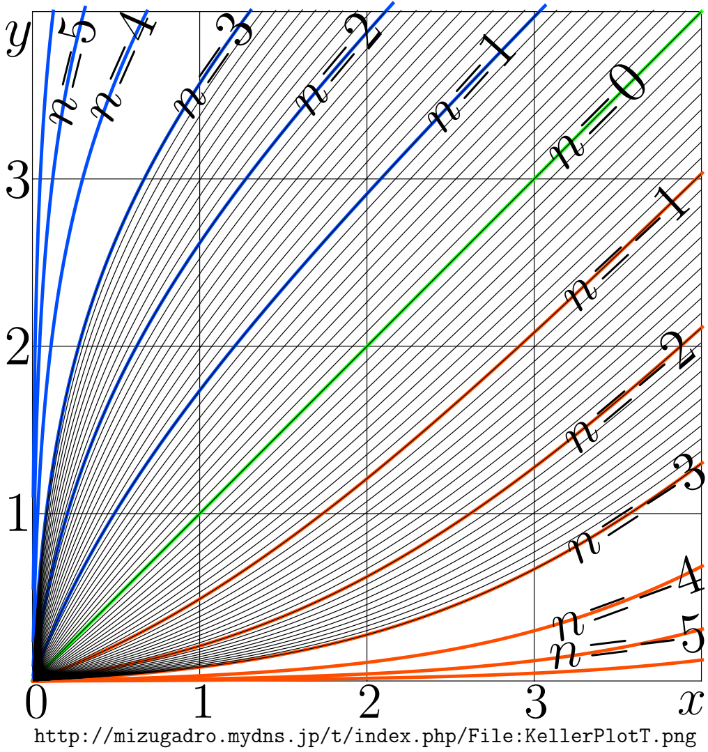
Fig. 5.11: y = \text{Keller}^n(x) . [kellerite]
