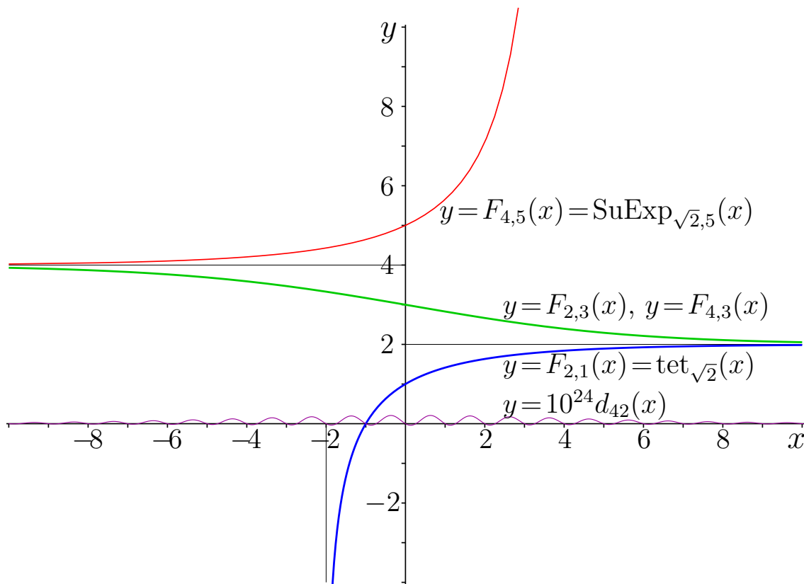
Fig. 16.9: Four superexponents to base \sqrt{2} [sqrt2sufuplot]
