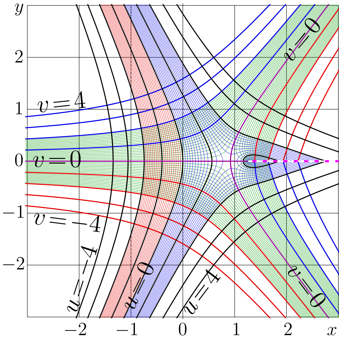
Fig. 7.12: u+iv = \text{Elu}_5^{0.5}(x+iy) [logi2b5]
