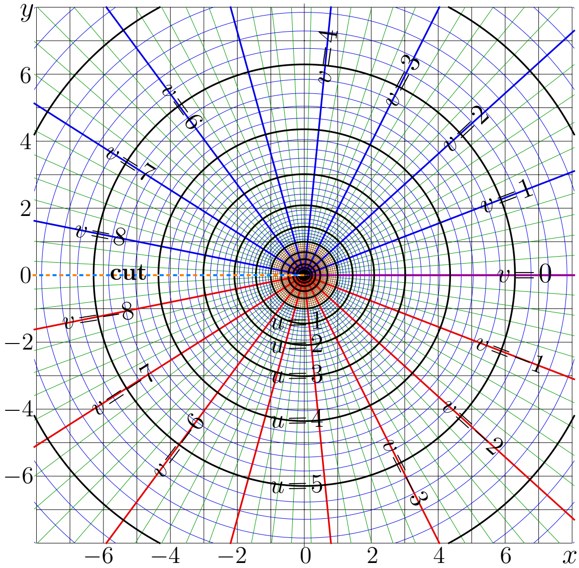
Fig. 10.4: u+iv=\log_{\eta}(x+iy) [loge1emap]
