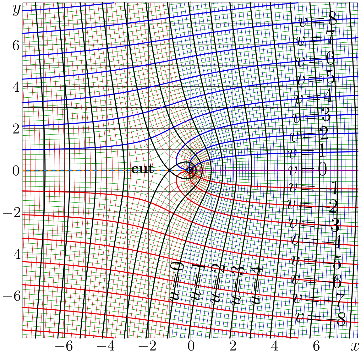
Fig. 5.3: u+iv = \text{ArcTania}(x+iy) [ArcTaniaMap]
