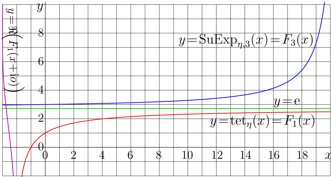
Fig. 10.5: Two super-exponentials to base b = \exp(1/e) [e1eplot]
