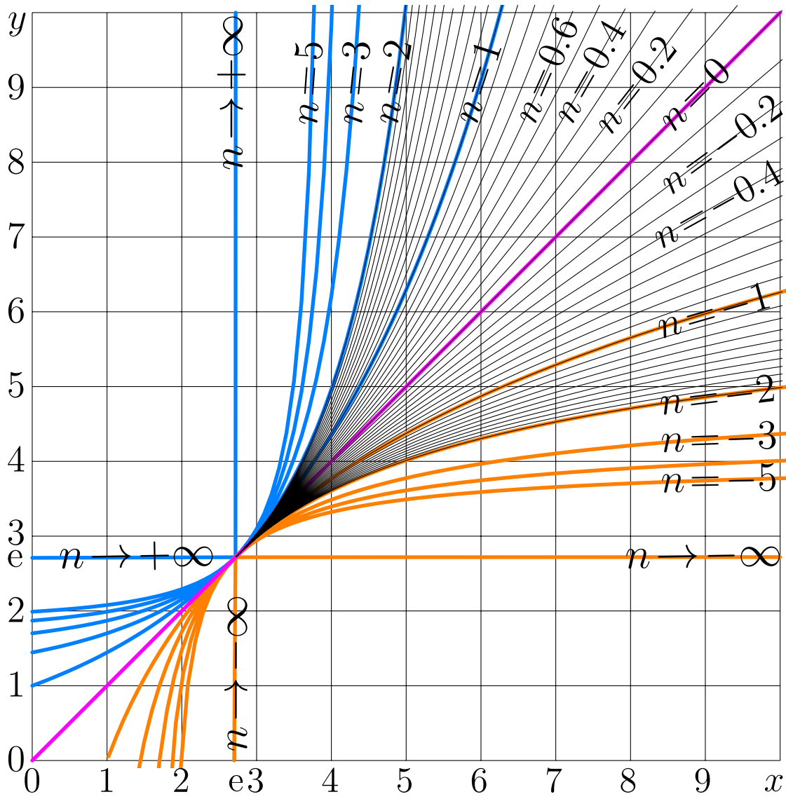
Fig. 10.8: y = \exp_{\eta,u}^n(x) by (10.53) versus x for various n [eleiter]
