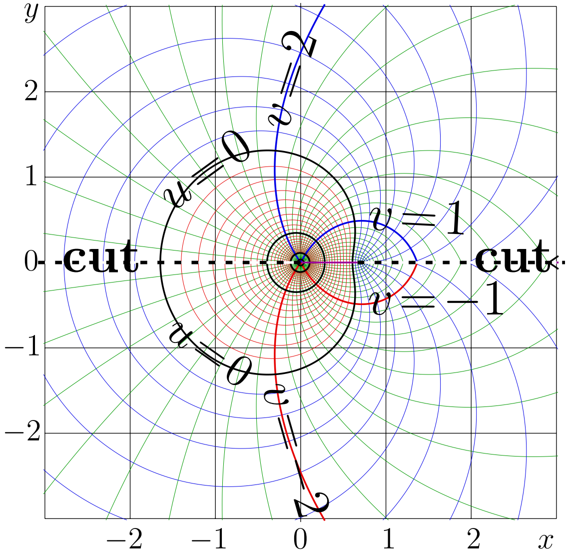
Fig. 7.7: u+iv = \text{ArcPav}_3(x+iy) [logi2d3]
