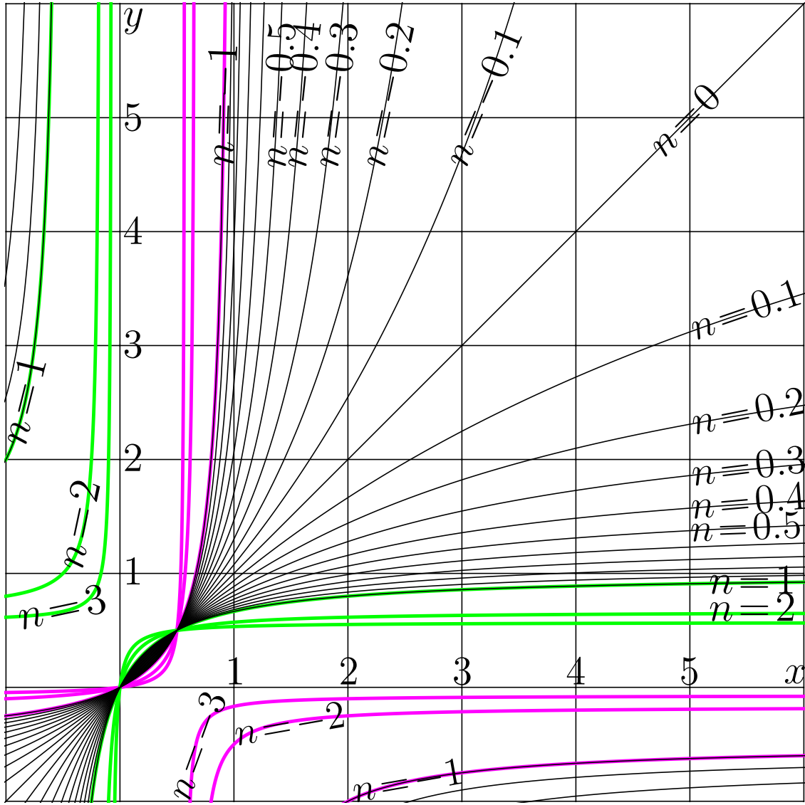
Fig. 4.6: y = t^n(x) by (4.13) at c = 0.5 [c05]
