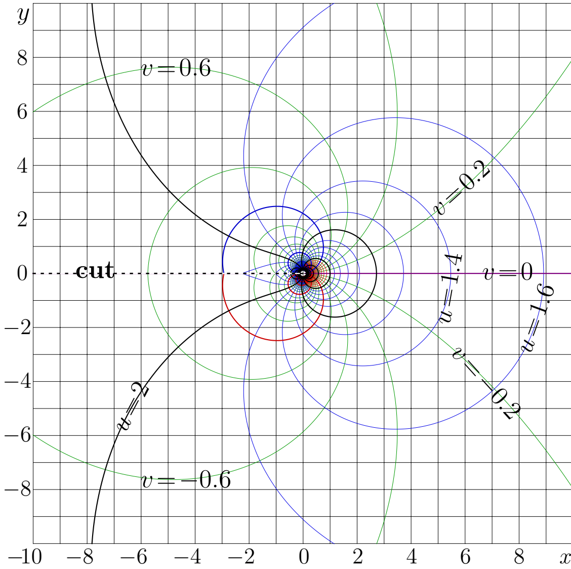
Fig. 11.7: u+iv = \text{AuZex}(x+iy) [auzexmap]
