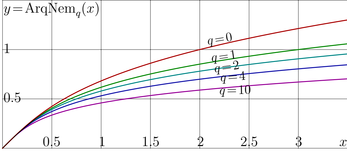
Fig. 13.3: y = \text{ArqNem}_q(x) for q = 0, 1, 2 [arqnemplot]
