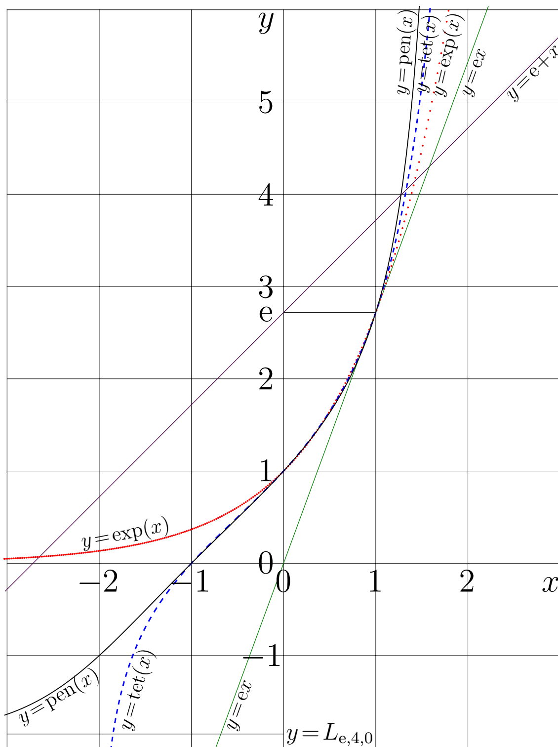
Fig. 19.7: y = A_{e,n}(x) for n = 1, 2, 3, 4, 5 [ackerplo]
