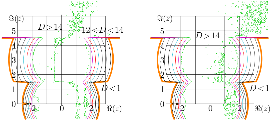
Fig. 14.11: Agreement D = D_8 by (14.59), left; the similar agreement for the contour integral with base domain shifted for -0.5 . [vladi08]
