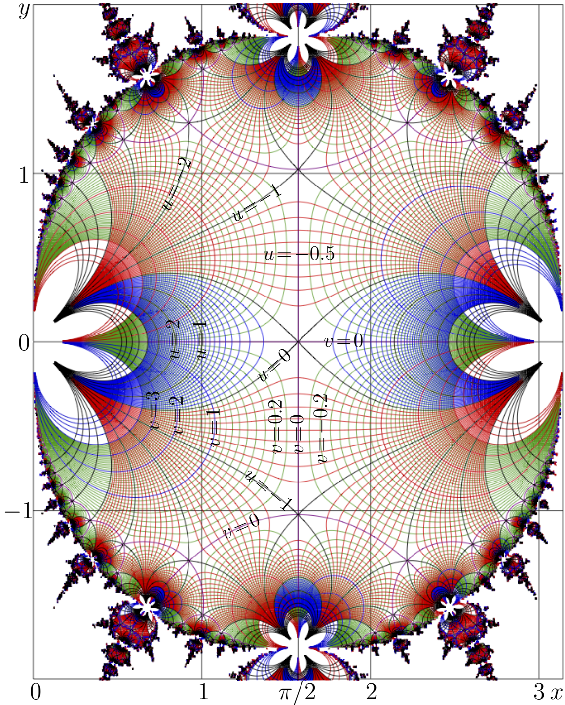
Fig. 12.4: u+iv = \text{AuSin}(x+iy) by formula (12.20) [ausinmap]
