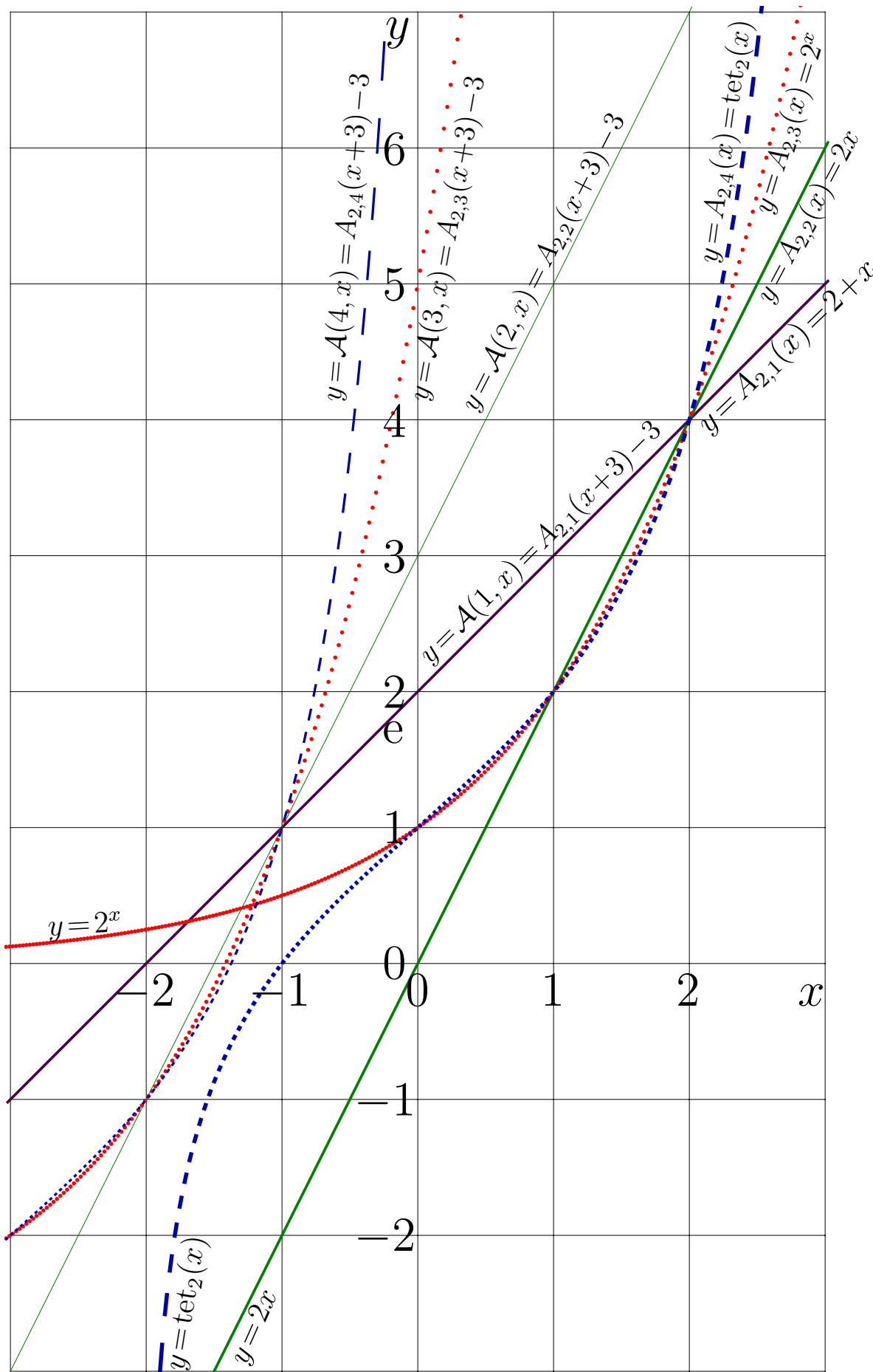
Fig. 19.2: Comparison of definitions for binary ackermanns [acker2t]
