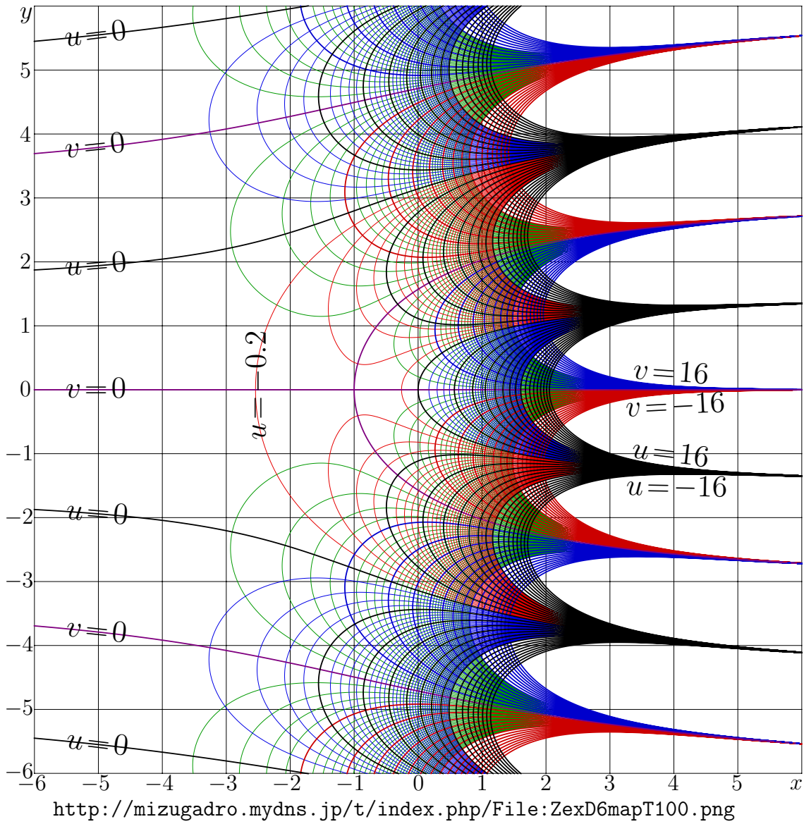
Fig. 11.3: u+iv=\text{zex}(x+iy) by (11.1) [zexmap]
