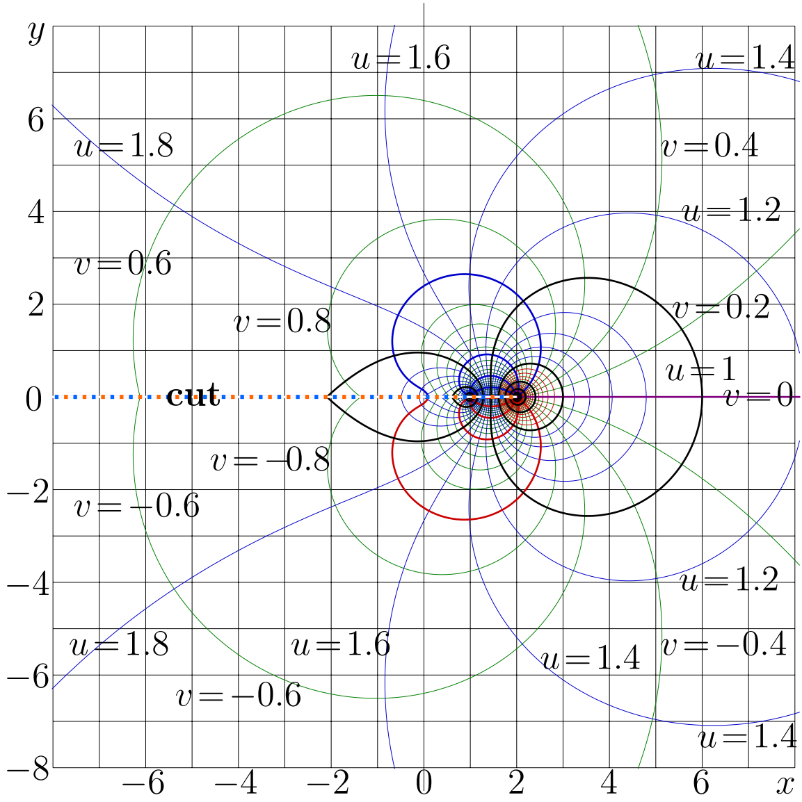
Fig. 8.7: u+iv = \text{AbelFactorial}(x+iy) . [AbelFactorialMap]
