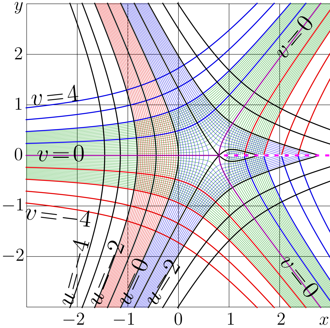
Fig. 7.11: u + iv = \text{Elu}_4^{0.5}(x + iy) [logi2b4]
