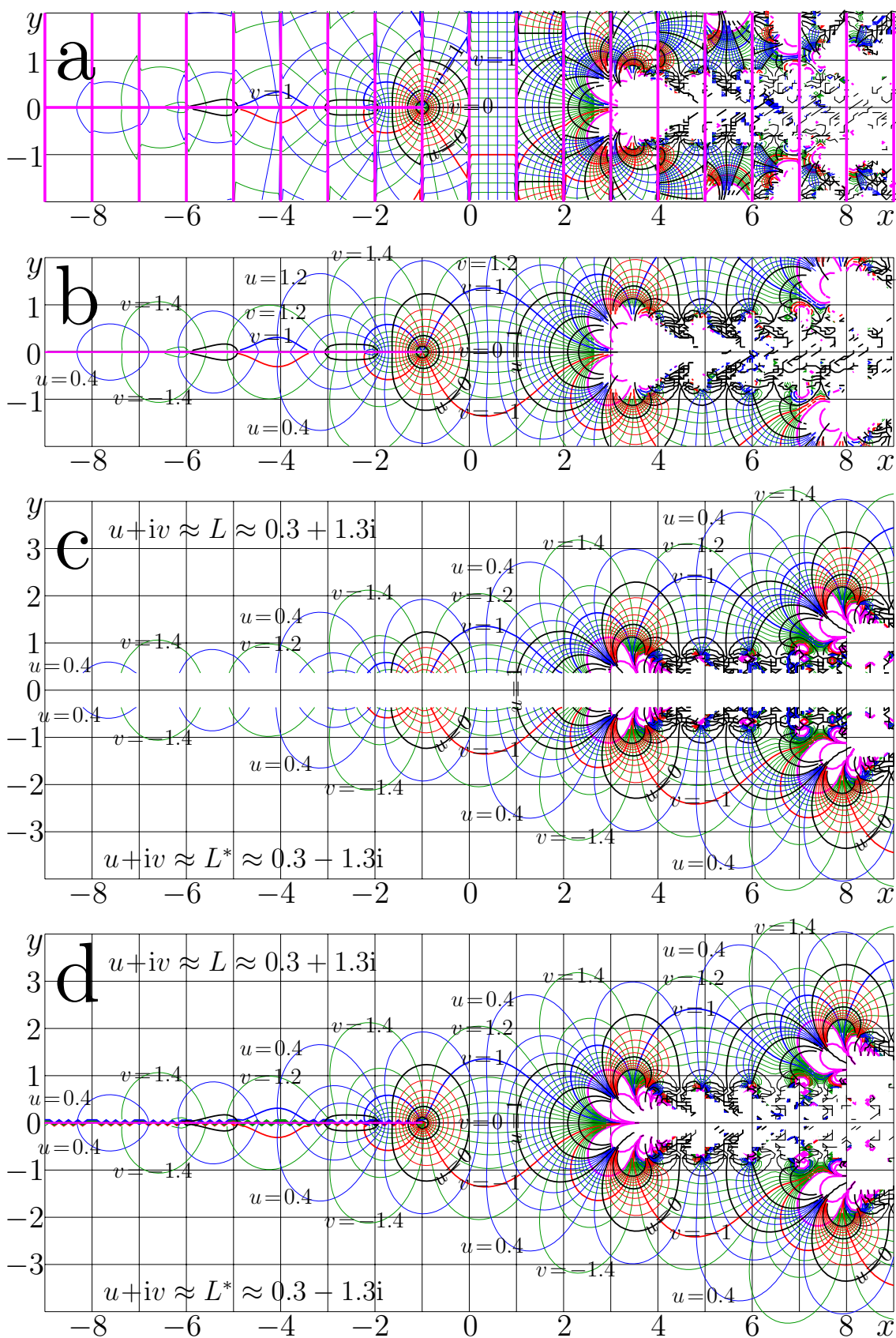
Fig. 14.4: \exp(u+iv) = f(x+iy) for the following functions: f = \text{uxp} , (a); f = \text{Fit}_3 , (b); f = \text{Fit}_6 , (c); f = \text{tet} , (d) [analuxpmap]
