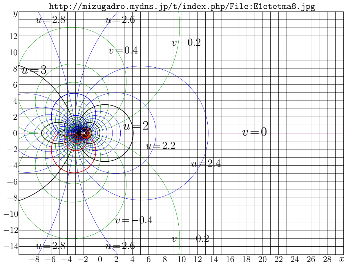
Fig. 10.6: u+iv = \text{SuExp}_{\eta,3}(x+iy) = F_3(x+iy) by (10.45), at the top, and u+iv = \text{tet}_{\eta}(x+iy) = F_1(x+iy) by (10.44), at the bottom. [e1efig2]
