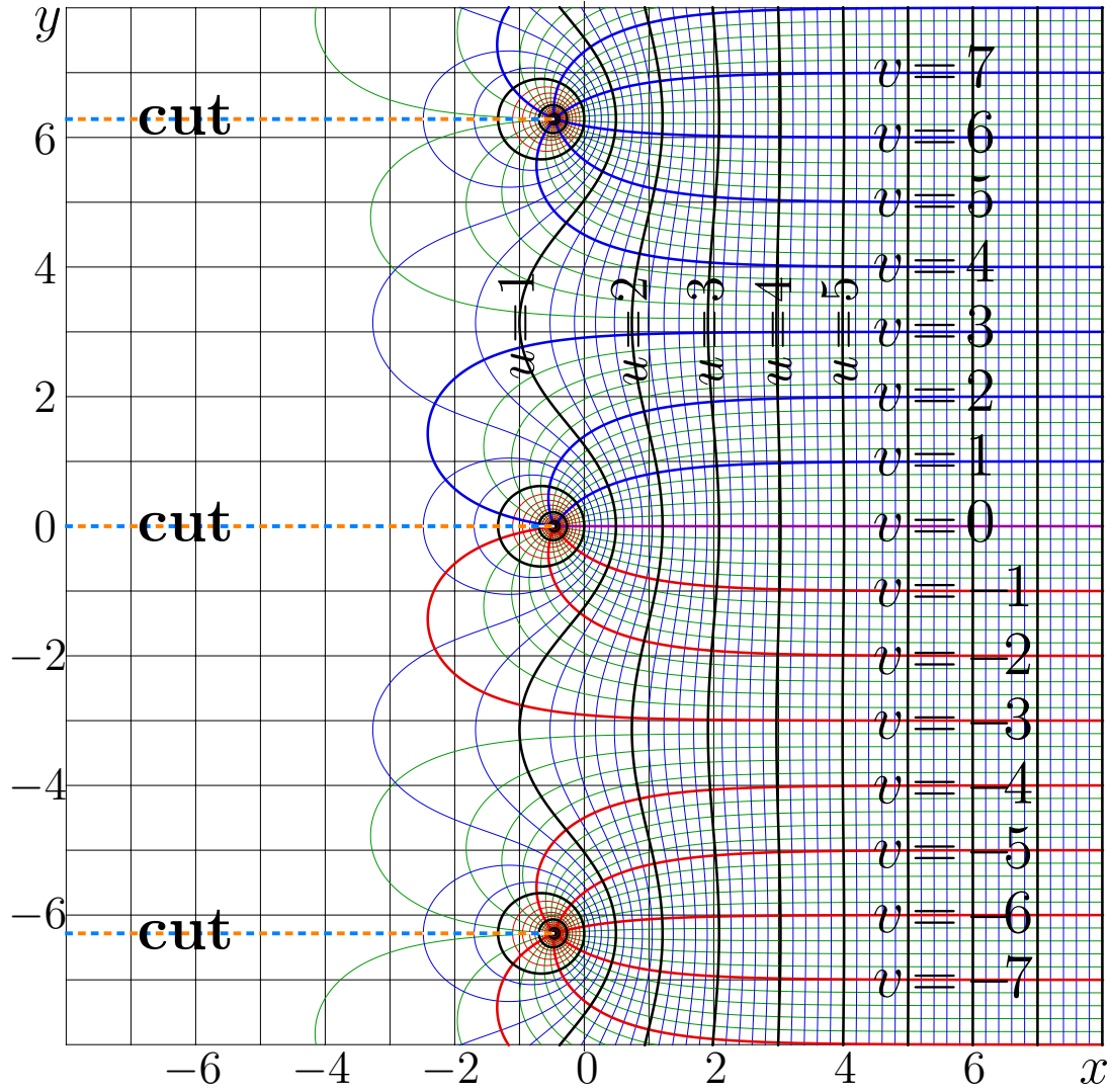
Fig. 5.7: u+v = \text{Keller}(x+iy) by (5.14). [KellerMap]
