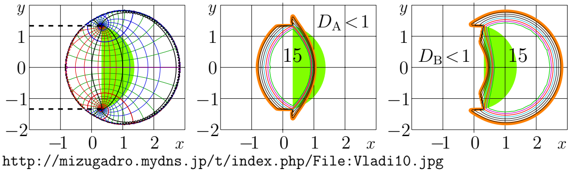
Fig. 15.2: u+iv=\text{slo}(x+iy) by (15.5), left, and the agreements by D_A=D_A(x+iy) , D_B=D_B(x+iy) , by formulas (15.7), (15.8)
