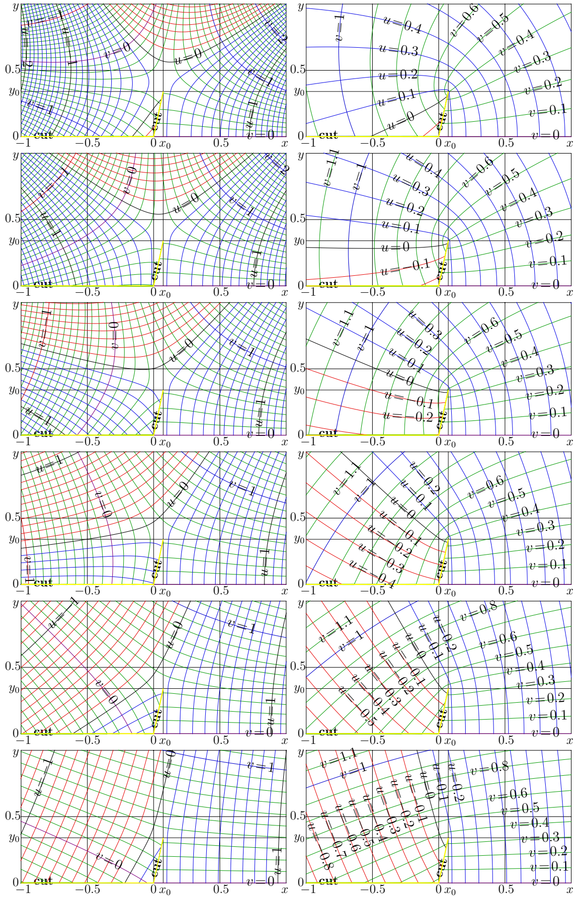
Fig. 13.9: u+iv = \text{Nem}_1^n(x+iy) by (13.24) for n = 0.6 \dots 0.1 , left, and for n = -0.6 \dots -0.1 , right [iteramap]
