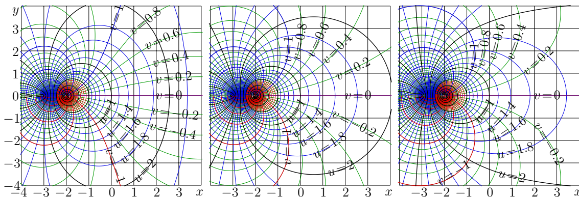
Fig. 17.4: u+iv = \text{tet}_b(x+iy) for b=1.5 , b=\exp(1/e) and b=\sqrt{2} [e1e09]
