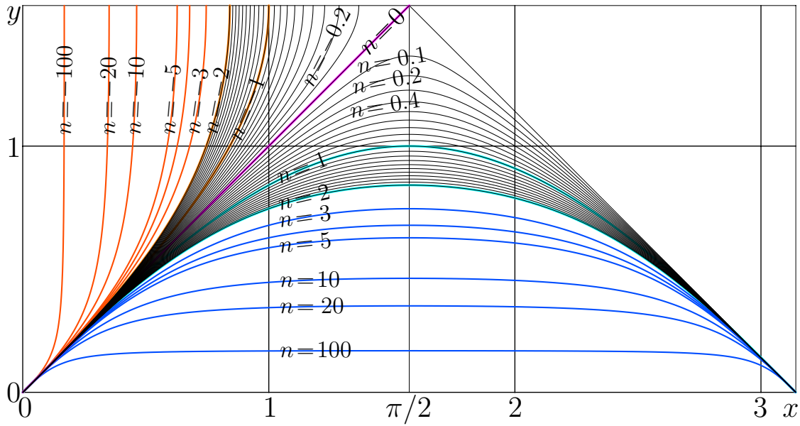
Fig. 12.6: y = \sin^n(x) by (12.25) versus x for various n [sinite]
