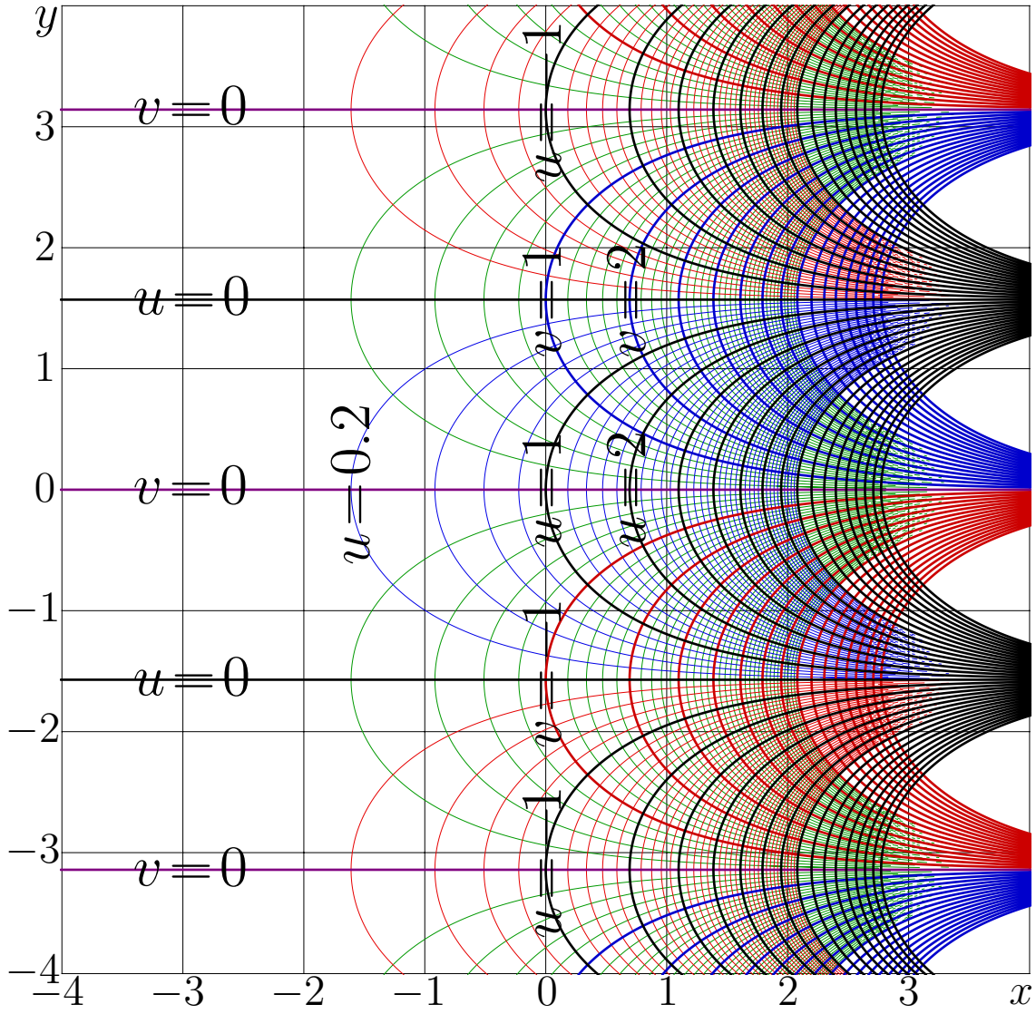
Fig. 14.2: u+iv = \exp(x+iy) [expMap]
