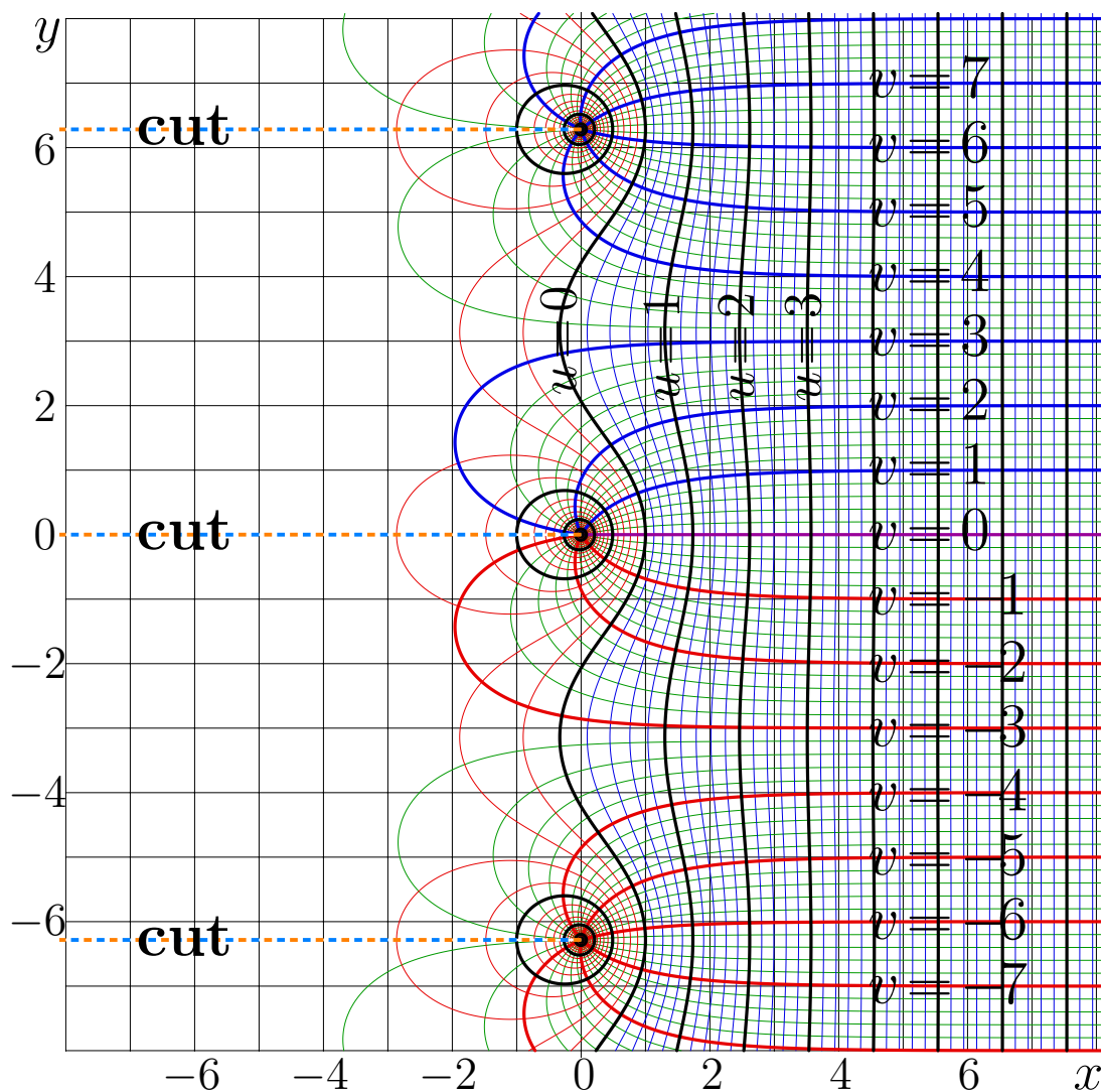
Fig. 5.13: u+iv = \text{ArcShoka}(x+iy) . [ArcShokaMap]
