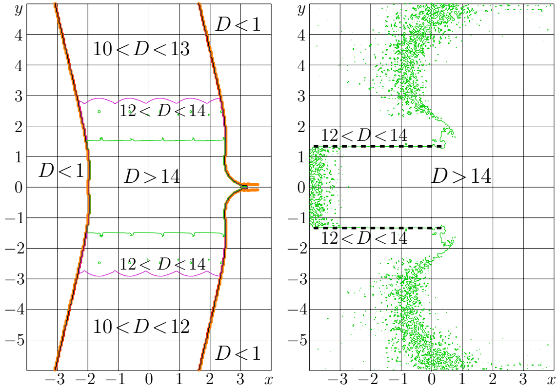
Fig. 15.3: D = D_{\text{at}}(x+iy) , left, and D = D_{\text{ta}}(x+iy) , right, by (15.12) and (15.13) [vladi11]
