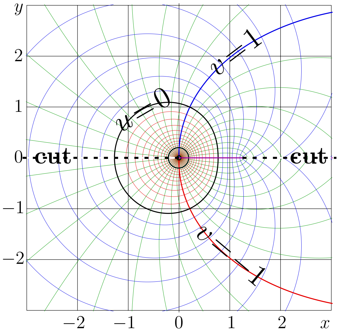
Fig. 7.9: u+iv = \text{ArcPav}_5(x+iy) . [logi2d5]
