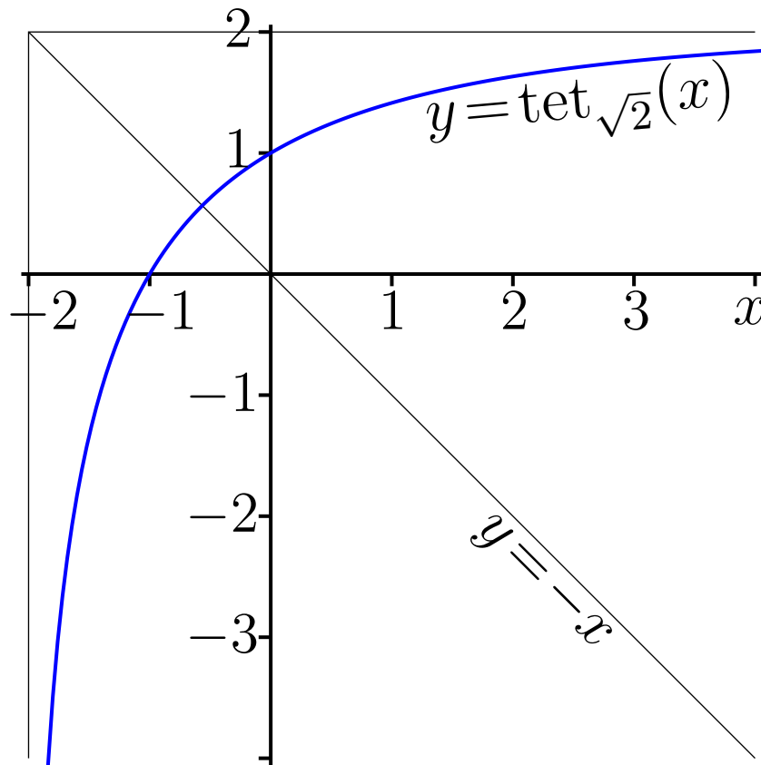
Fig. 16.1: y = \text{tet}_{\sqrt{2}}(x) [sqrt27a]
