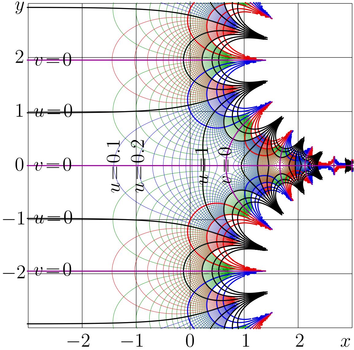
Fig. 7.6: u+iv = \text{Pav}_5(x+iy) by (7.8) [logi2c5]
