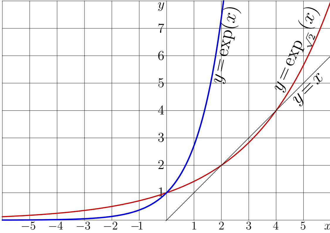
Fig. 14.3: y = \exp(x) and y = \exp_{\sqrt{2}}(x) [ExpQ2ePlot]
