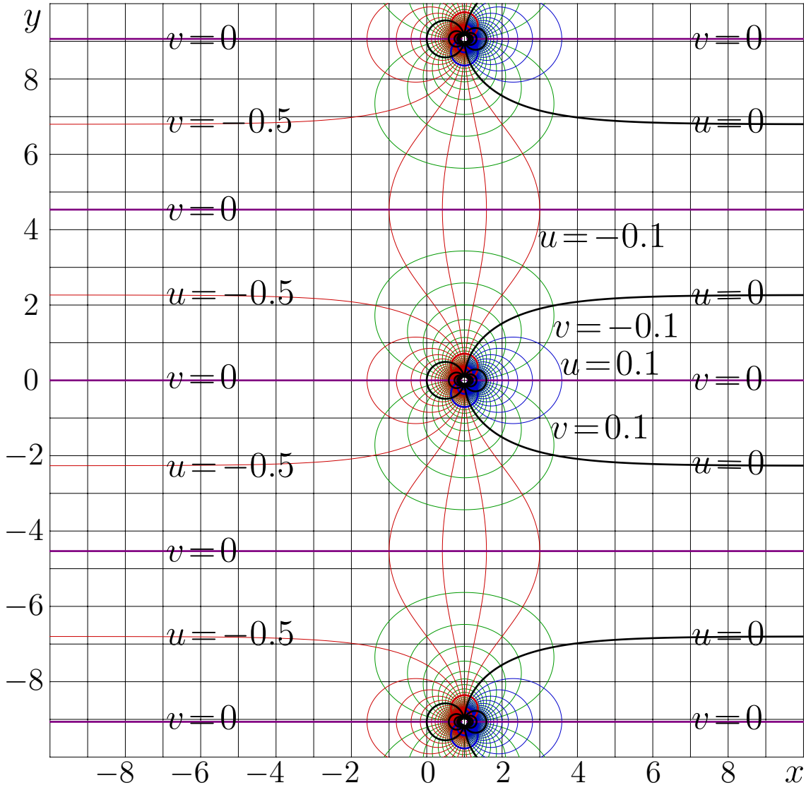
Fig. 4.9: u+iv = f(x+iy) by (4.15) at c=2 [fzfracmap]
