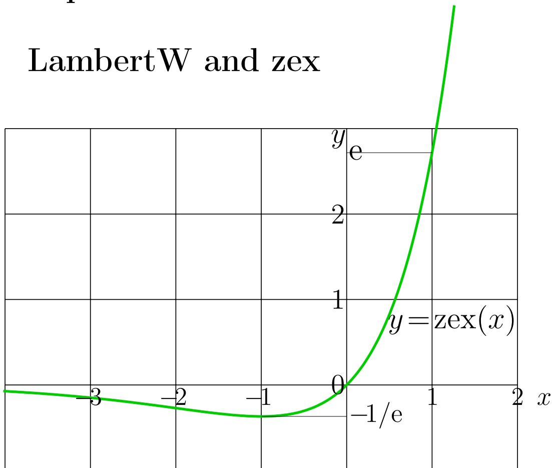
Fig. 11.1: y = \text{zex}(x) = x \exp(x) [zexplot]
