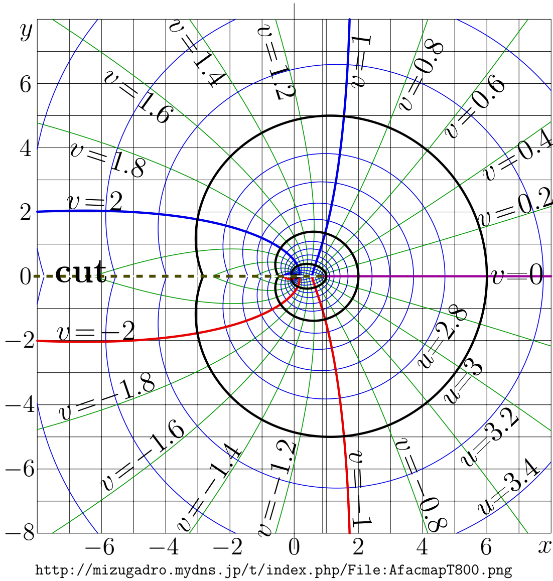
Fig. 8.4: u+iv = \text{ArcFactorial}(x+iy) [arcfacmap]
