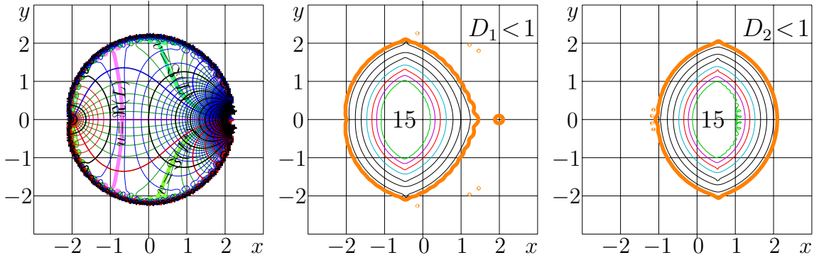
Fig. 14.6: u+iv=\text{naiv}(x+iy) by (14.32) for N=50 , left; agreements D_1=D_{\text{naiv1}}(x+iy) and D_2=D_{\text{naiv2}}(x+iy) by (14.34) and (14.35), central and right hand side maps. [vladi04]
