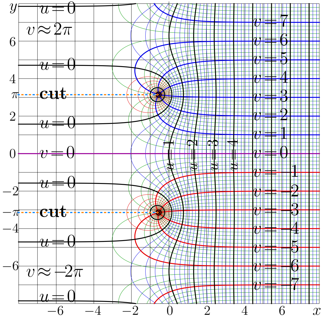
Fig. 5.12: u+iv = \text{Shoka}(x+iy) [ShokaMap]
