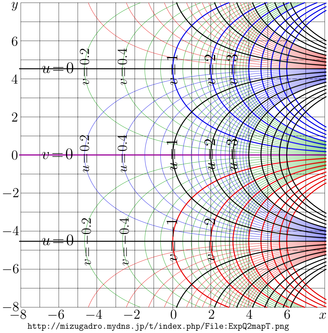
Fig. 9.2: u + iv = \exp_{\sqrt{2}}(x + iy)
