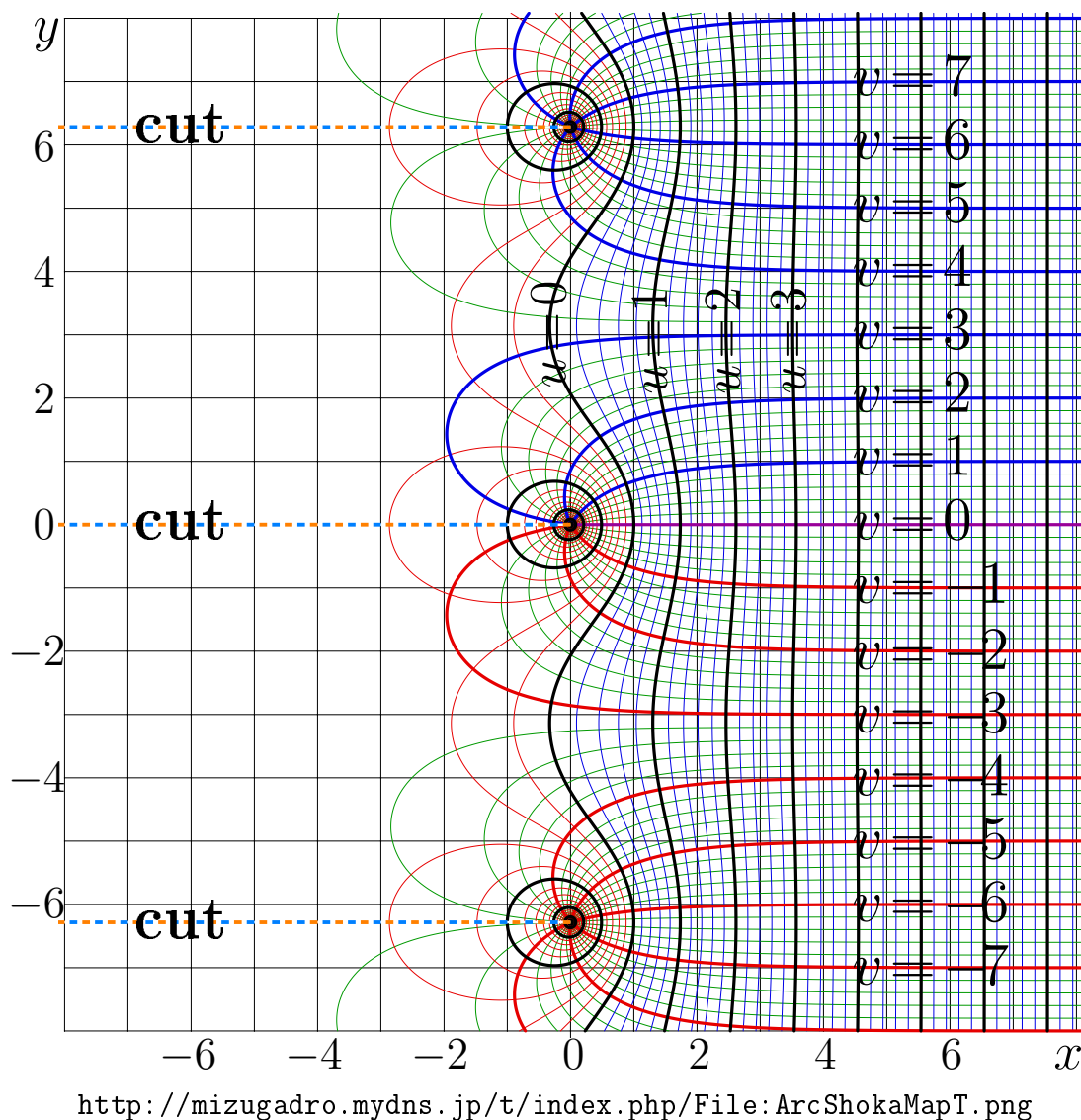
Fig. 5.13: u+iv = \text{ArcShoka}(x+iy) .
