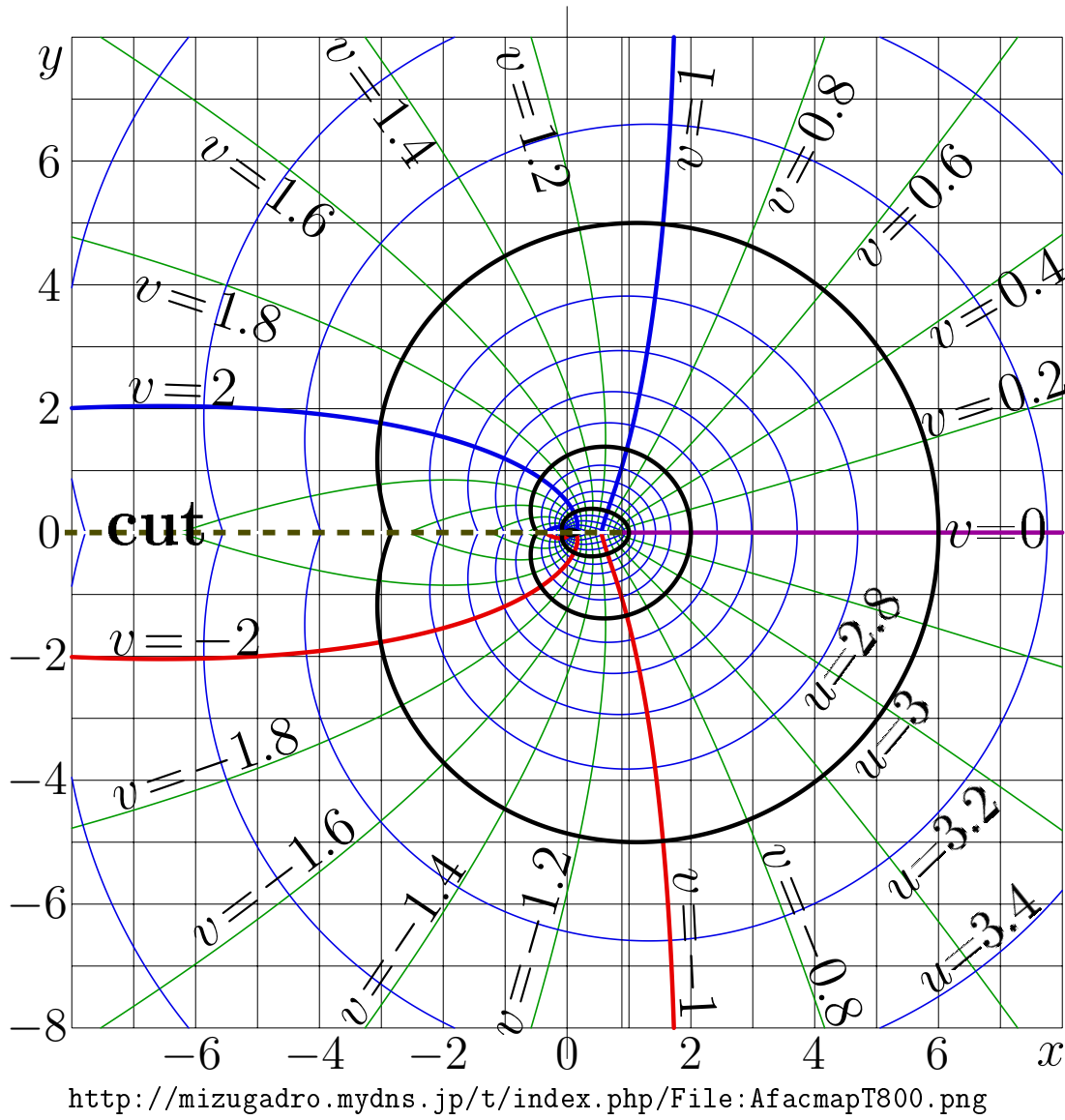
Fig. 8.4: u+iv = \text{ArcFactorial}(x+iy)
