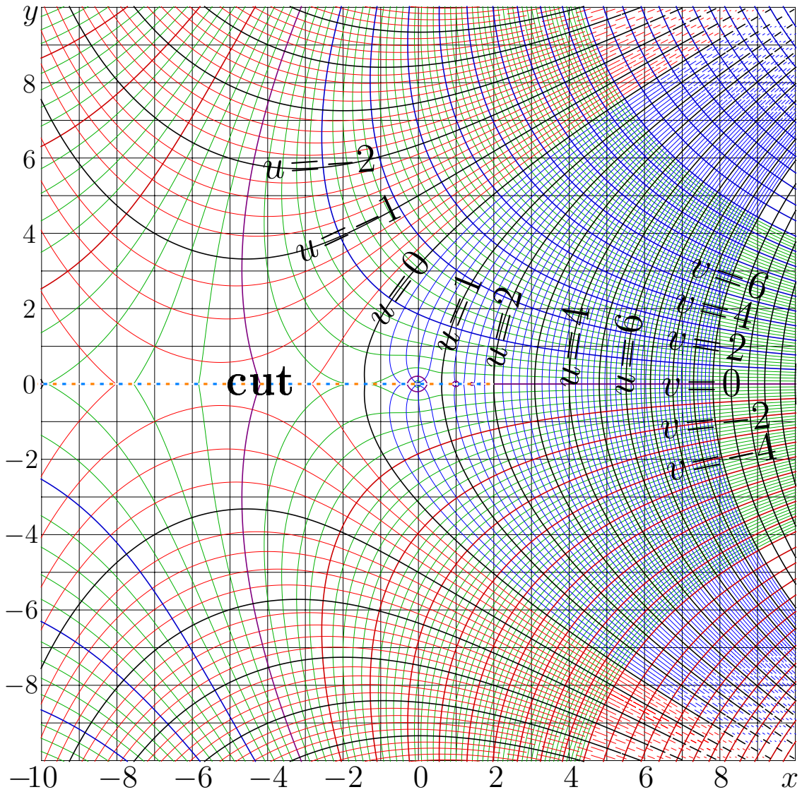
Fig. 9.9: u+iv=T^{1/2}(x+iy) by formula (9.24).
