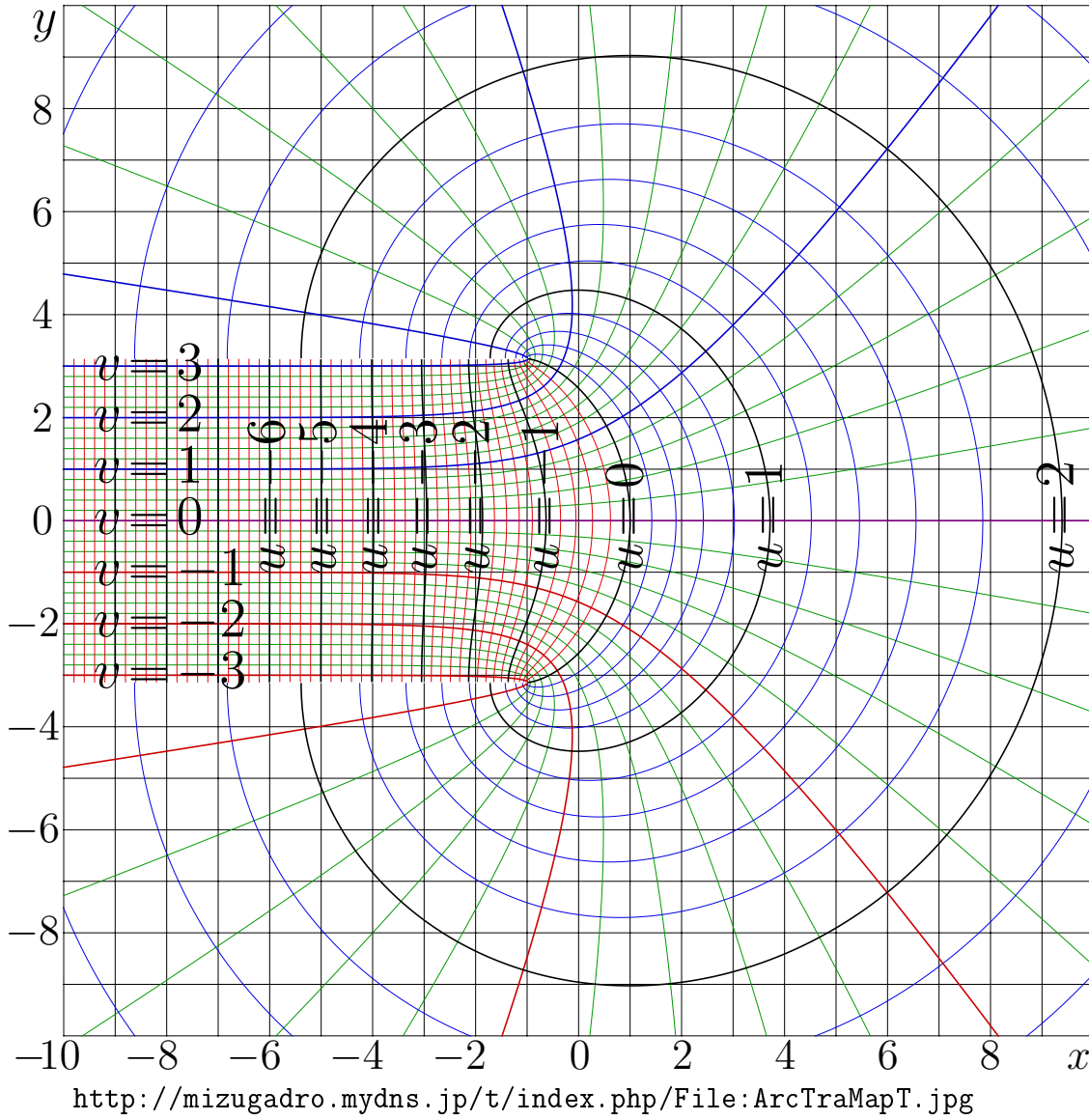
Fig. 20.3: u+iv = \text{ArcTra}(x+iy)
