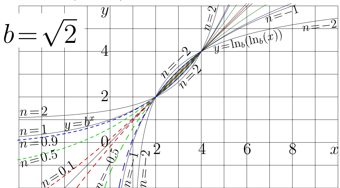
http://mizugadro.mydns.jp/t/index.php/File:E1e14z600.jpg Fig. 17.3: y = \exp_b^n(x) for various n at b=e , b=\exp(1/e) , b=\sqrt{2}
