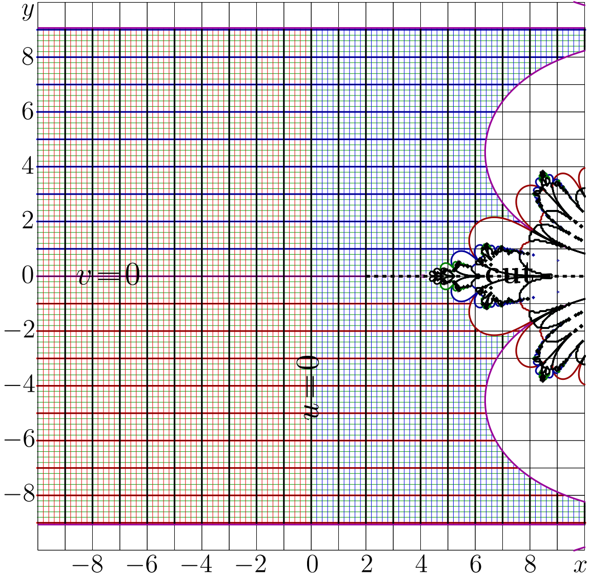
Fig. 16.4: u+iv = \text{tet}_{\sqrt{2}}(\text{ate}_{\sqrt{2}}(x+iy))
