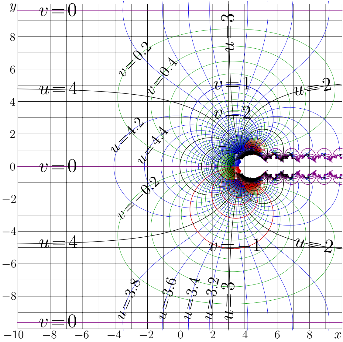
Fig. 9.6: u+iv = \text{SuExp}_{\sqrt{2},5}(x+iy) by (9.13)
