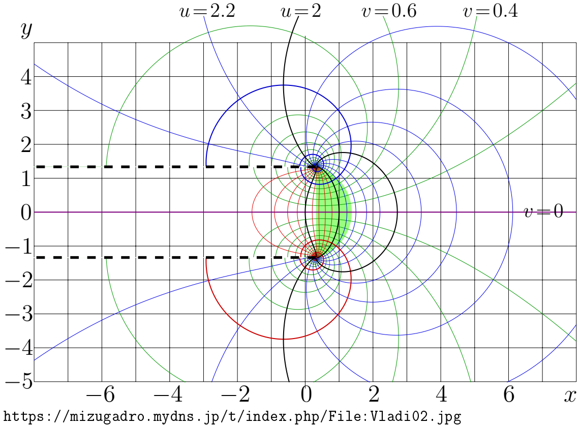
Fig. 15.1: u+iv = \text{ate}(x+iy)
