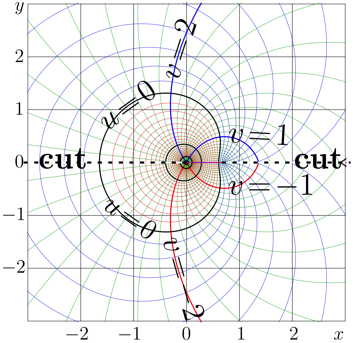
Fig. 7.7: u+iv = \text{ArcPav}_3(x+iy)
