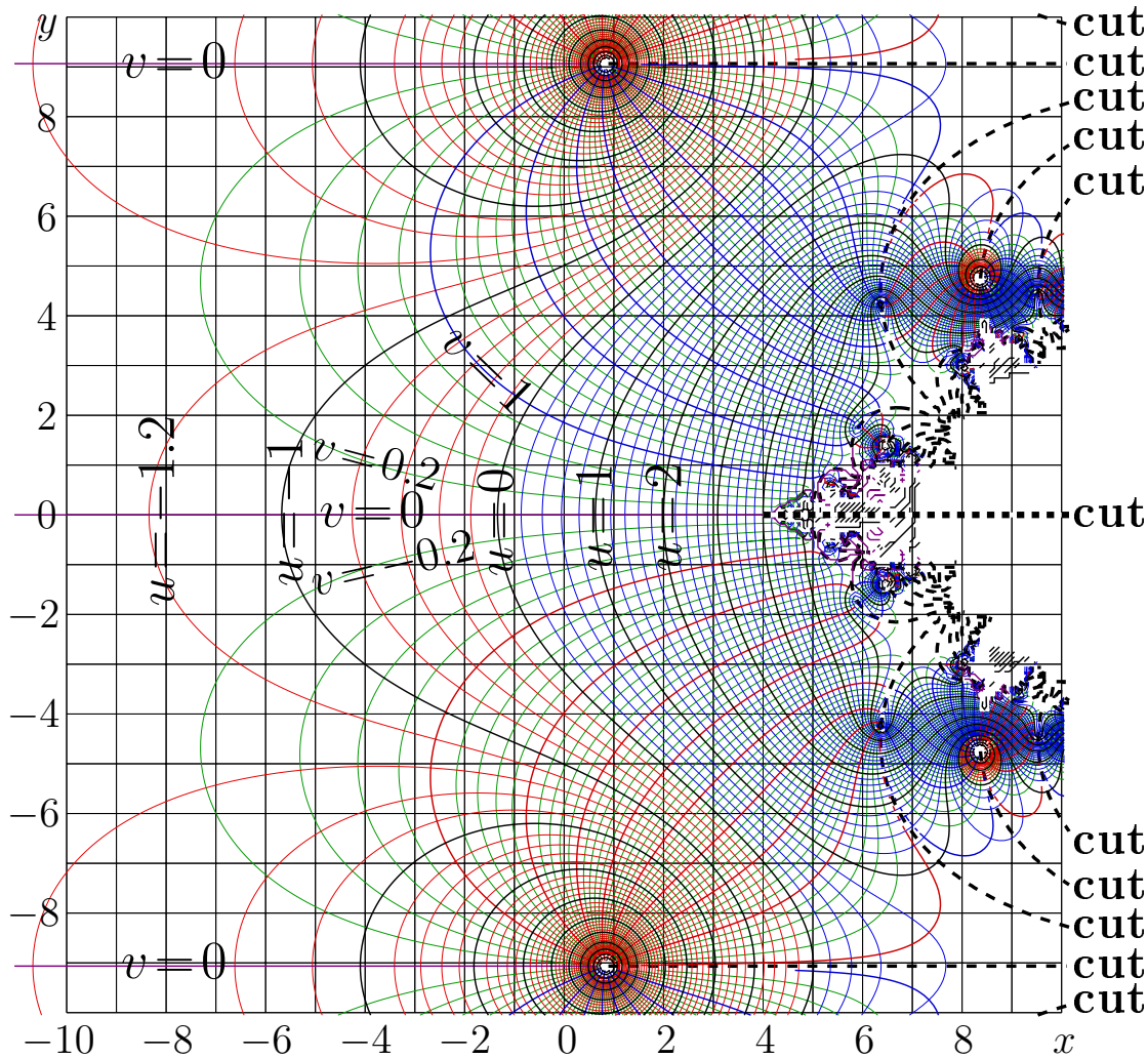
Fig. 16.7: u+iv = \exp_{\sqrt{2},d}^{1/2}(x+iy)
