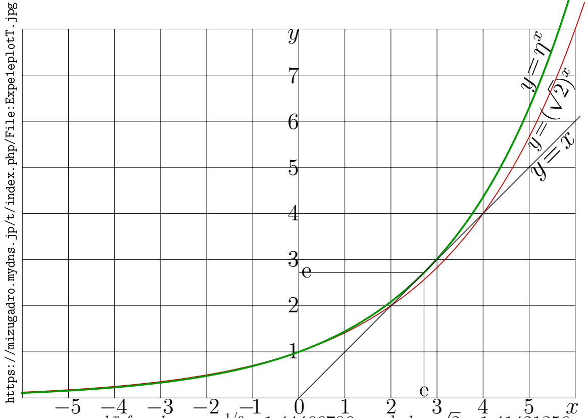
Fig. 10.1: y = b^x for b = \eta = e^{1/e} \approx 1.44466786 and b = \sqrt{2} \approx 1.41421356
