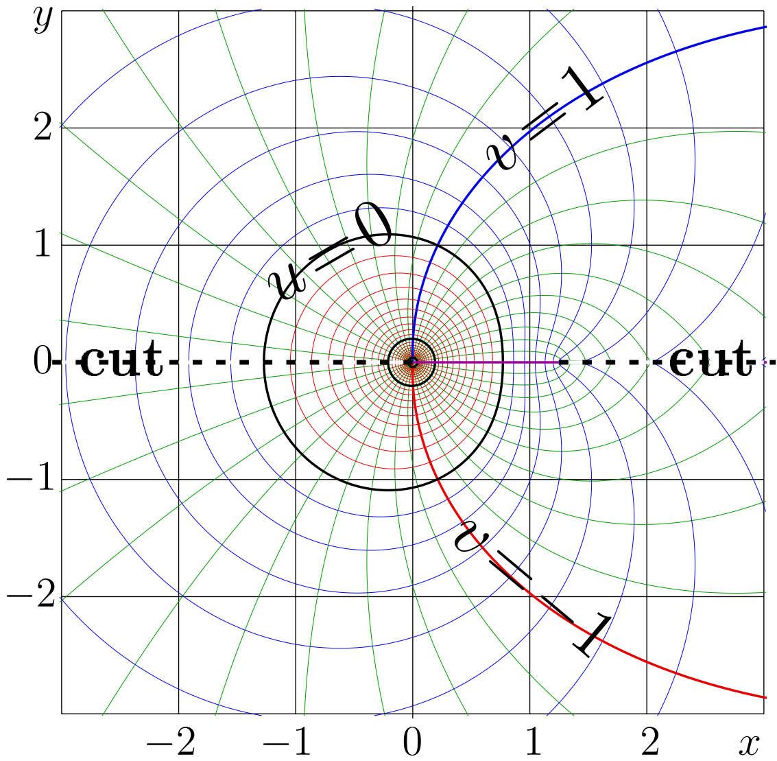
Fig. 7.9: u+iv = \text{ArcPav}_5(x+iy) .
