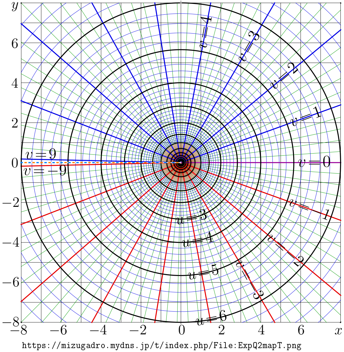
Fig. 9.3: u+iv = \log_{\sqrt{2}}(x+iy)
