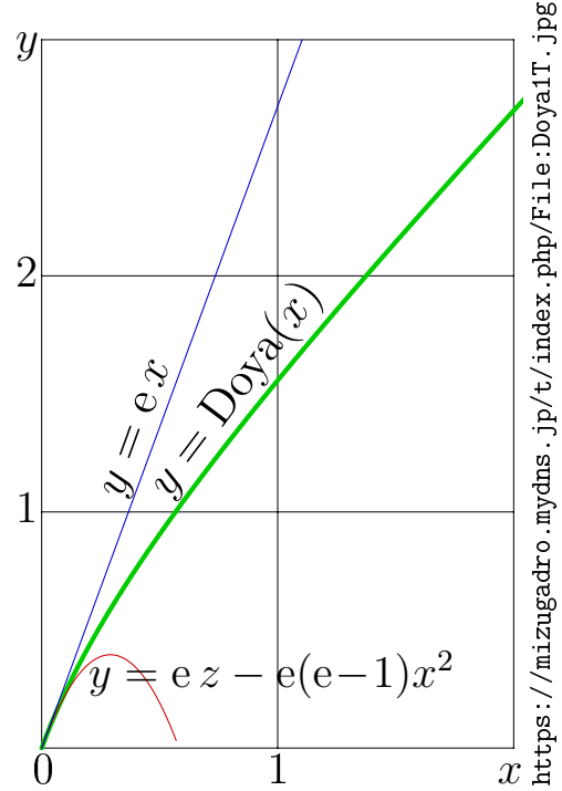
Fig. 6.1: Function Doya and its polynomial approximations
