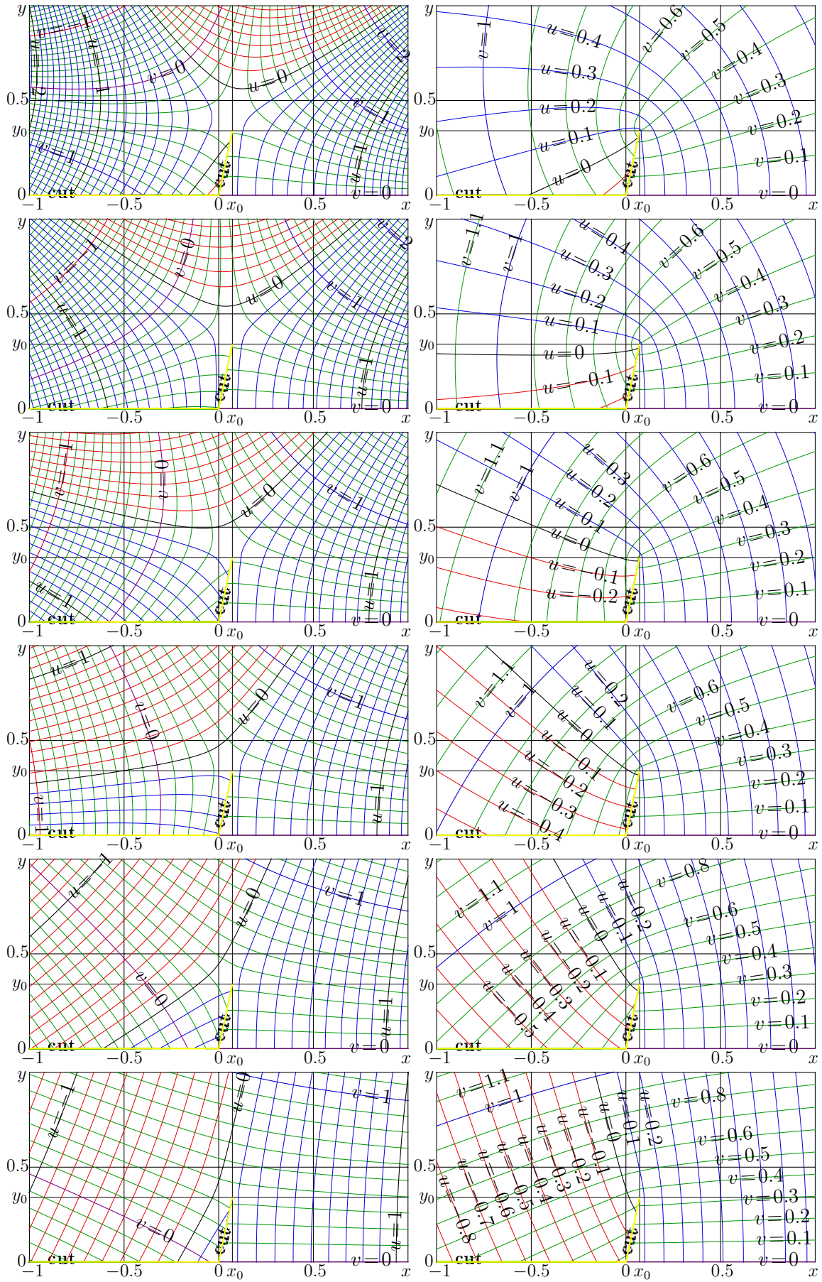
Fig. 13.9: u+iv = \text{Nem}_1^n(x+iy) by (13.24) for n = 0.6 \dots 0.1 , left, and for n = -0.6 \dots -0.1 , right
