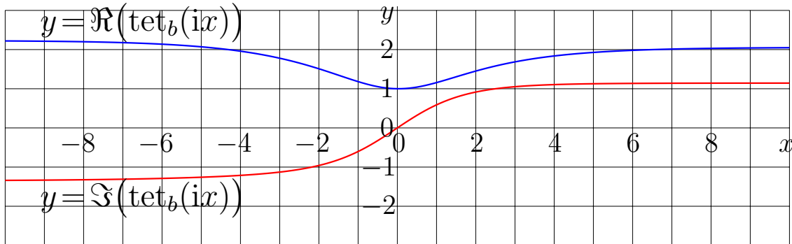
Fig. 18.3: Tetration to base b = 1.52598338517 + 0.0178411853321i : Top map: u+iv = \text{tet}_b(x+iy) ; Intermediate plot: y = \Im(\text{tet}_b(x)) and y = \Re(\text{tet}_b(x)) , thick curves; the thin curve shows y = \text{tet}_{1.5}(x) from figure 17.1 ; Bottom plot: y = \Im(\text{tet}_b(ix)) and y = \Re(\text{tet}_b(ix))
