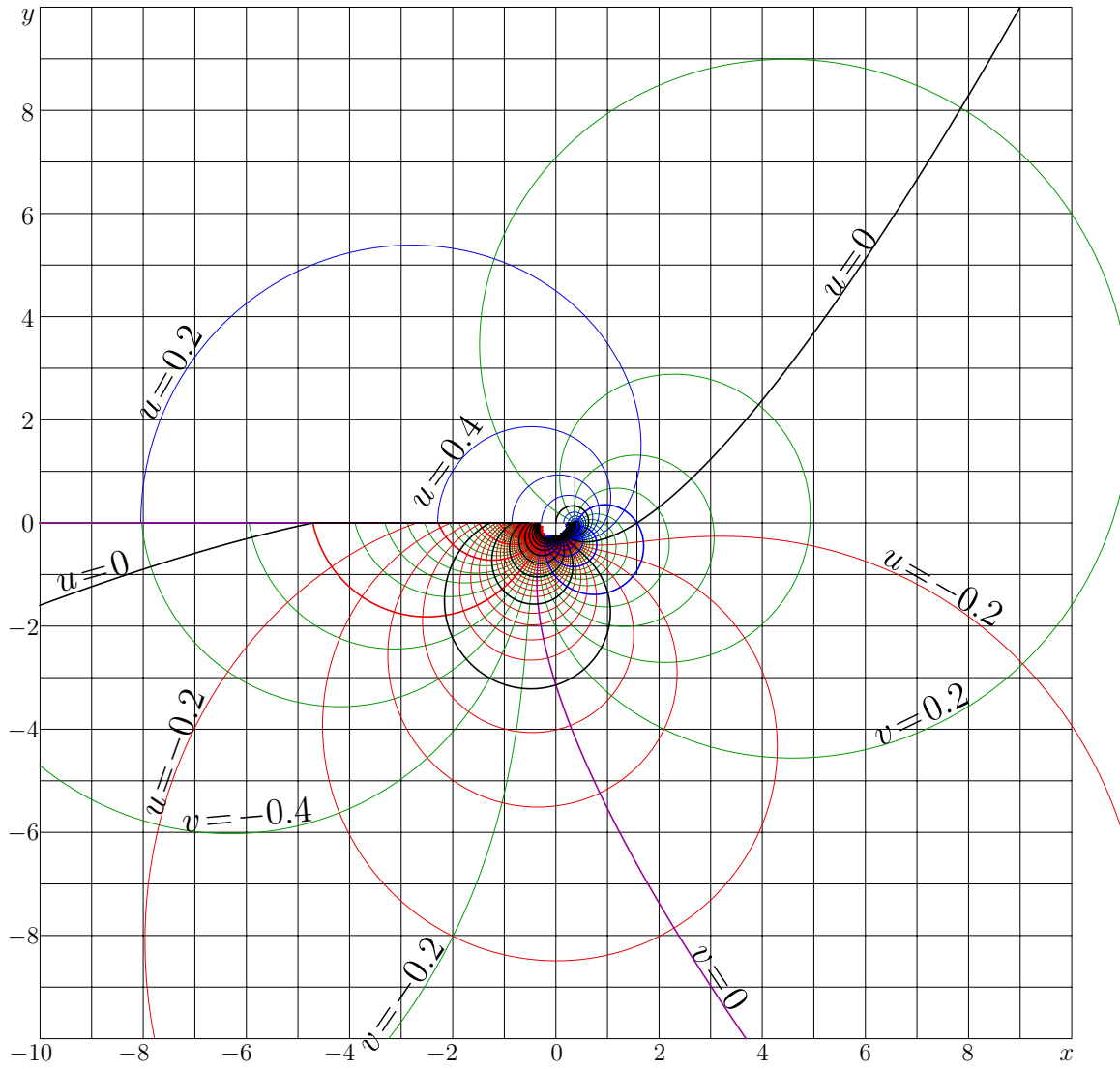
Fig. 18.1: u+iv=\text{filog}(x+iy) , as solution L=\text{filog}(B) of (18.1)
