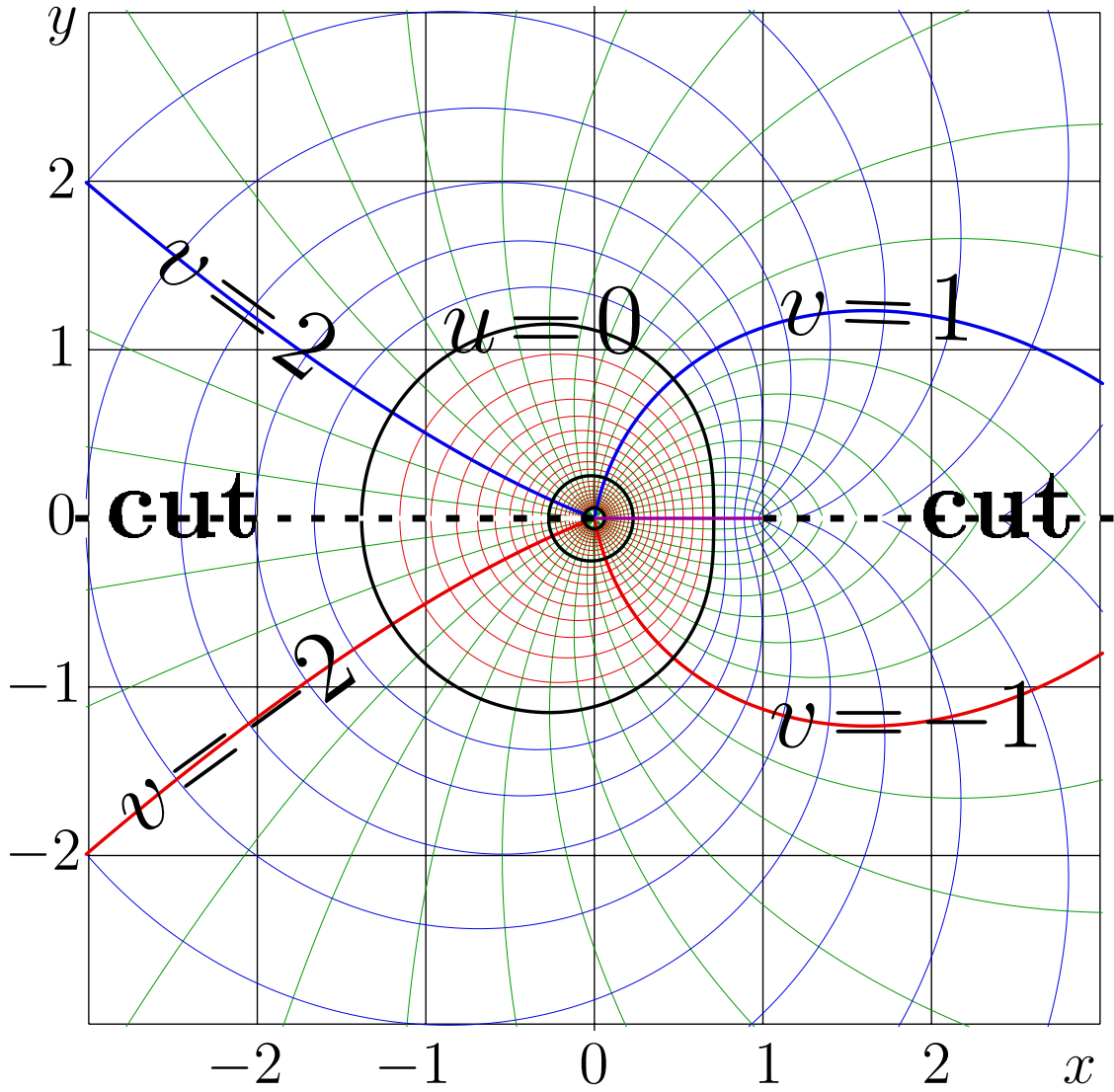
Fig. 7.8: u+iv = \text{ArcPav}_4(x+iy) .
