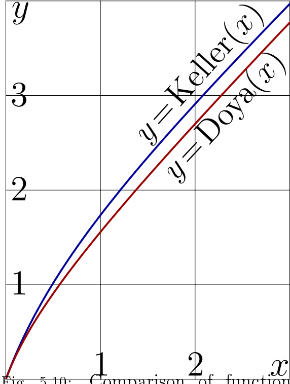
Fig. 5.10: Comparison of functions Keller и Doya by (5.14) and (5.11)
