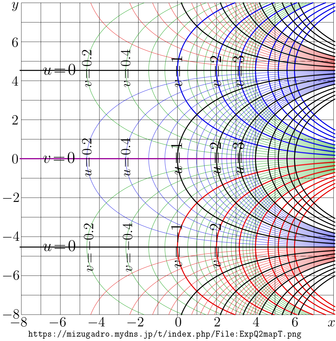
Fig. 9.2: u+iv = \exp_{\sqrt{2}}(x+iy)
