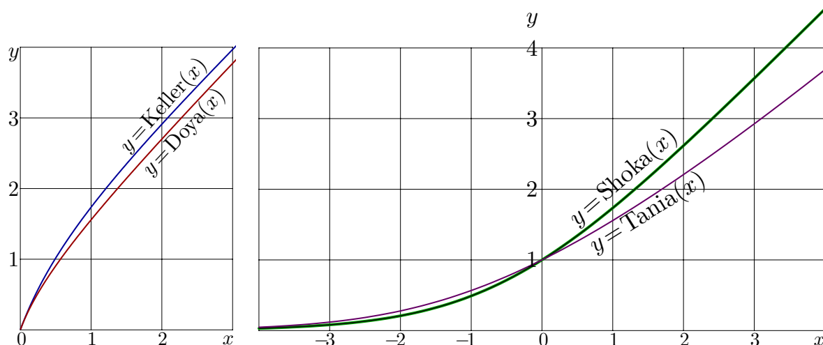
Fig. 2. Function Keller by (6) in comparison with function Doya by (5), left; function Shoka by (8) in comparison with function Tania by (7), right.
