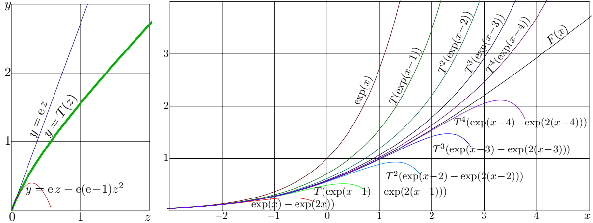
Fig. 1. Left: Transfer function T by (5) and its approximations. Right: superfunction F by (7) and its approximations \tilde{F} by the regular iteration (18) for n=0..4 .
