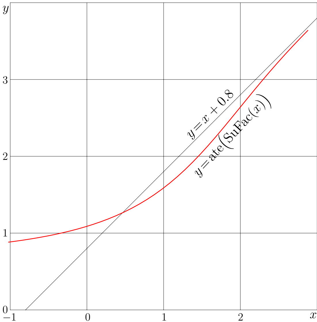
Plot of combination of natural ArcTetration and SuperFactorial:
