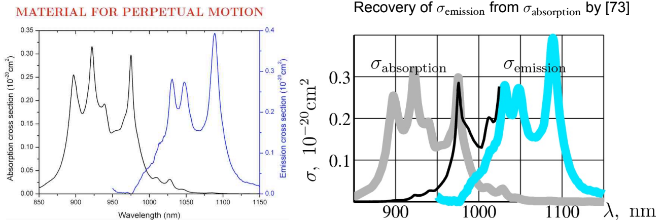
Fig. 6. Fake result [70, 71, 72]; correction of \sigma_{\text{emission}} by the McCumber relation [73] (thin line)
