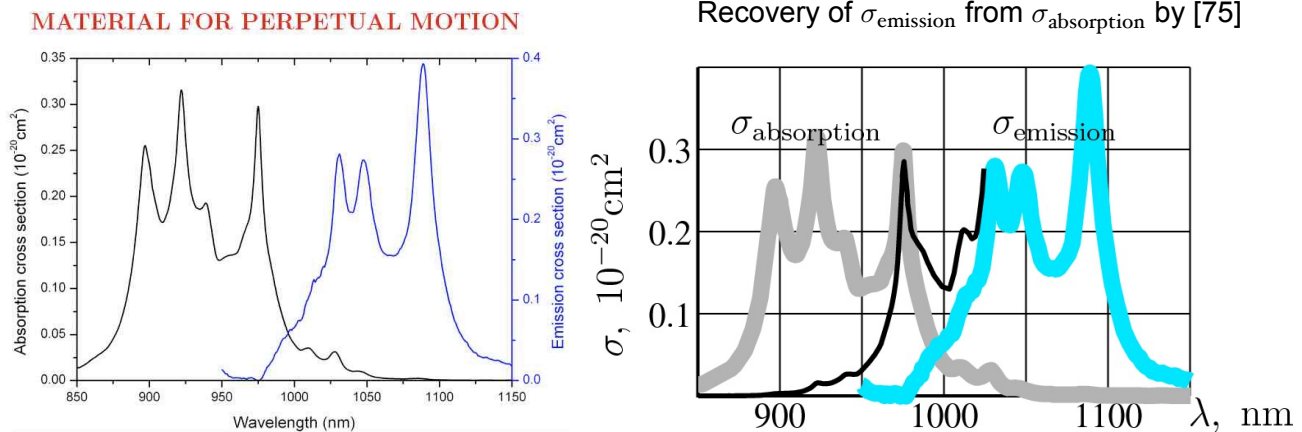
Fig. 6. Fake result [72, 73, 74]; correction of \sigma_{\text{emission}} by the McCumber relation [75] (thin line)
